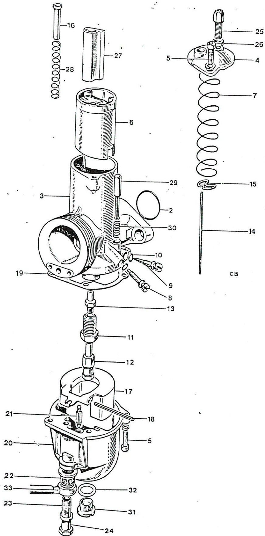
Fig. 6. CARBURETOR, T100R
