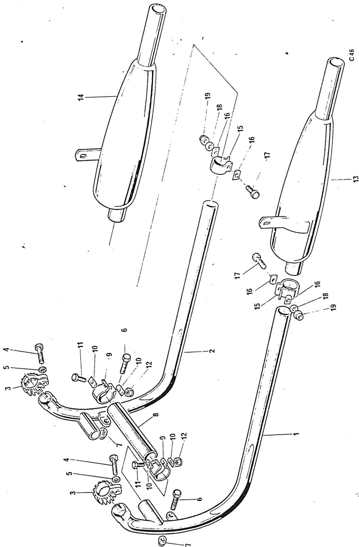
Fig. 15. EXHAUST SYSTEM
