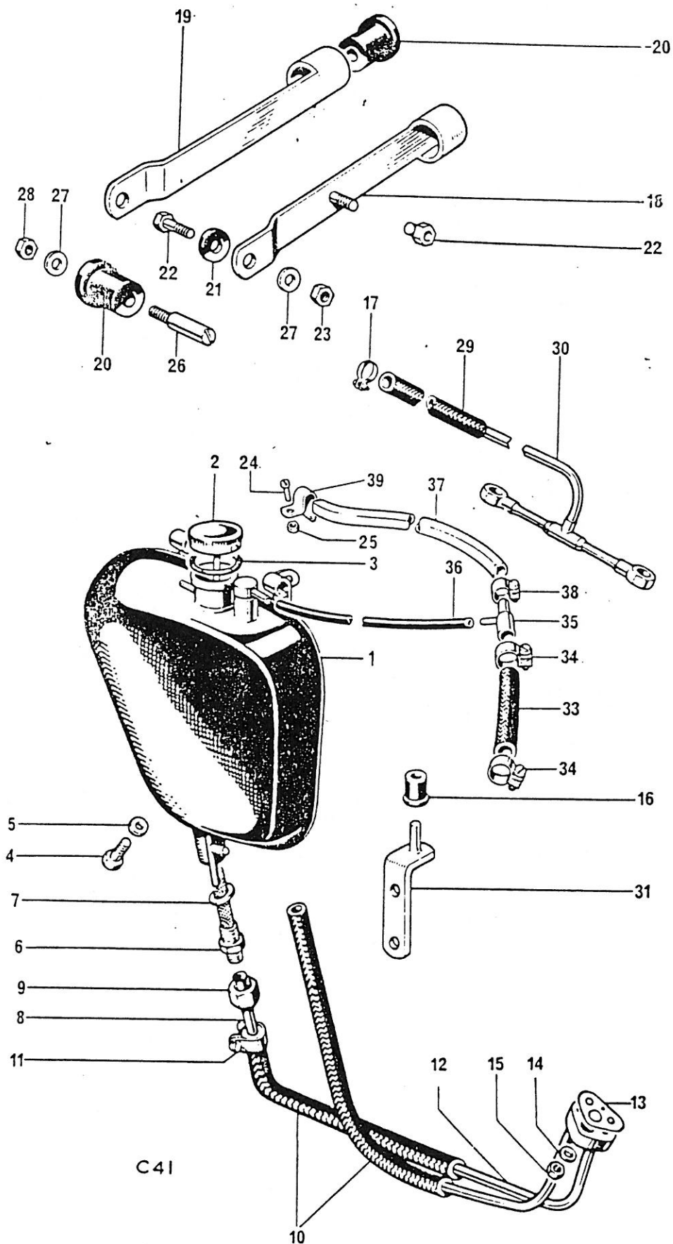
Fig. 28. OIL TANK
