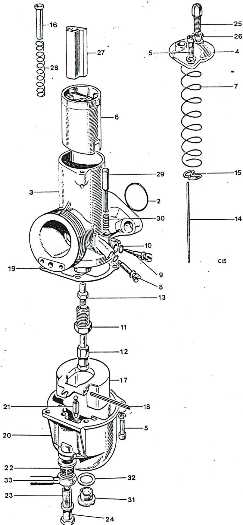
Fig. 5. CARBURETOR T100C
