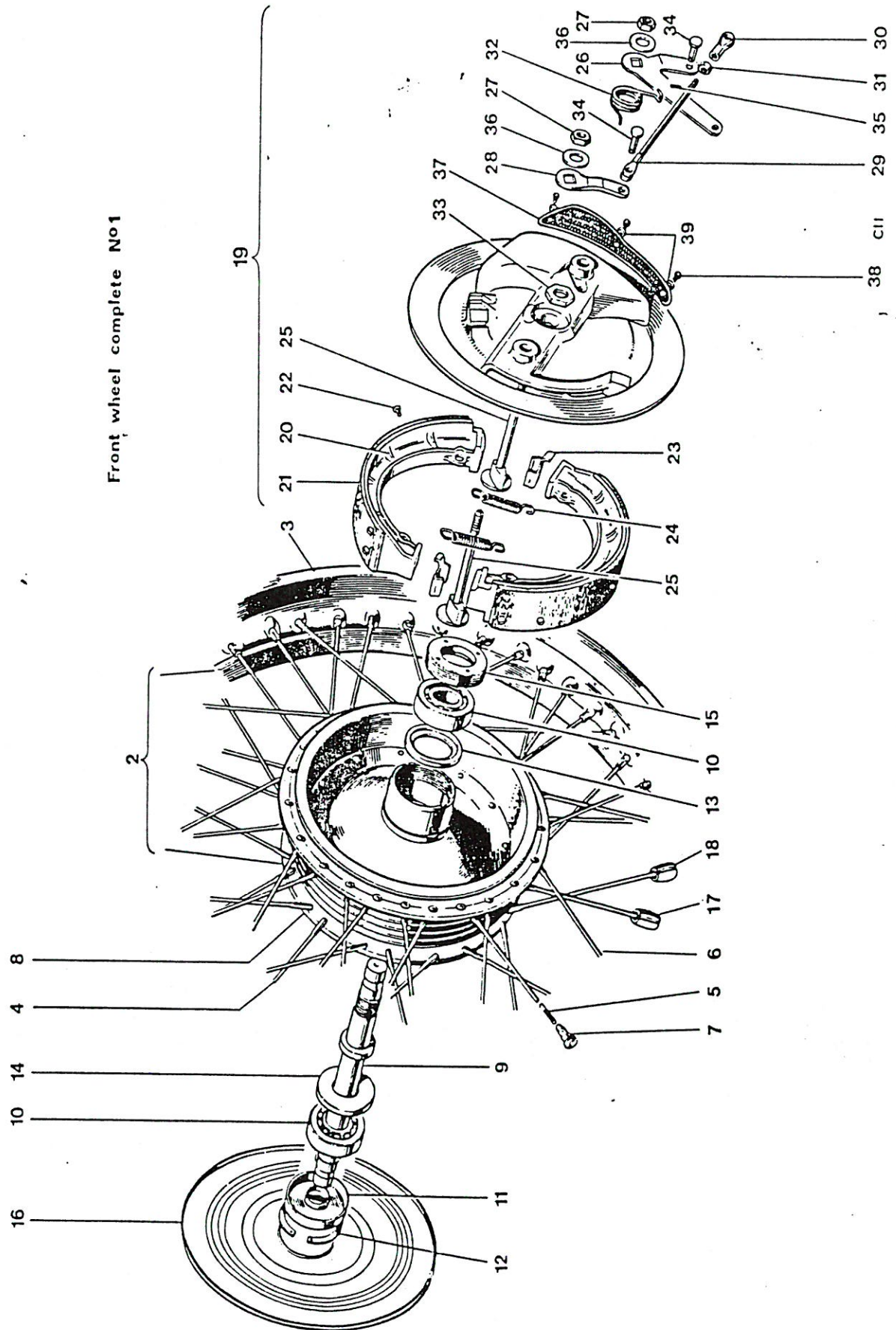
Fig. 21. FRONT WHEEL T100R
