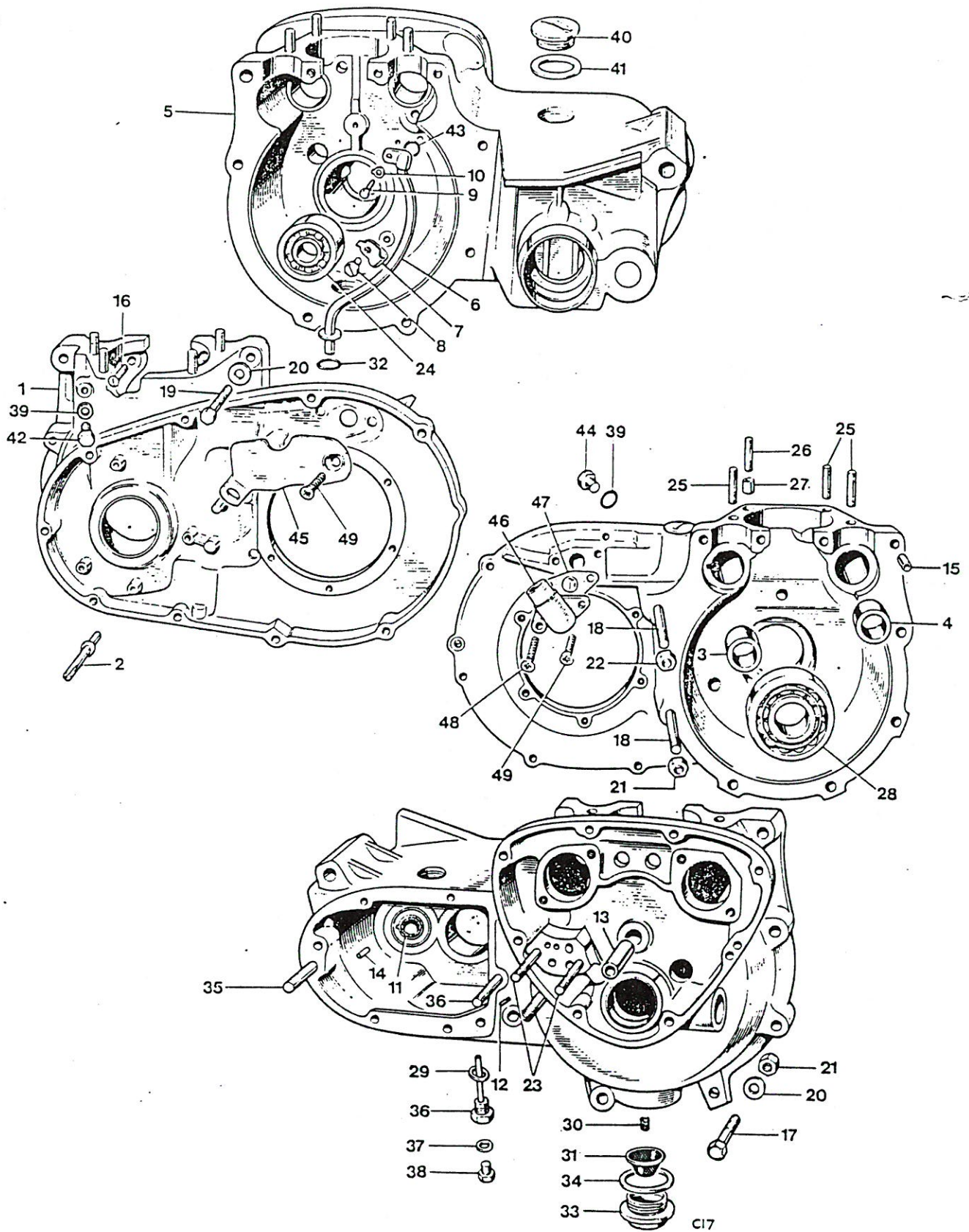
Fig. 2 CRANKCASE
