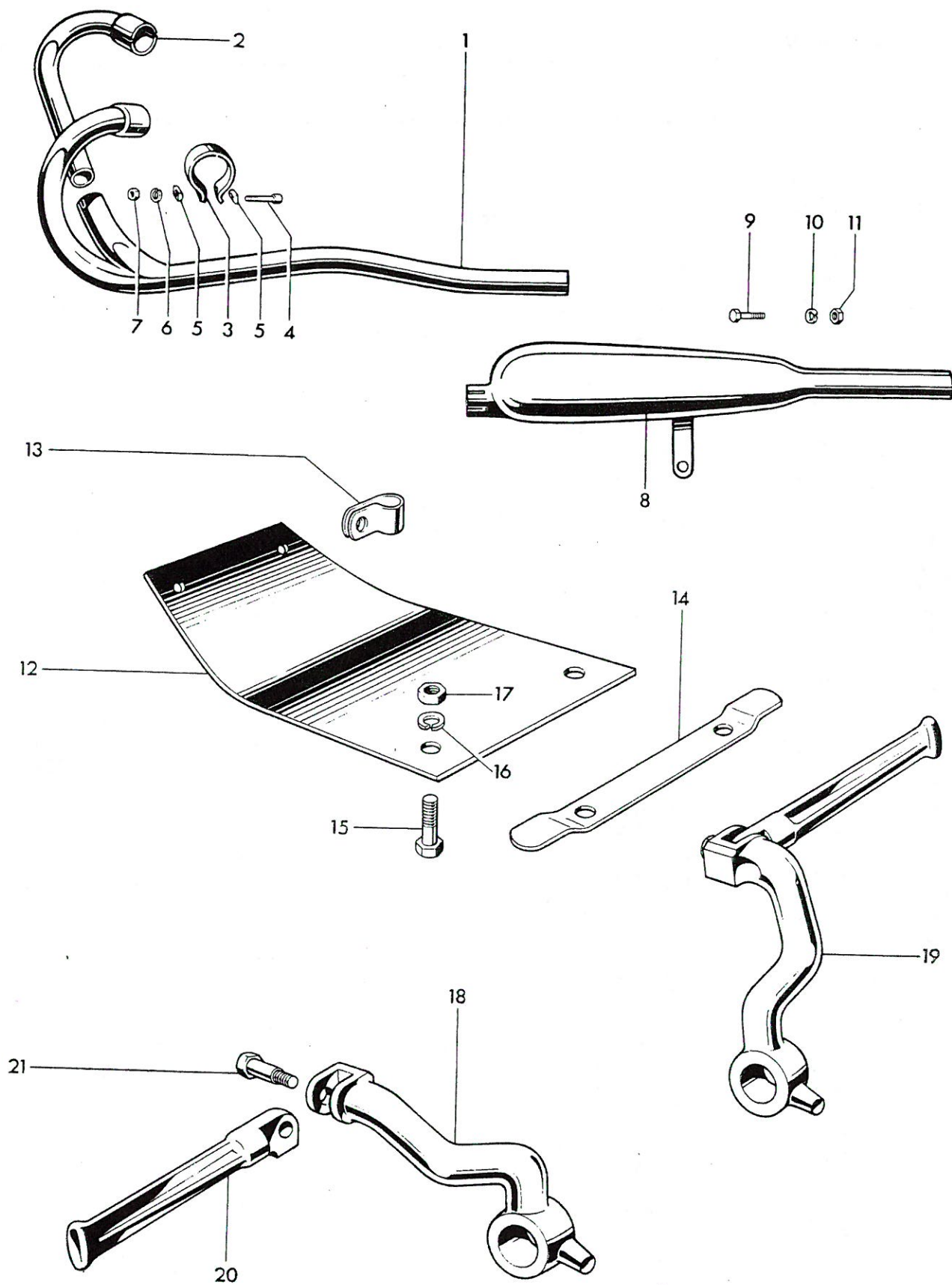
Fig. 12. EXHAUST PIPES, UNDERSHIELD AND FOOTPEGS (T100C)
