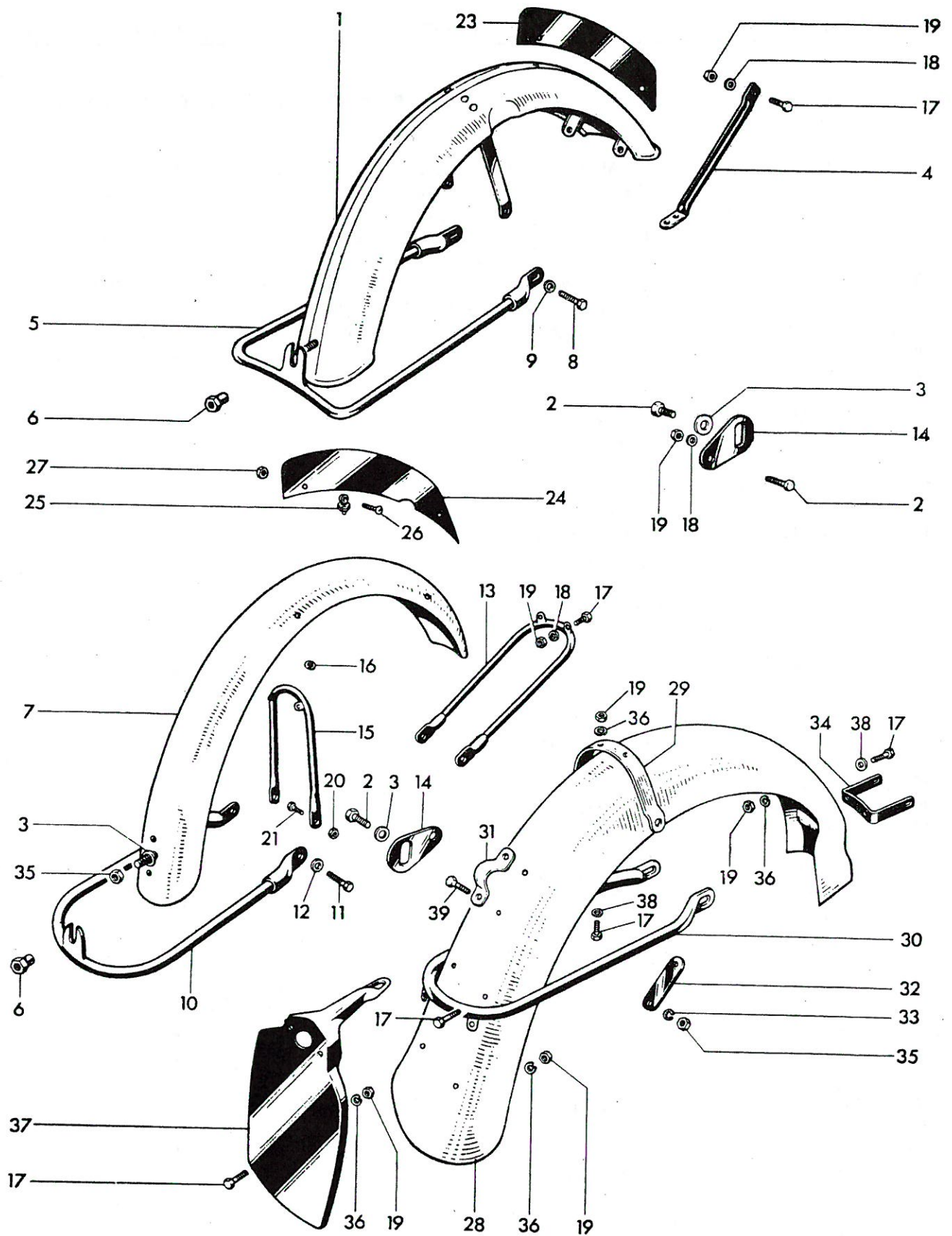
Fig. 22. MUDGUARDS (STANDARD)
