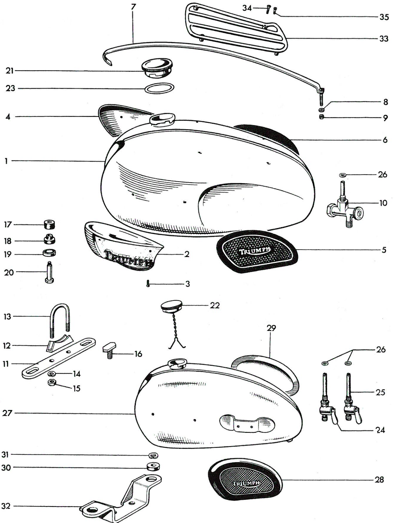
Fig. 25. PETROL TANK
