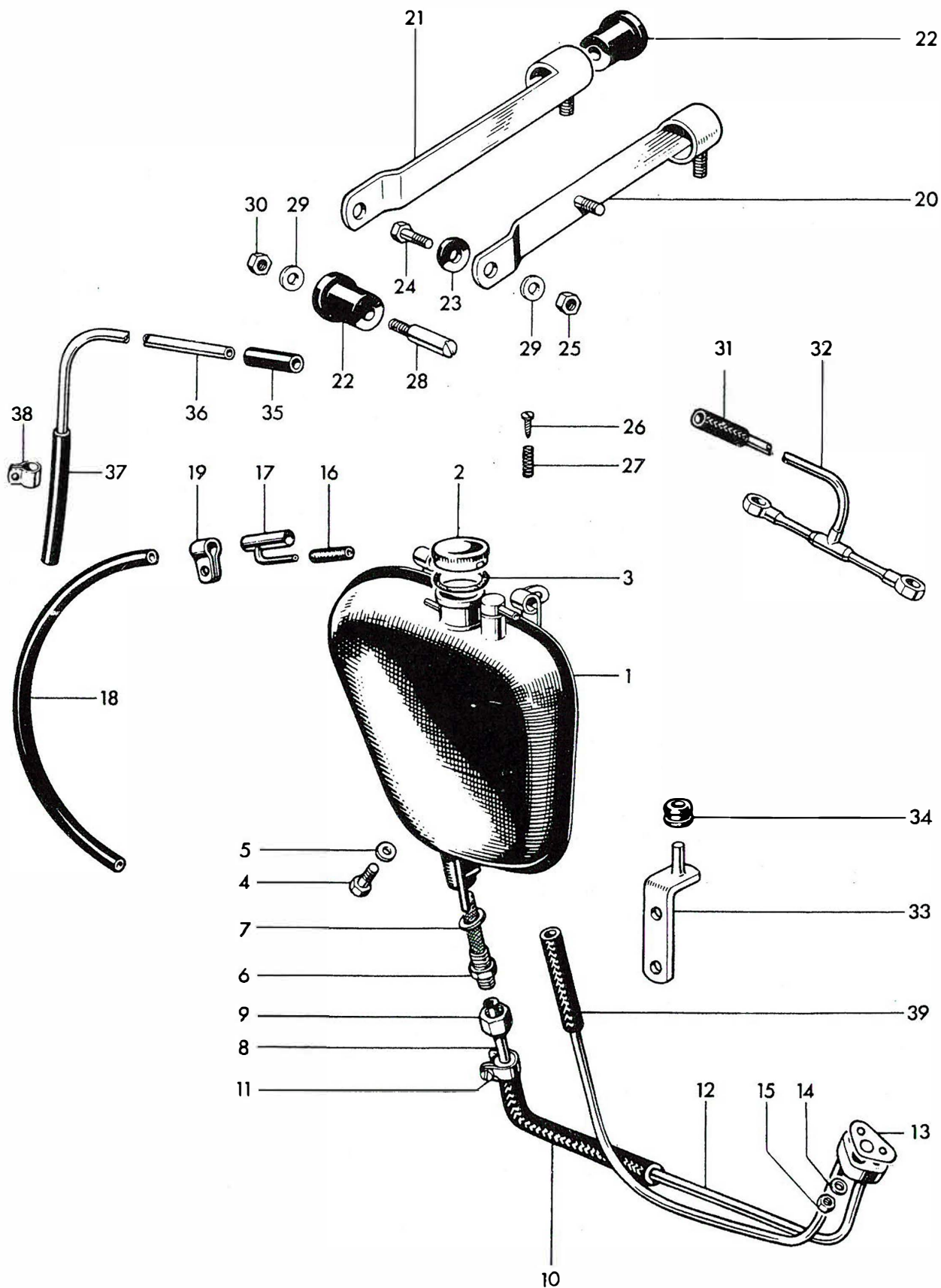
Fig. 26. OIL TANK
