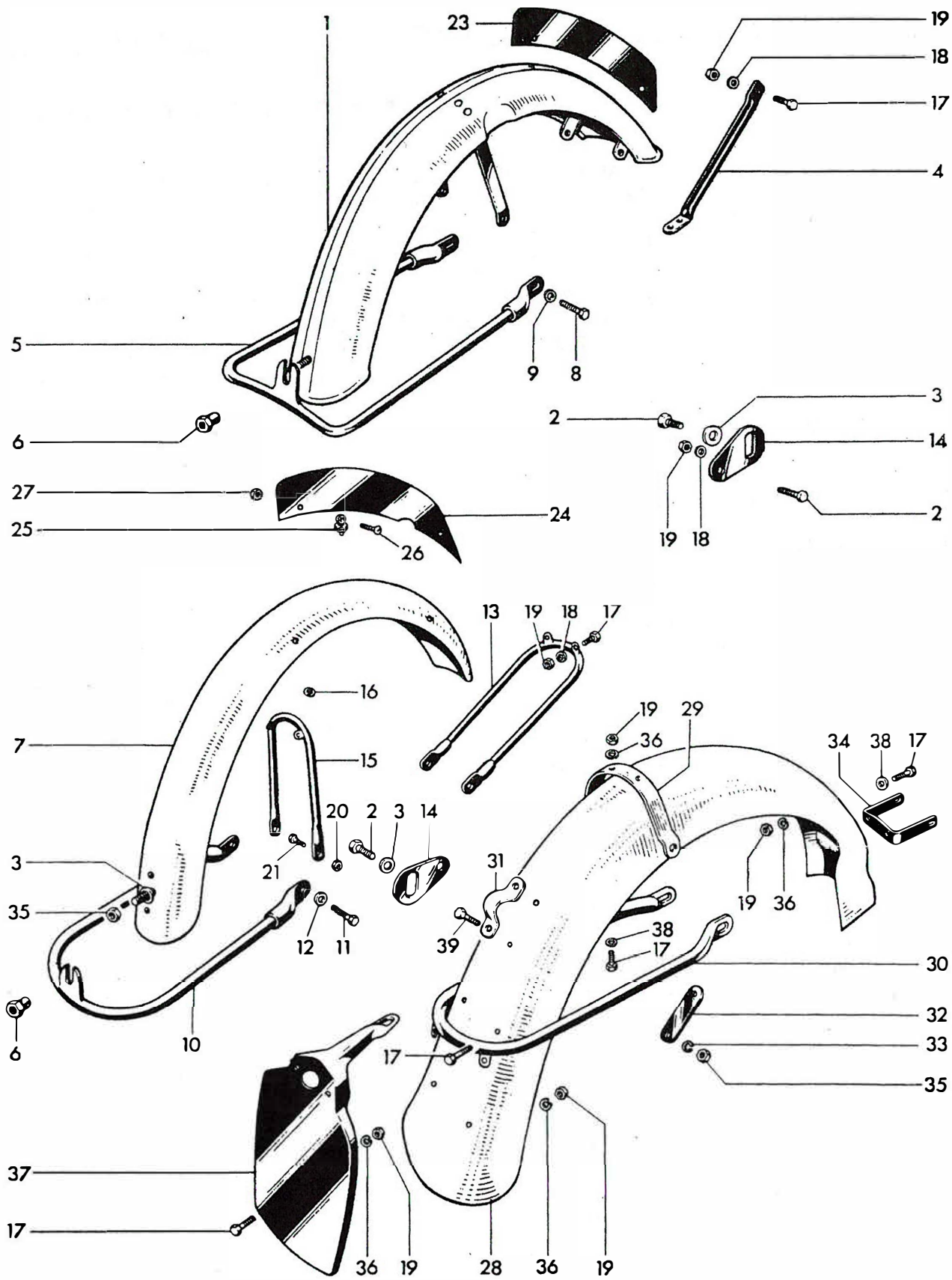
Fig. 22. MUDGUARDS (STANDARD)
