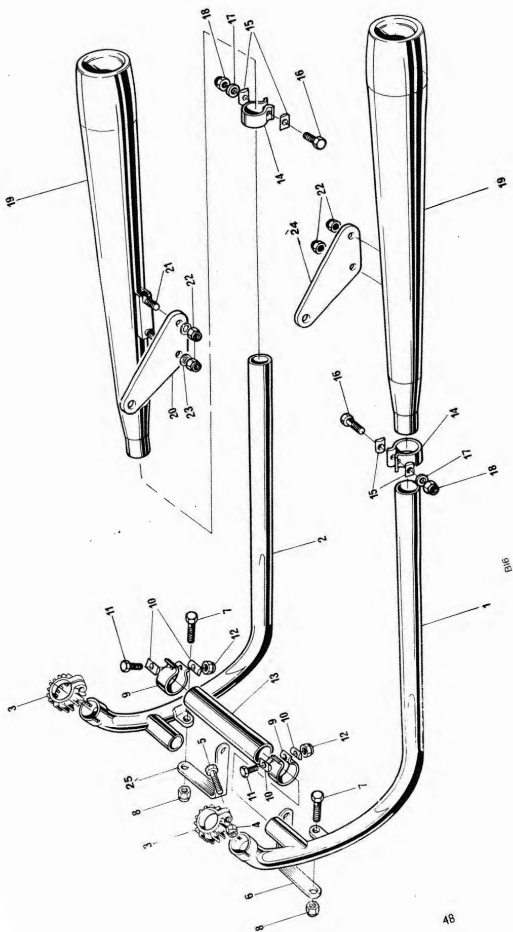
EXHAUST PIPES AND MUFFLERS Fig. 19.
