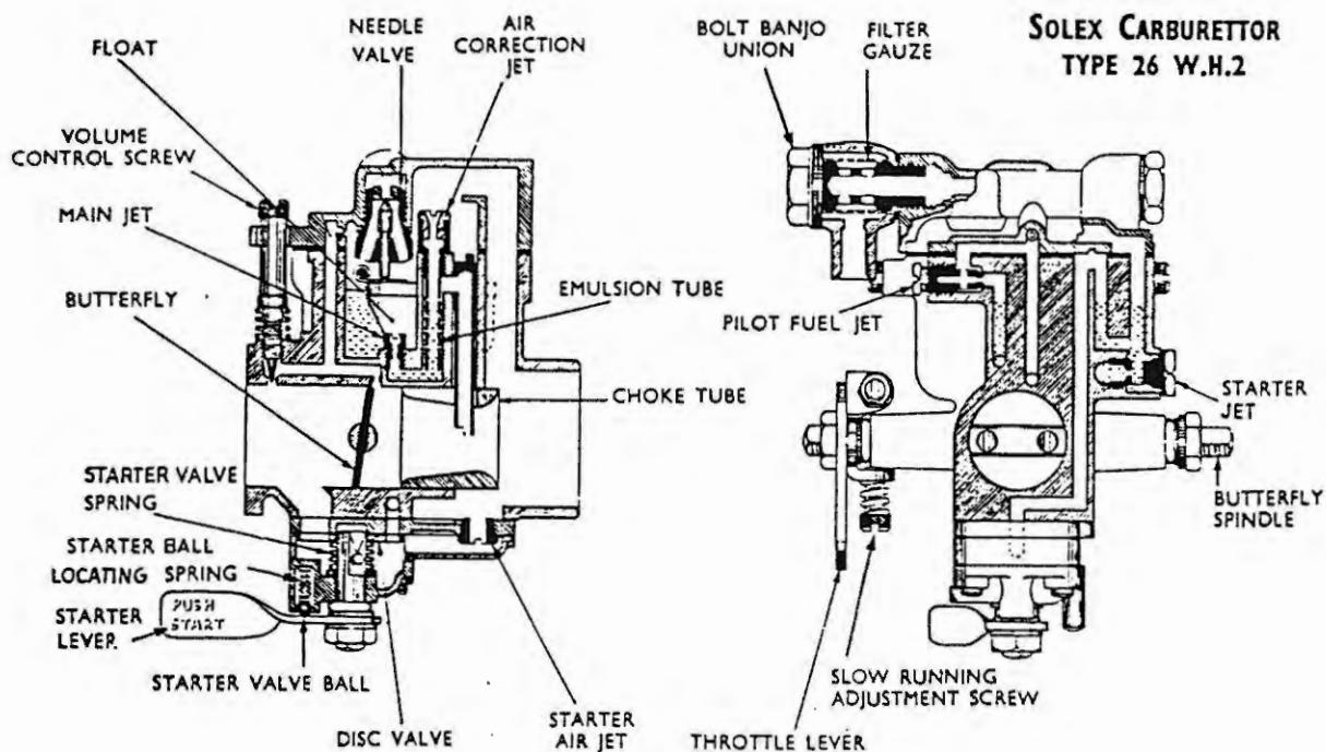
Fig. 12. SOLEX CARBURETTER.
