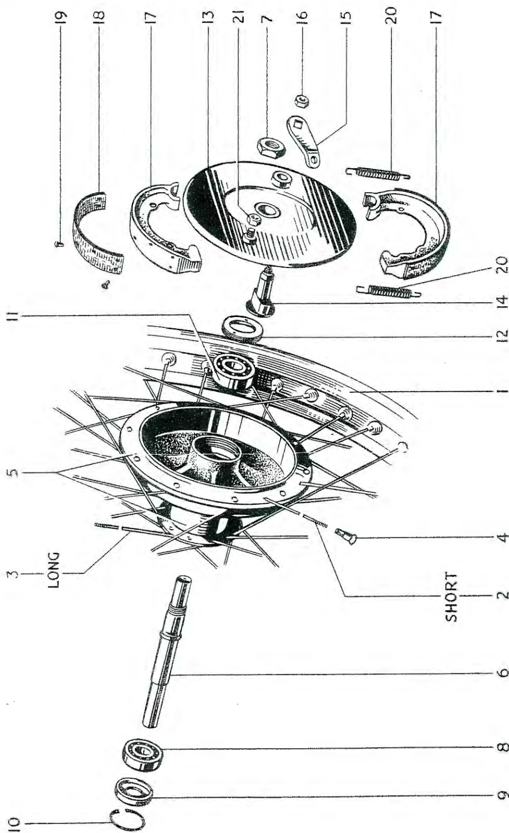
FIG. 7. FRONT WHEEL.
