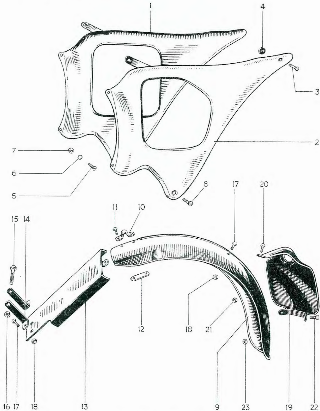
FIG. 10. REAR PANELS.
