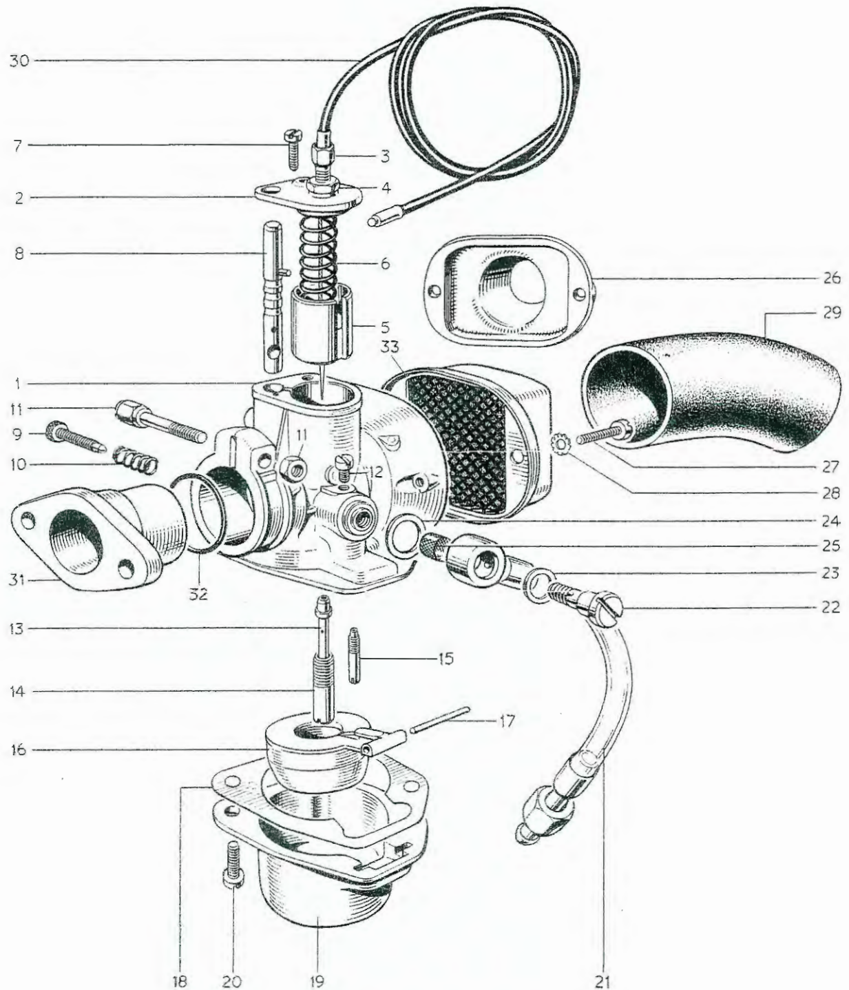
FIG. 15. ZENITH CARBURETTER
