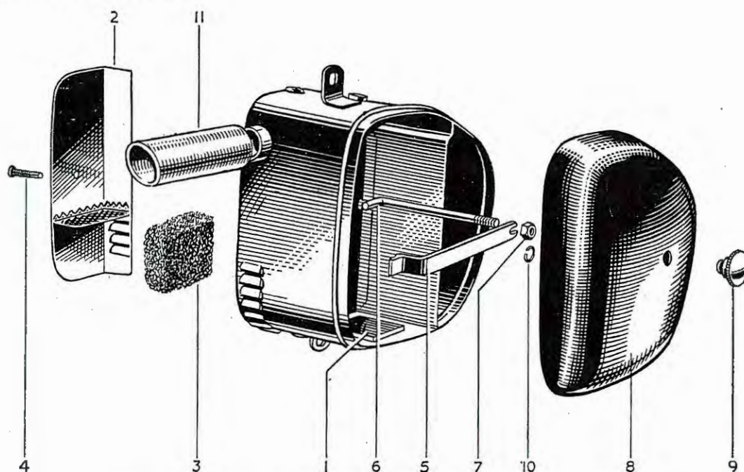
FIG. 10. TOOLBOX, BATTERY CARRIER AND AIR CLEANER.
