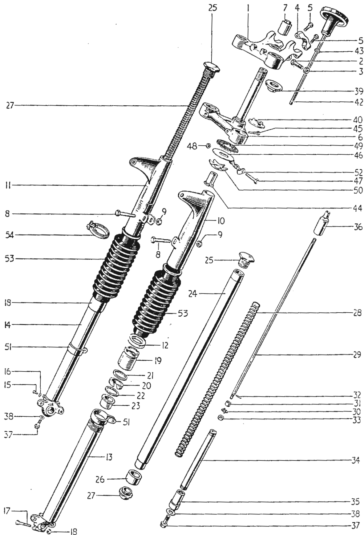
FIG. 16. TELESCOPIC FORK (TROPHY)
