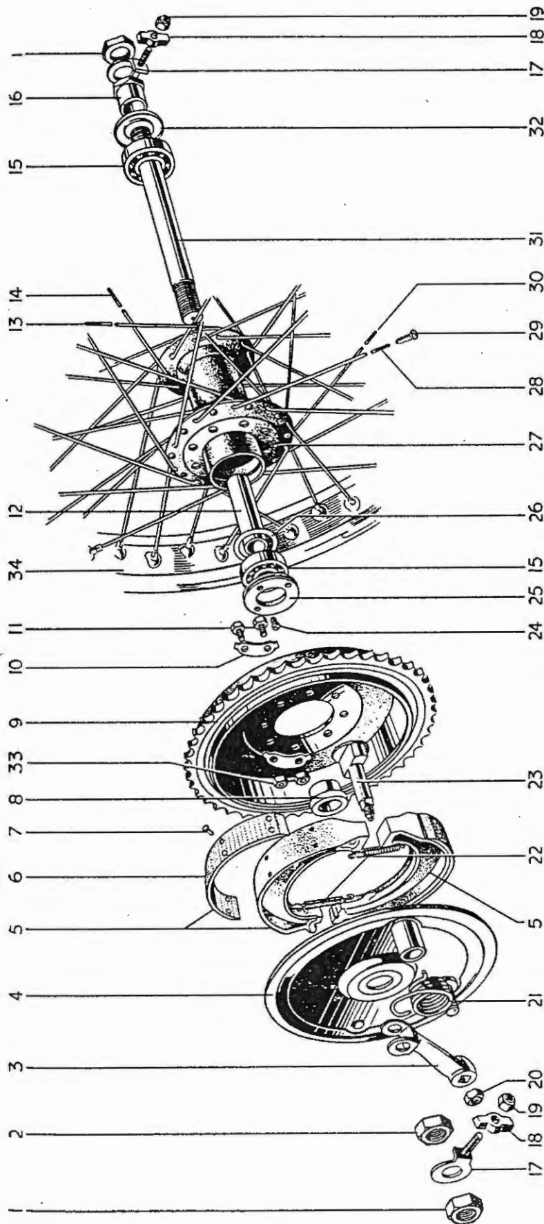
FIG. 19. REAR WHEEL
