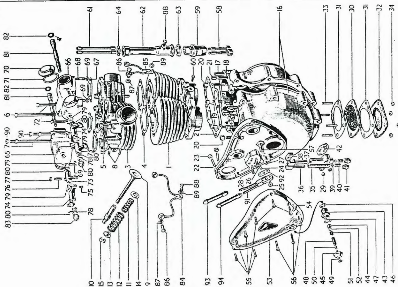
FIG. 4. CRANKCASE, CYLINDER BLOCK, CYLINDER HEAD, etc.
