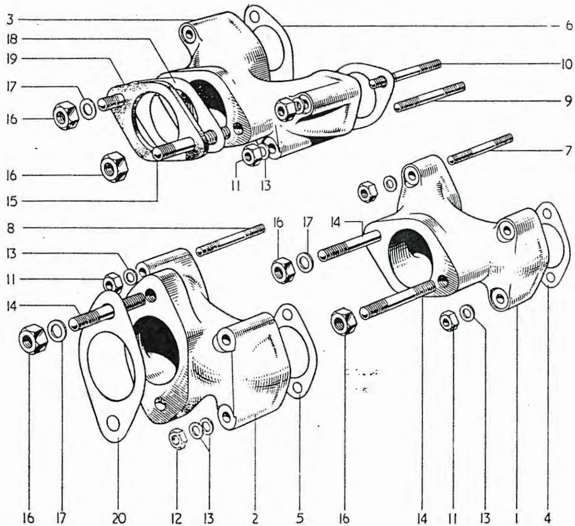
FIG. 1. INLET MANIFOLDS
