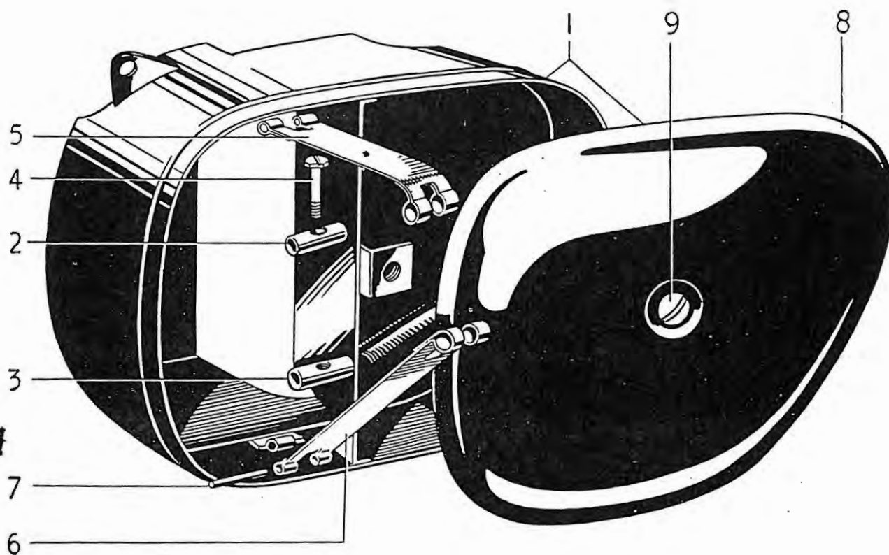
FIG. 26. BATTERY CARRIER AND TOOL BOX
