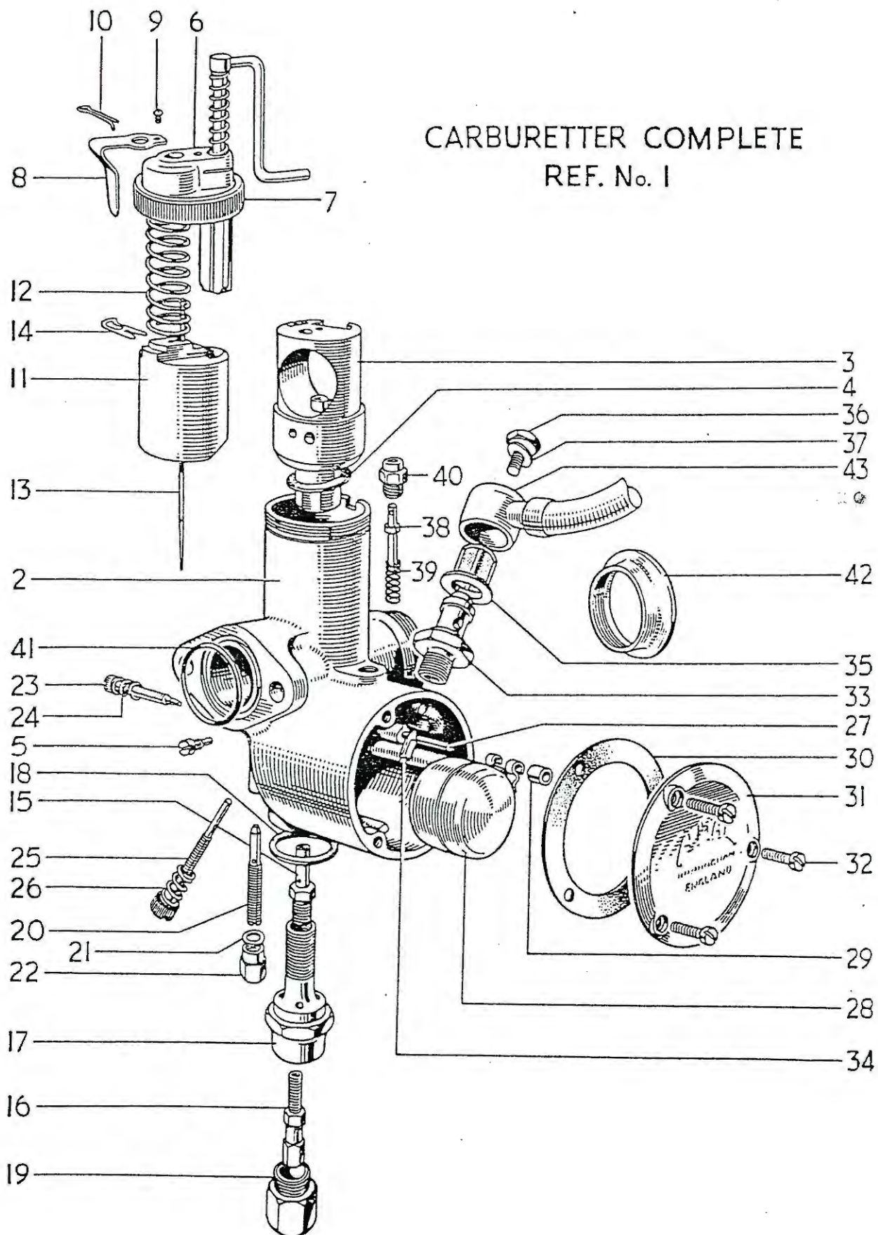
Fig. 28. CARBURETTER, 3TA and 5TA
