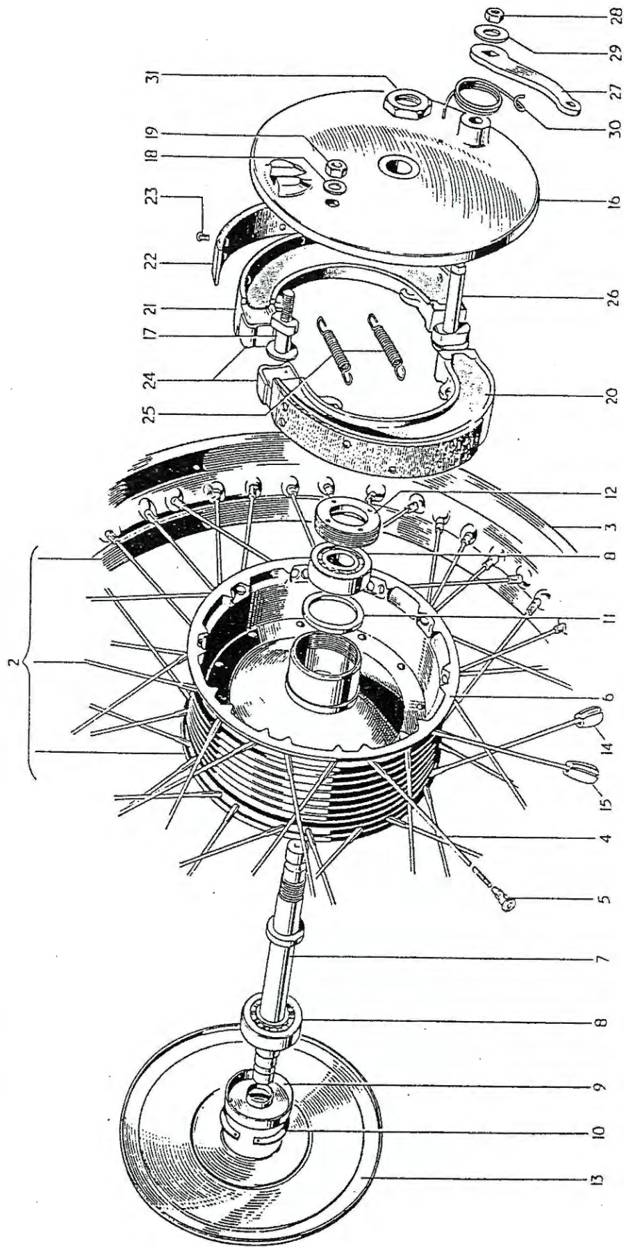
Fig. 17. FRONT WHEEL
