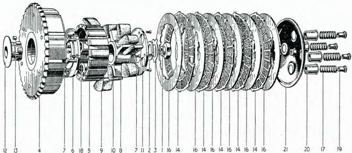
FIG. II. CLUTCH AND SHOCK ABSORBER
