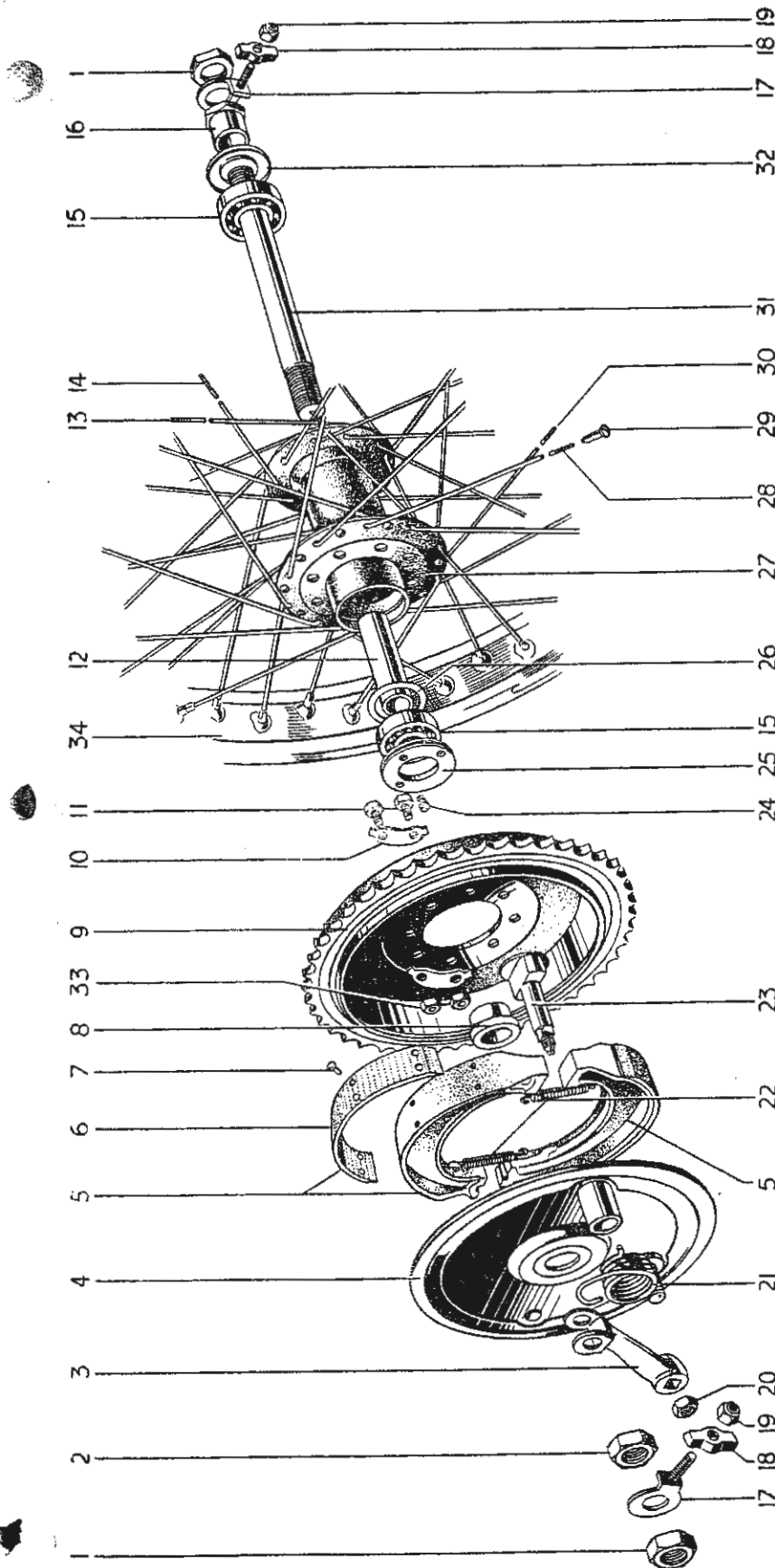
FIG. 19. REAR WHEEL
