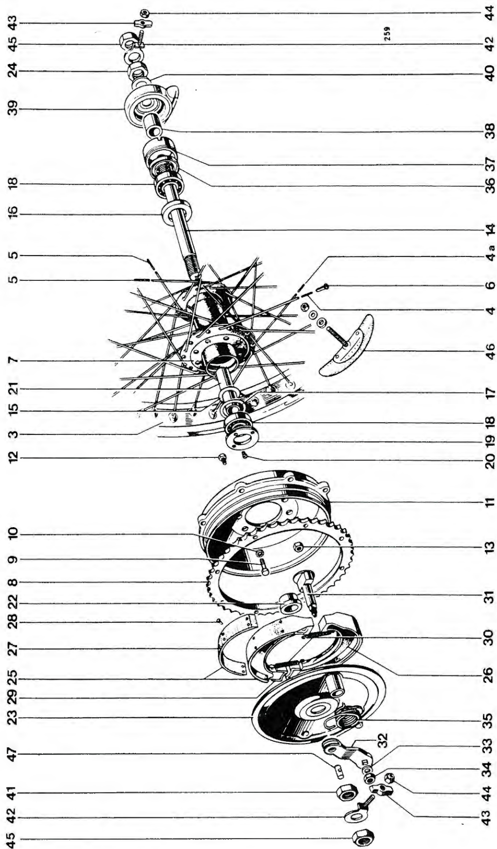
Fig. 21. REAR WHEEL
