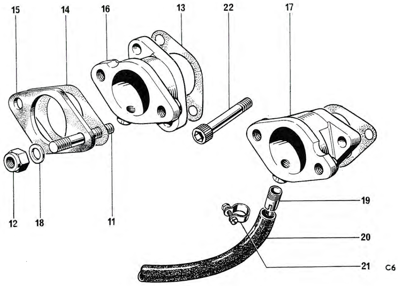
Fig. 4. INLET MANIFOLDS
