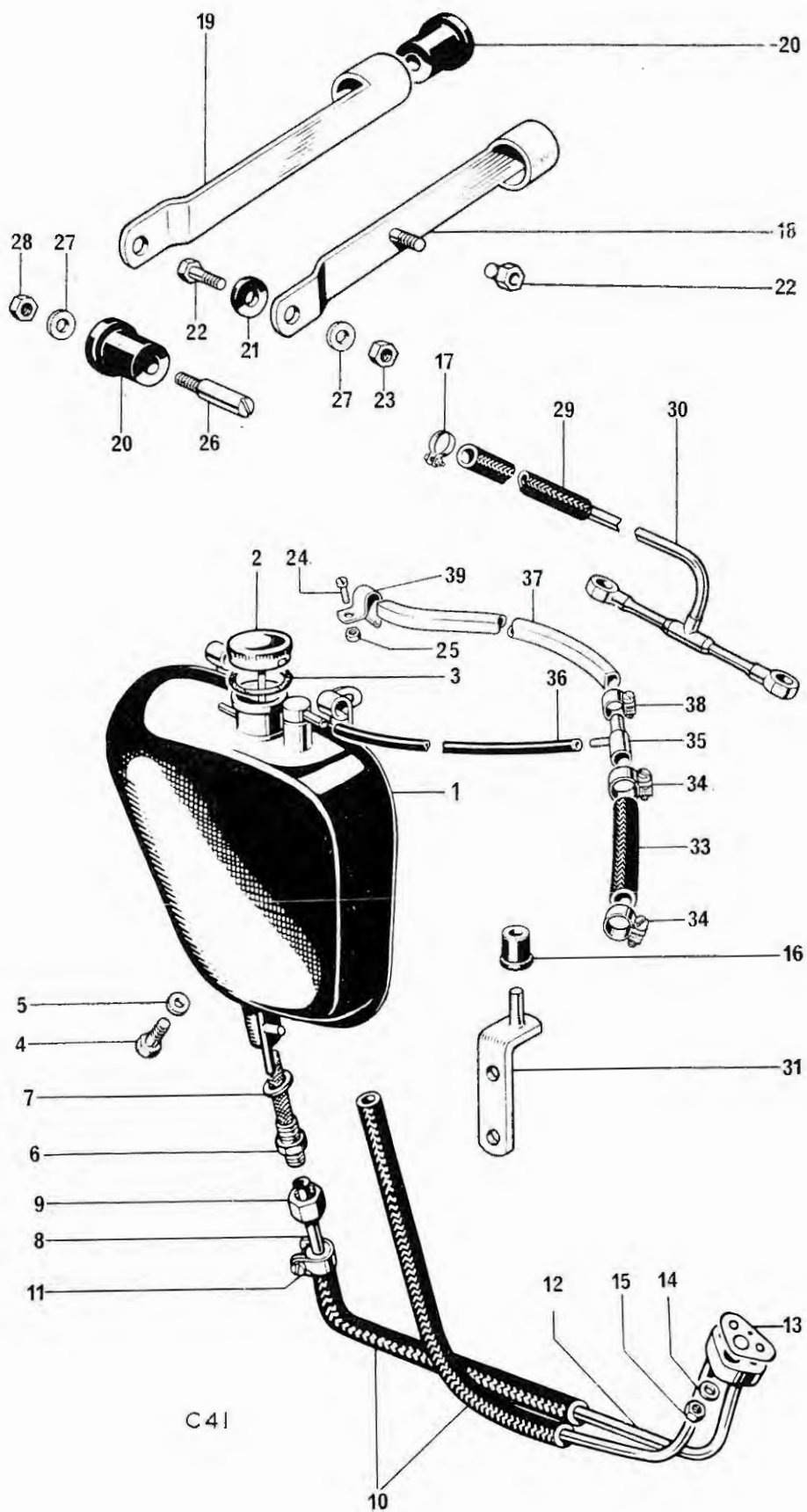
Fig. 26. OIL TANK
