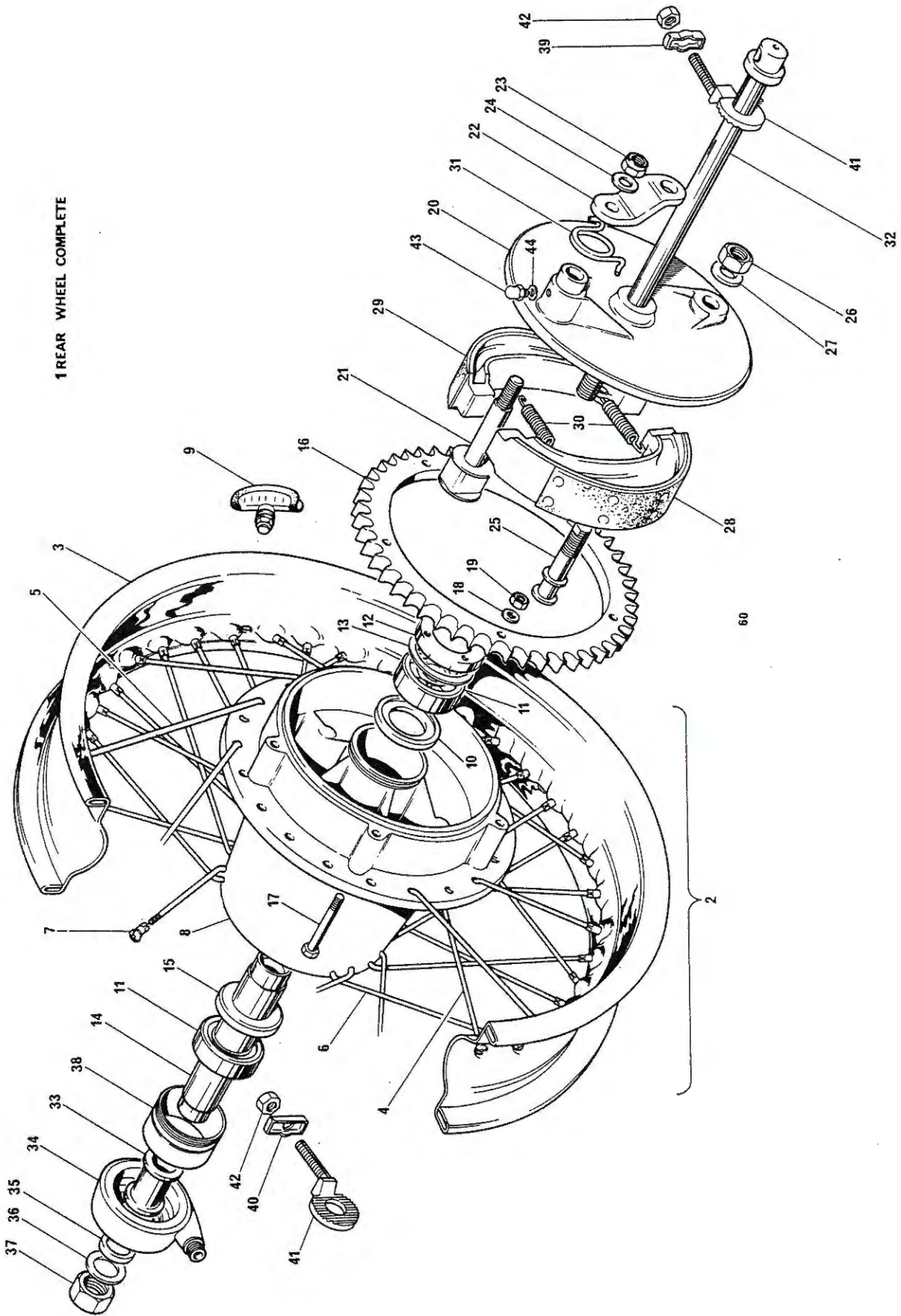
Fig. 22. REAR WHEEL
