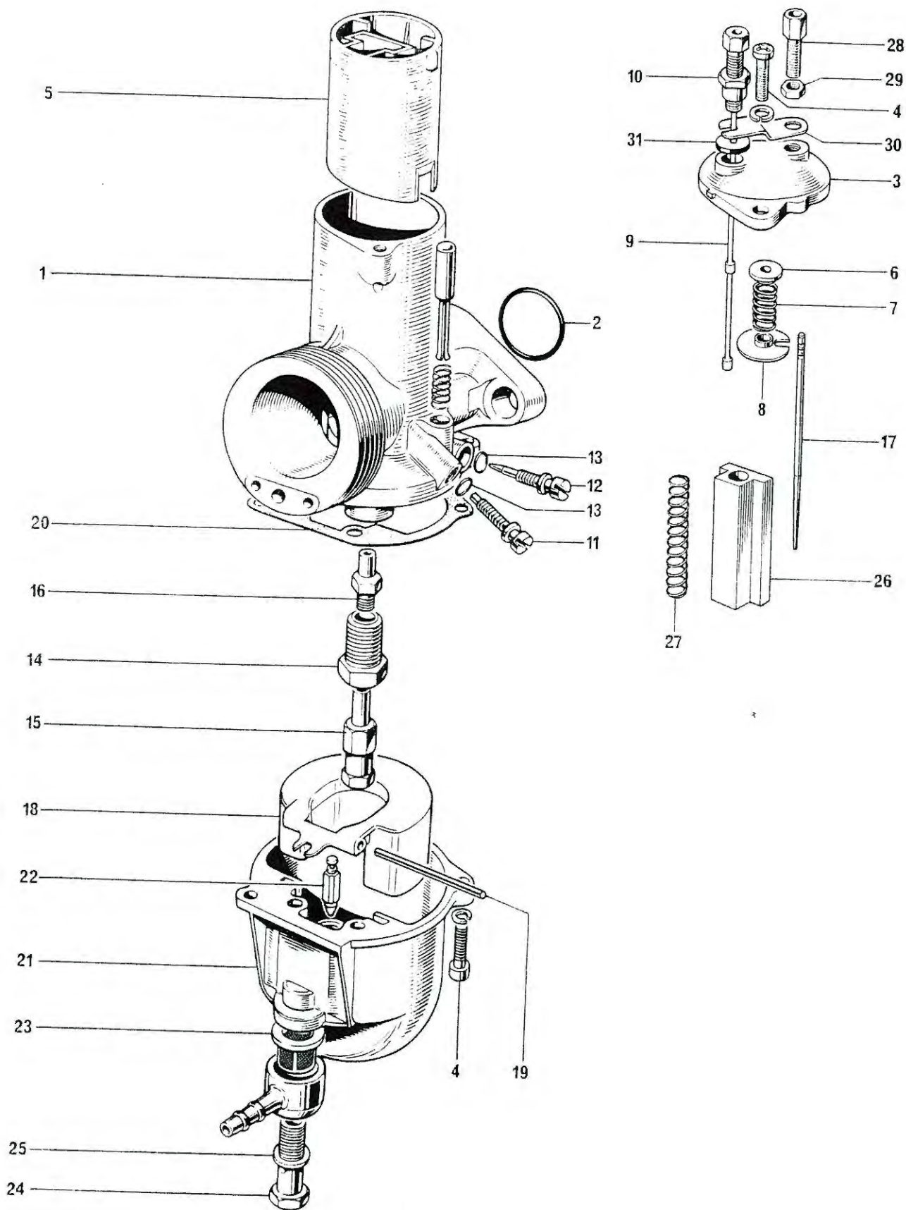
Fig. 31. AMAL CARBURETTER AND AIR CLEANER CONNECTIONS
