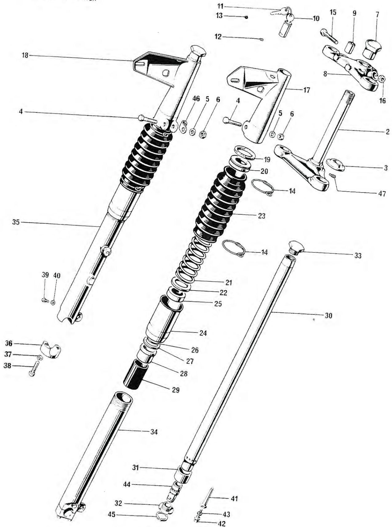
Fig. 18. TELESCOPIC FRONT FORK
