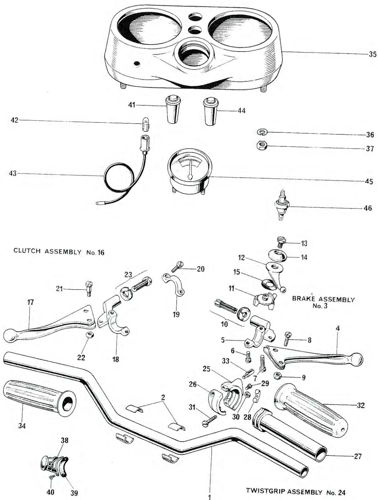
Fig. 28. HANDLEBARS, CONTROLS, BINNACLE AND OIL WARNING LIGHT
