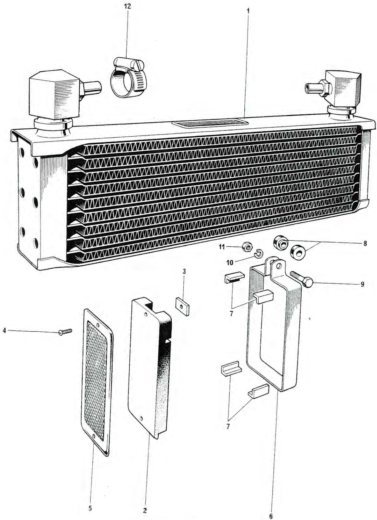
Fig. 22. OIL COOLER
