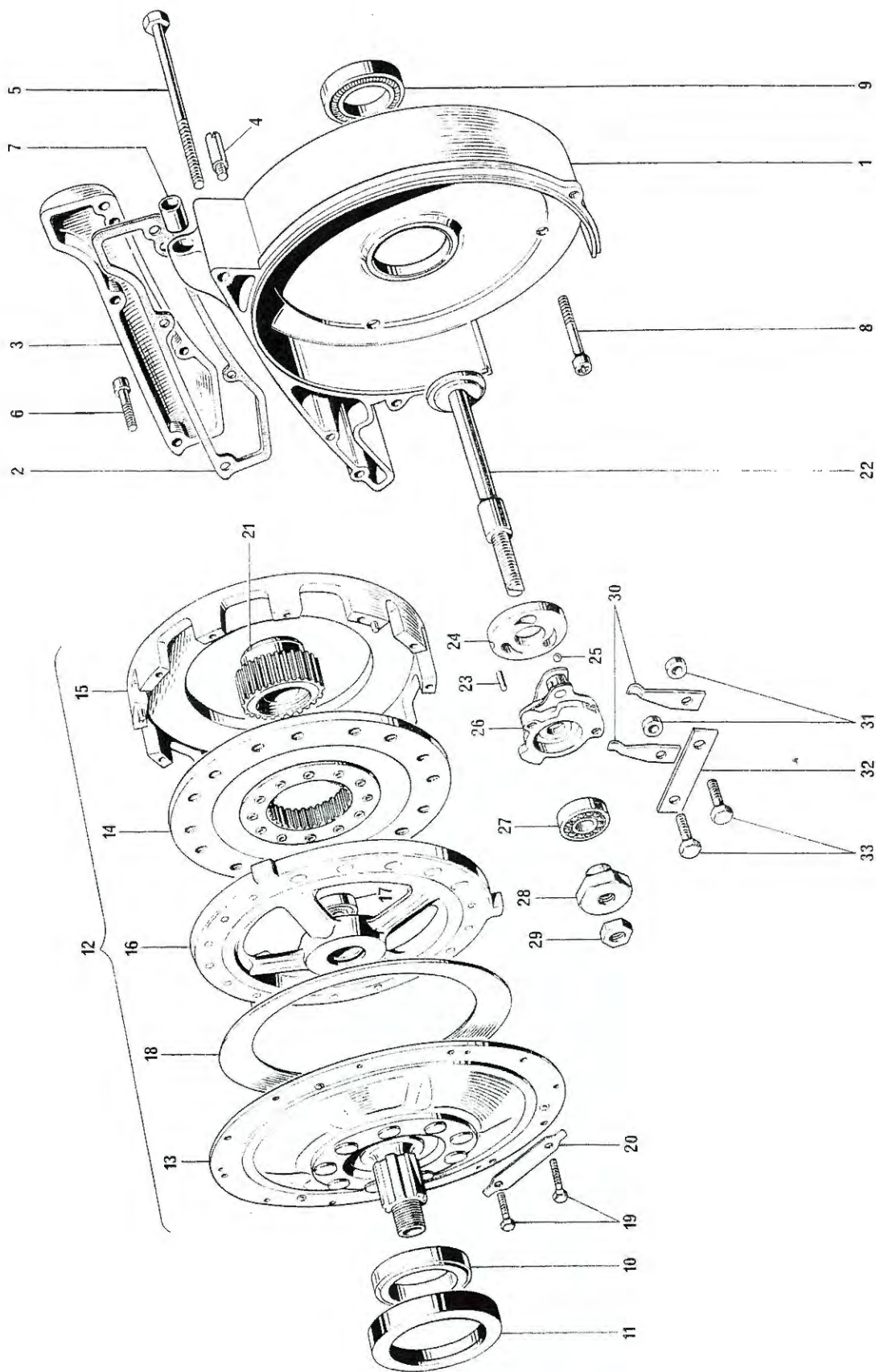
Fig. 11. CLUTCH AND CLUTCH OPERATION
