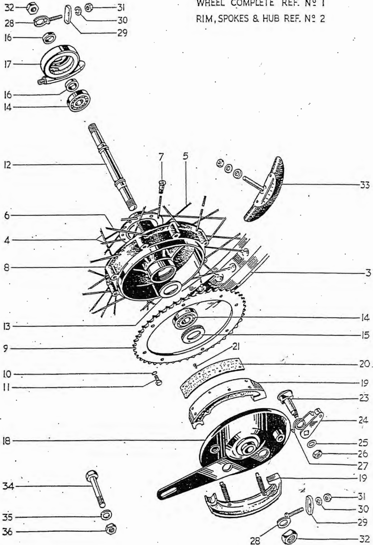
Fig. 11. REAR WHEEL
