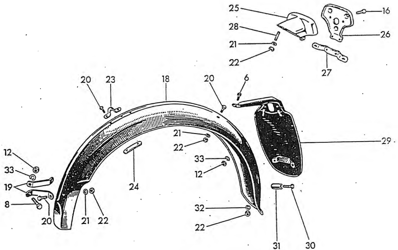
Fig. 12. MUDGUARDS AND NUMBER PLATES
