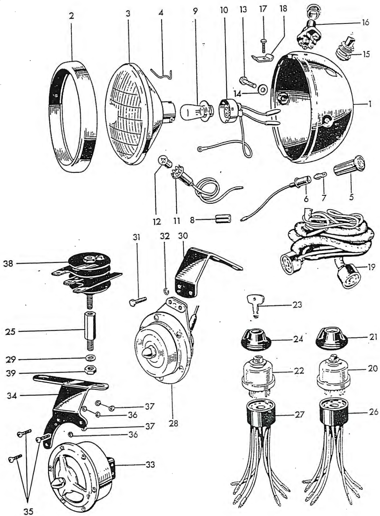
Fig. 19. ELECTRICAL EQUIPMENT
