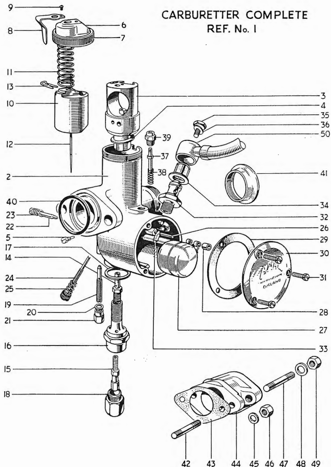
Fig. 23. AMAL CARBURETTER.
