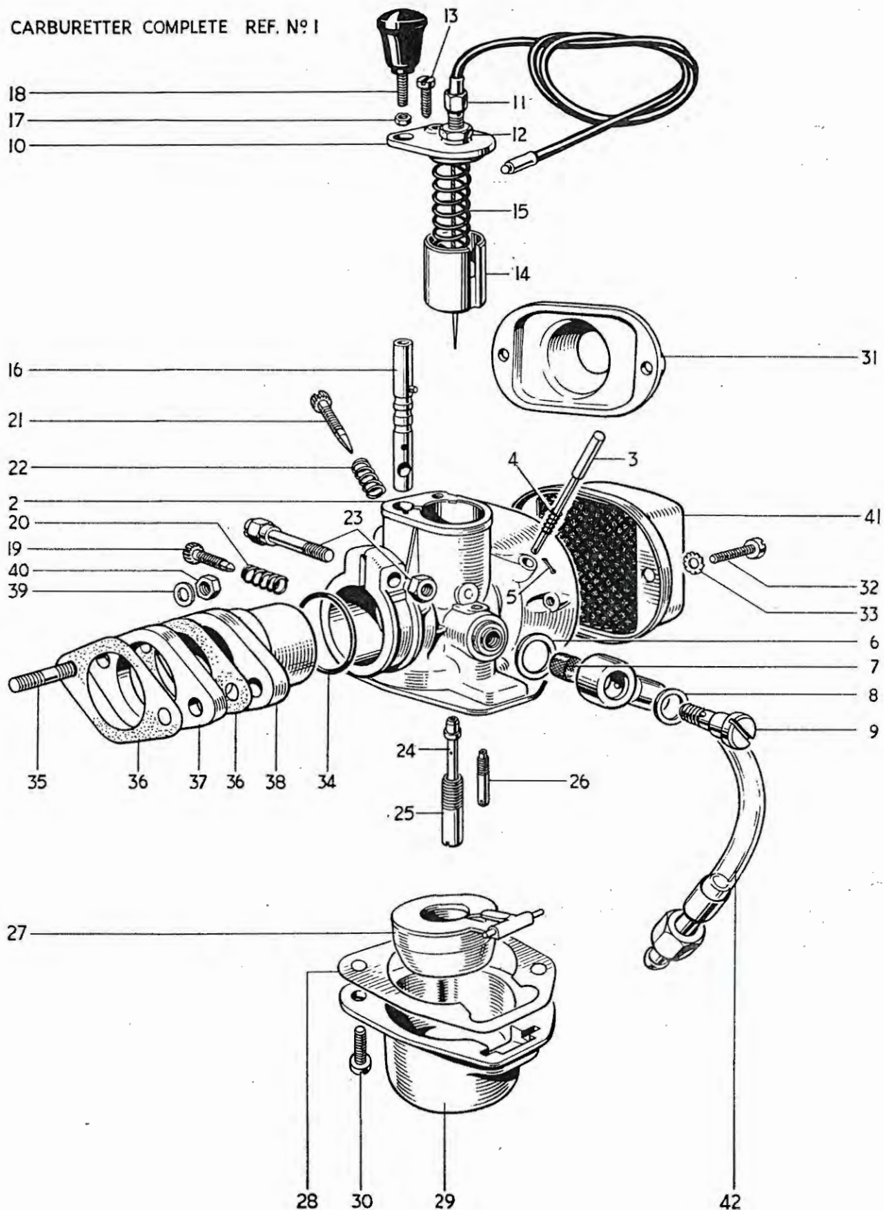
Fig. 24. ZENITH CARBURETTER.
