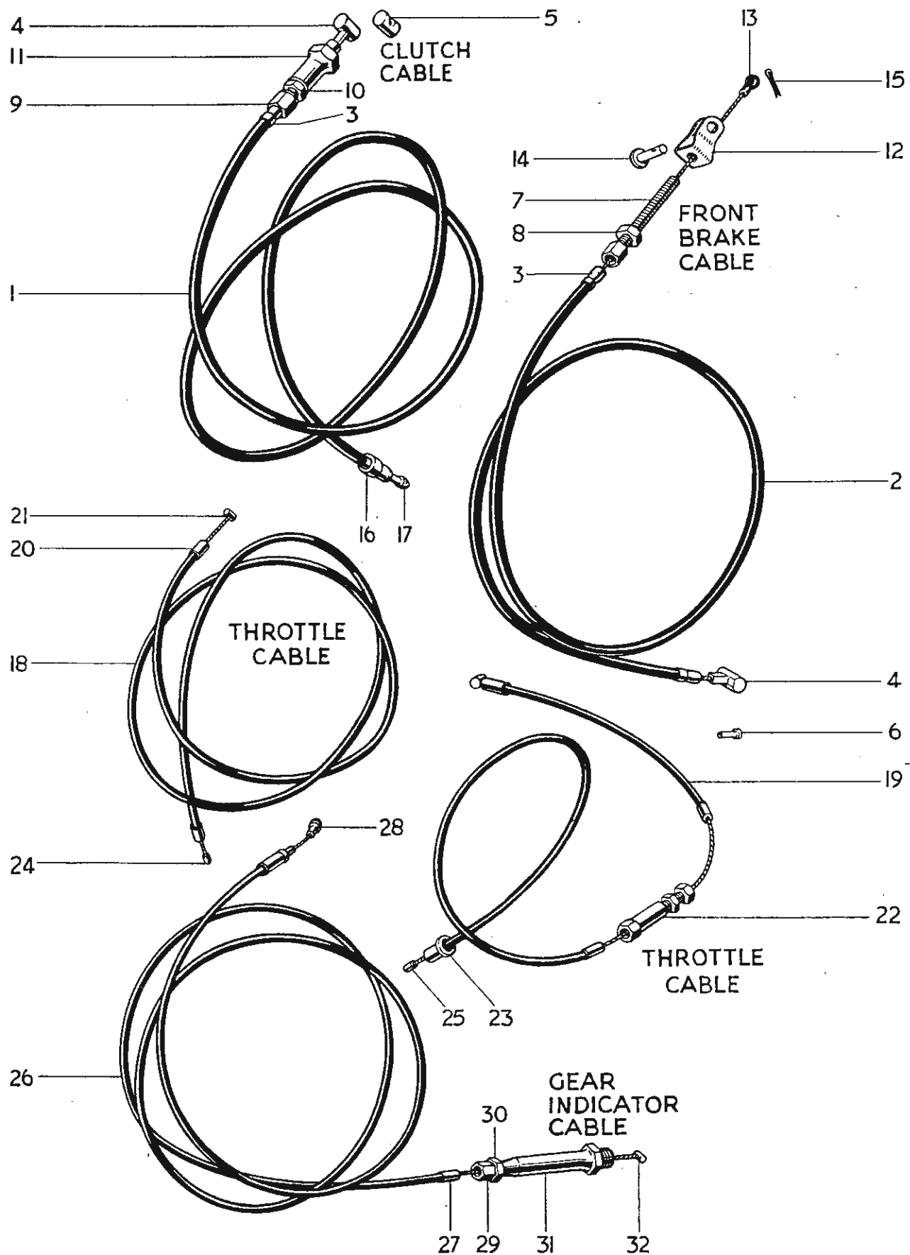
Fig. 22. CONTROL CABLES.
