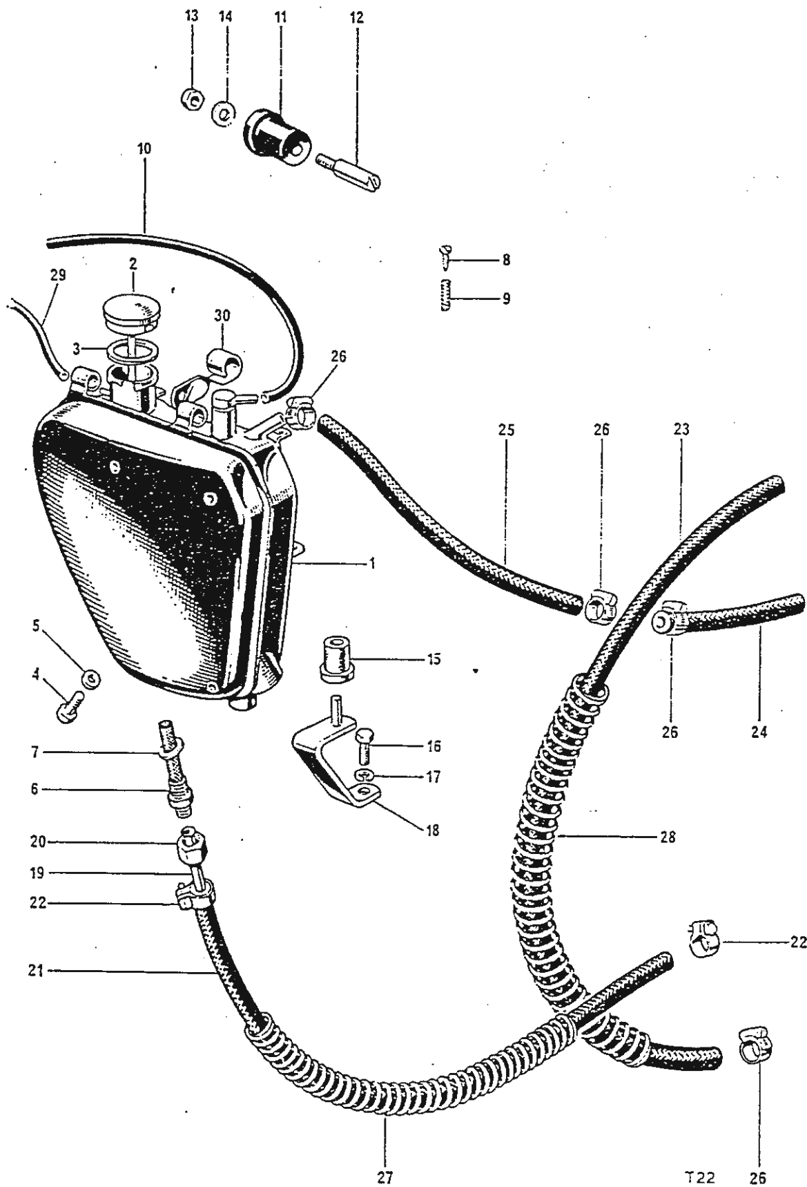
Fig. 26. OIL TANK
