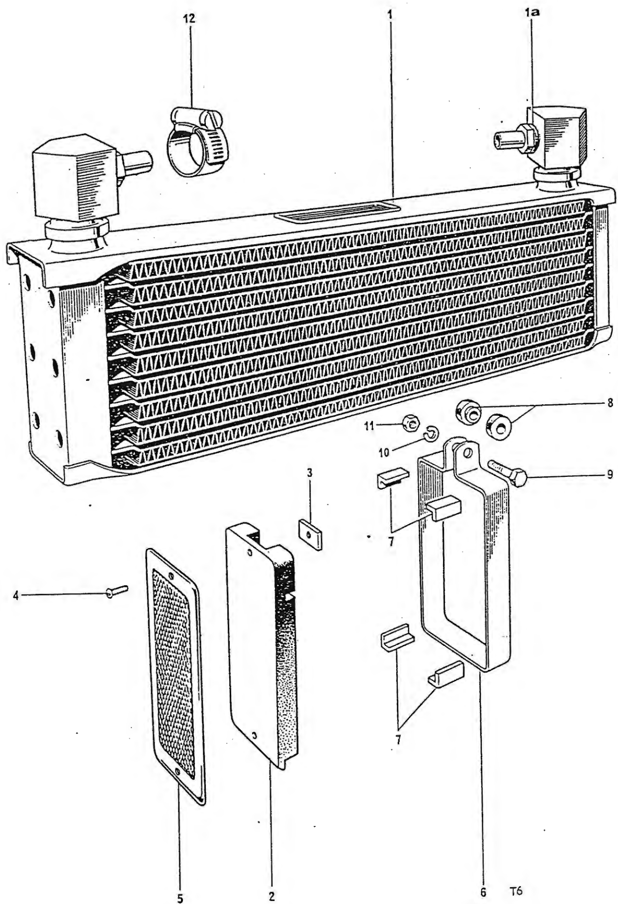
Fig. 24. OIL COOLER
