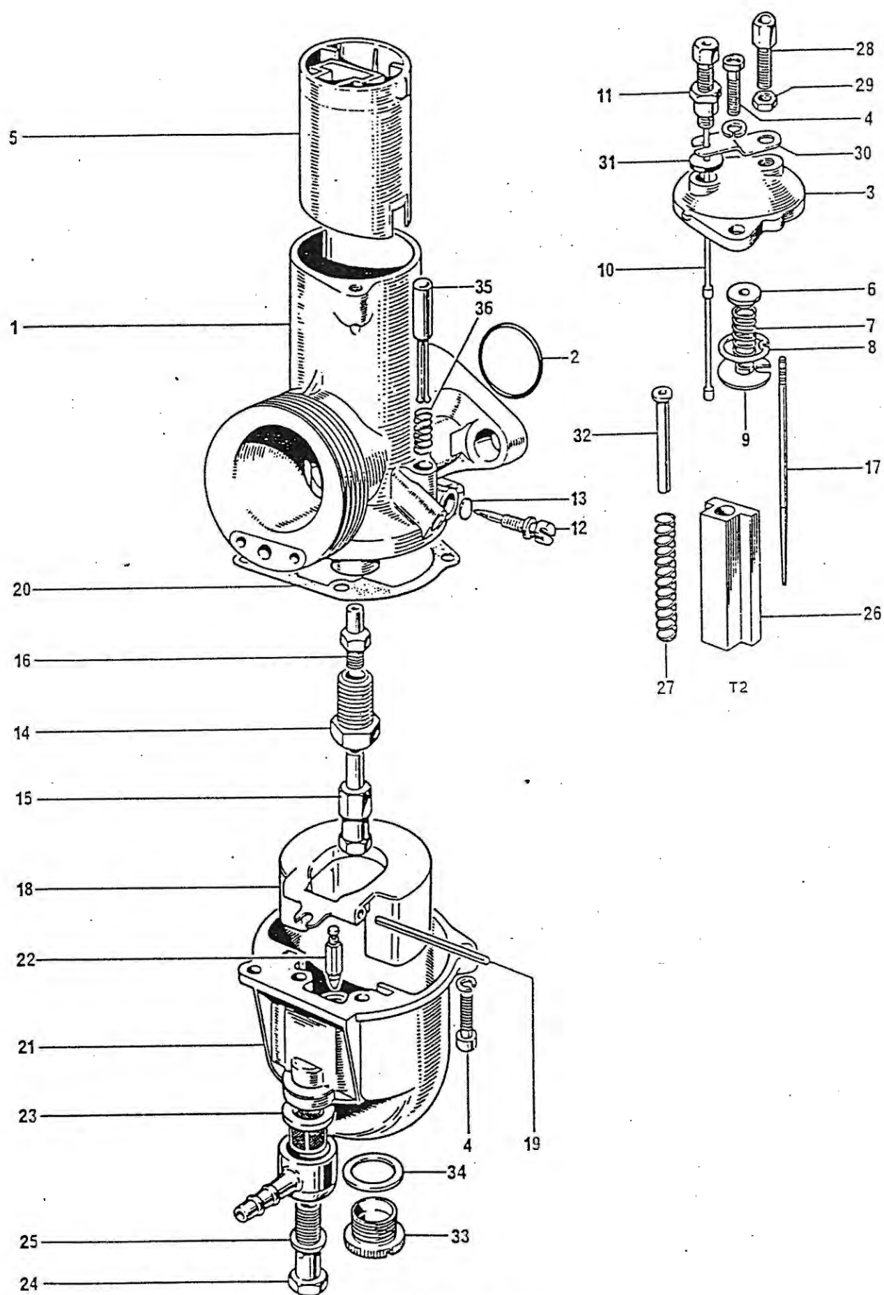
Fig. 5. CARBURETORS
