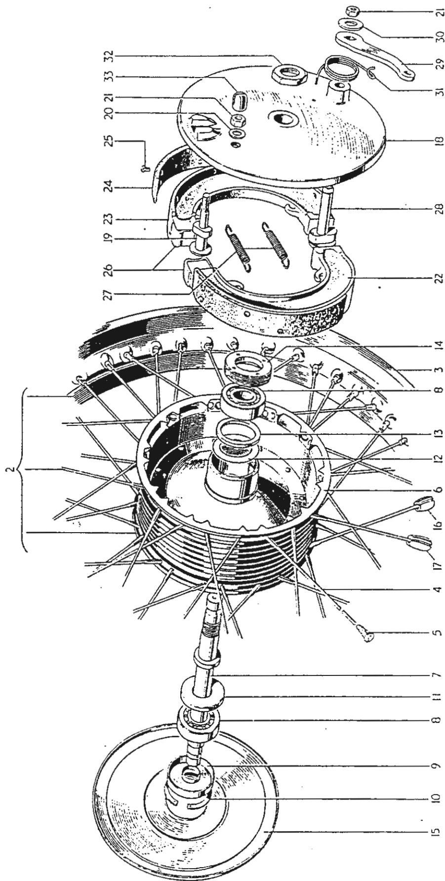
FIG. 19. FRONT WHEEL
