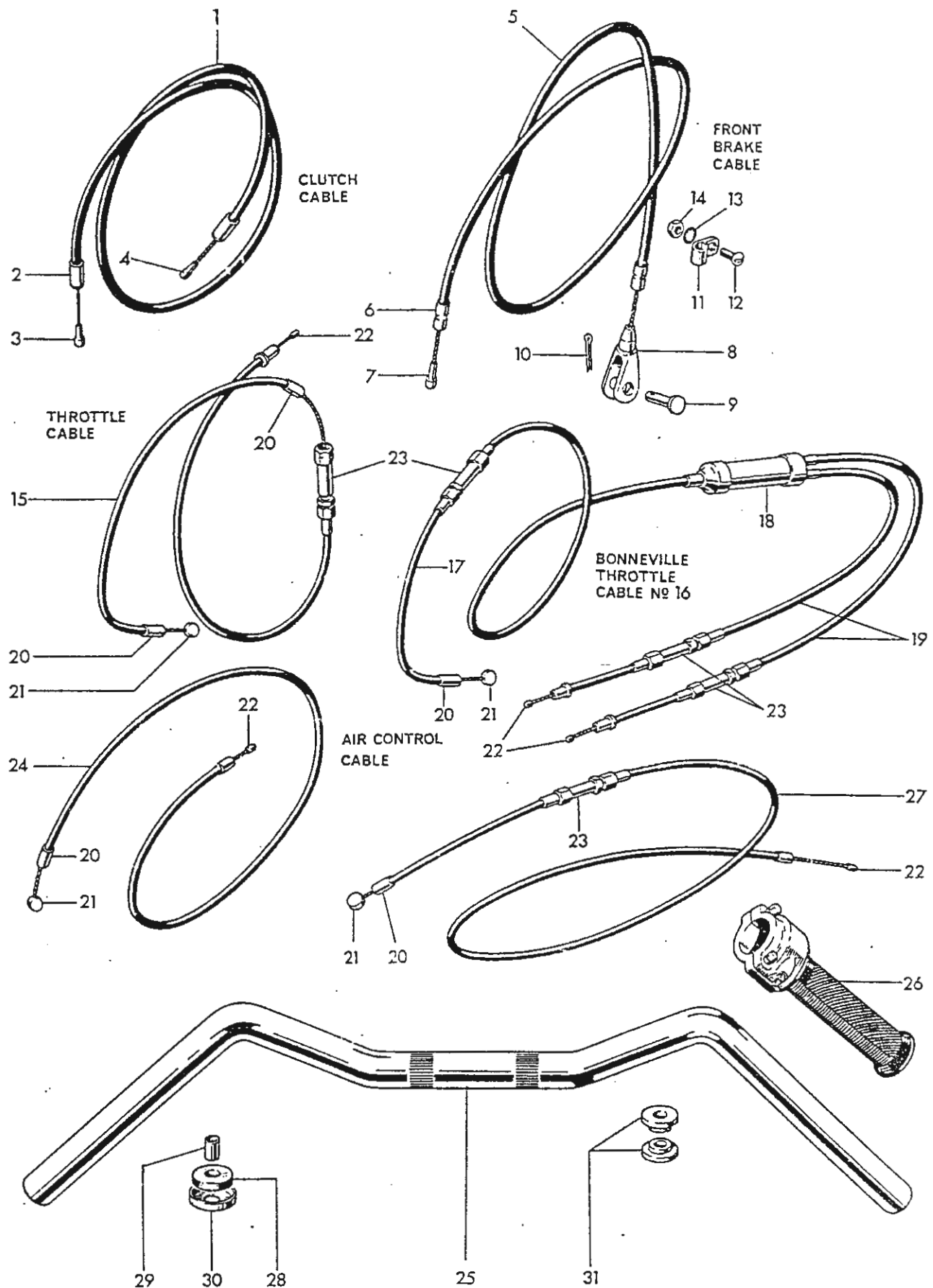
Fig. 28. CONTROL CABLES AND AMERICAN HANDLEBARS
