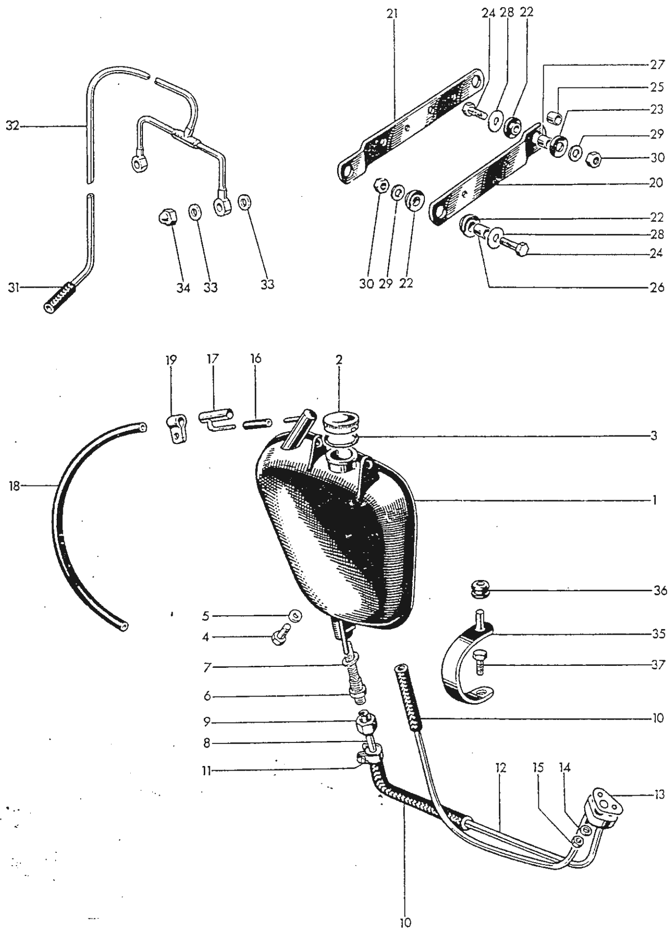
Fig. 23. OIL TANK
