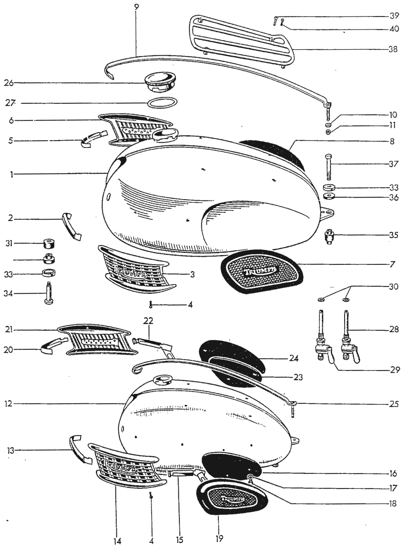
Fig. 22. PETROL TANKS
