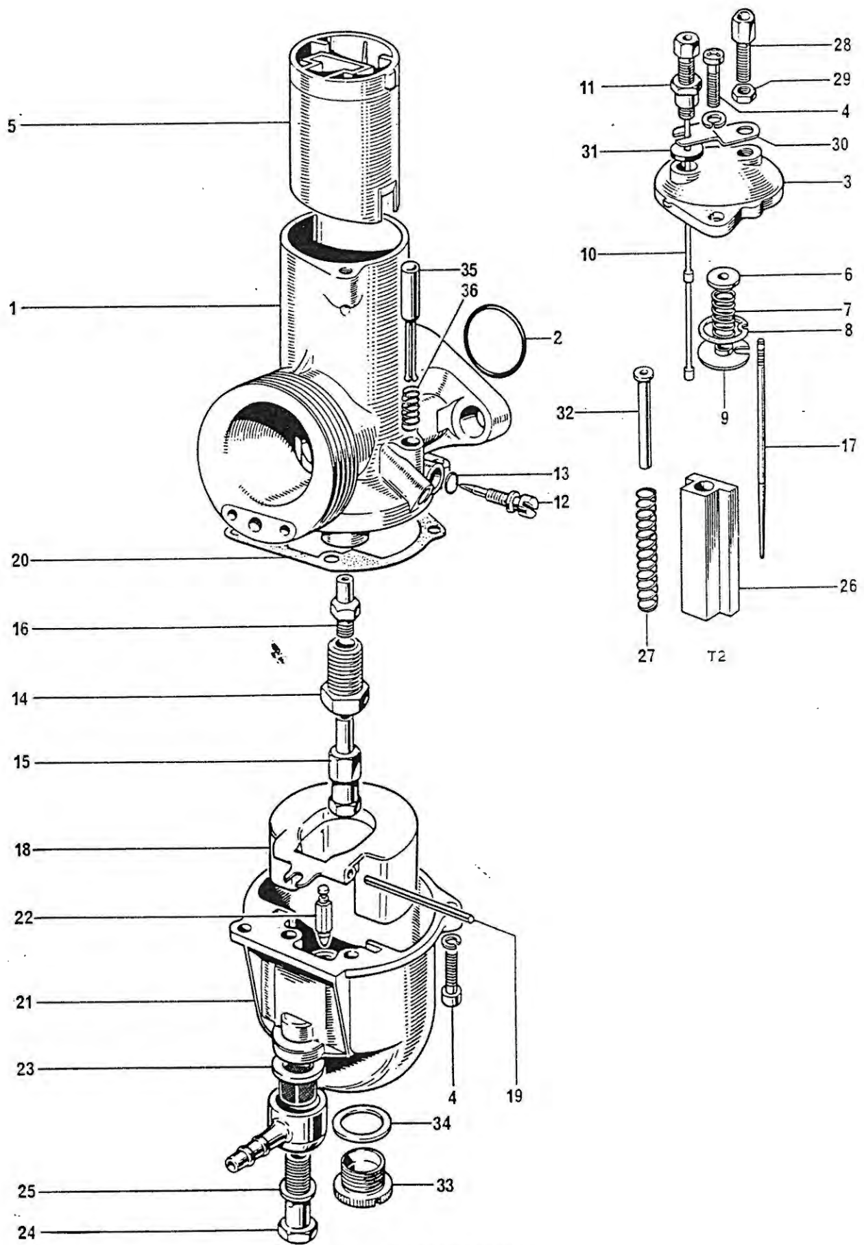
Fig. 5. CARBURETORS
