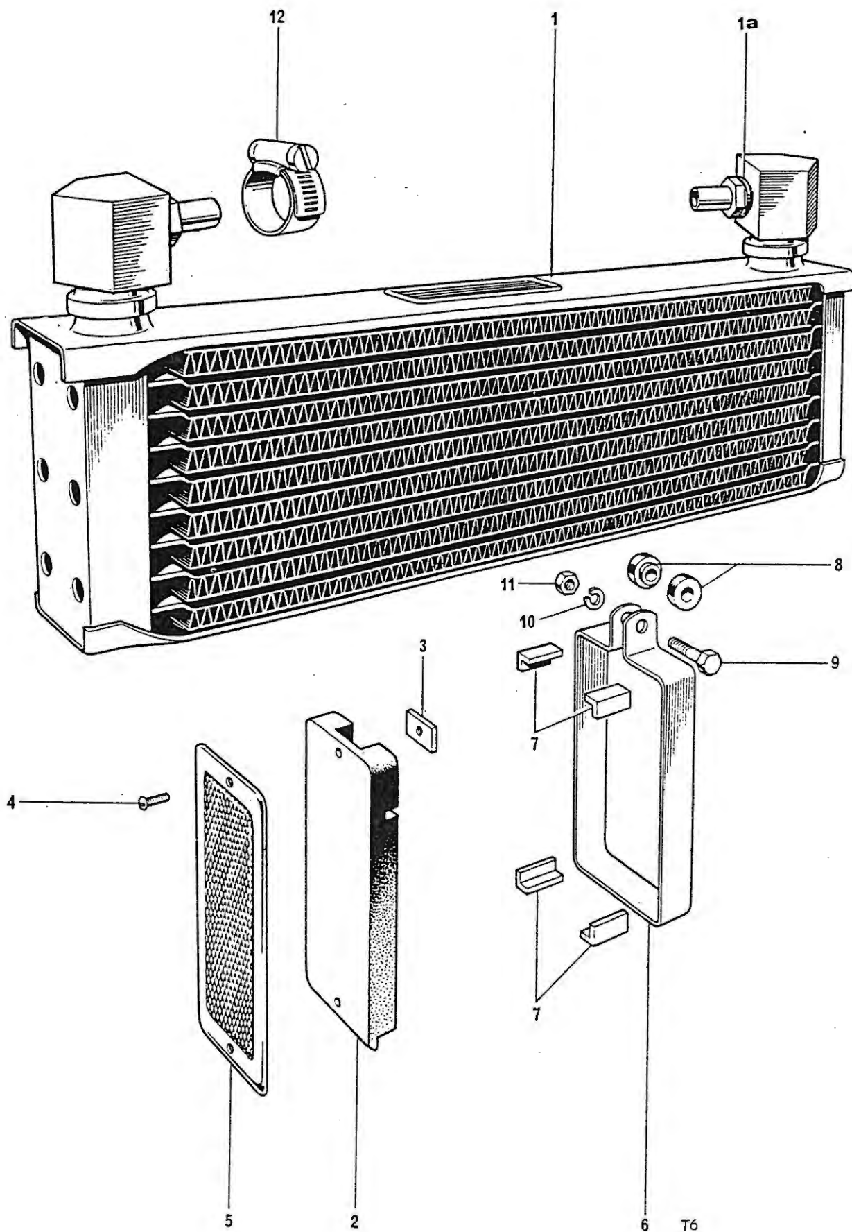
Fig. 24. OIL COOLER
