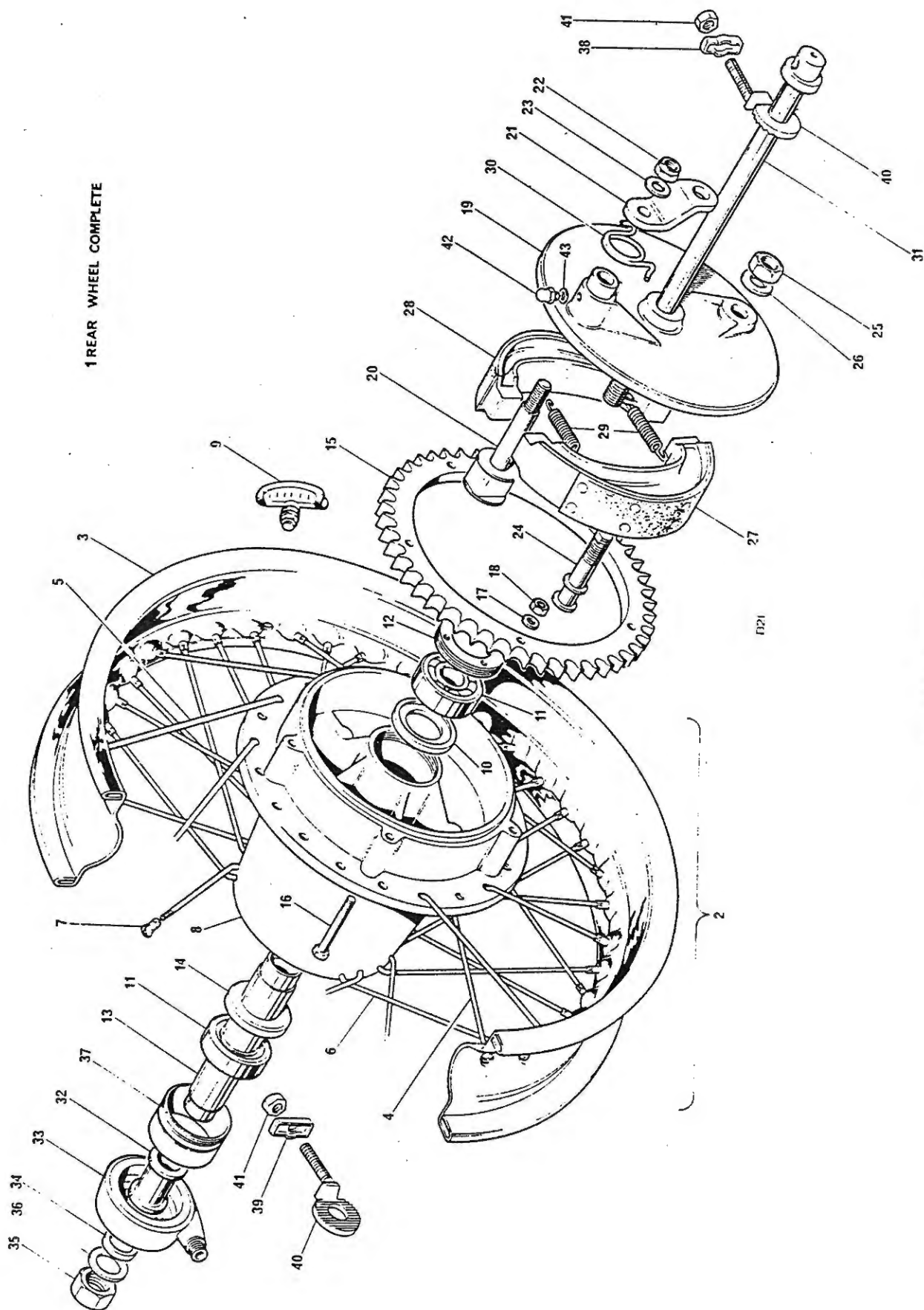
Fig. 23. REAR WHEEL
