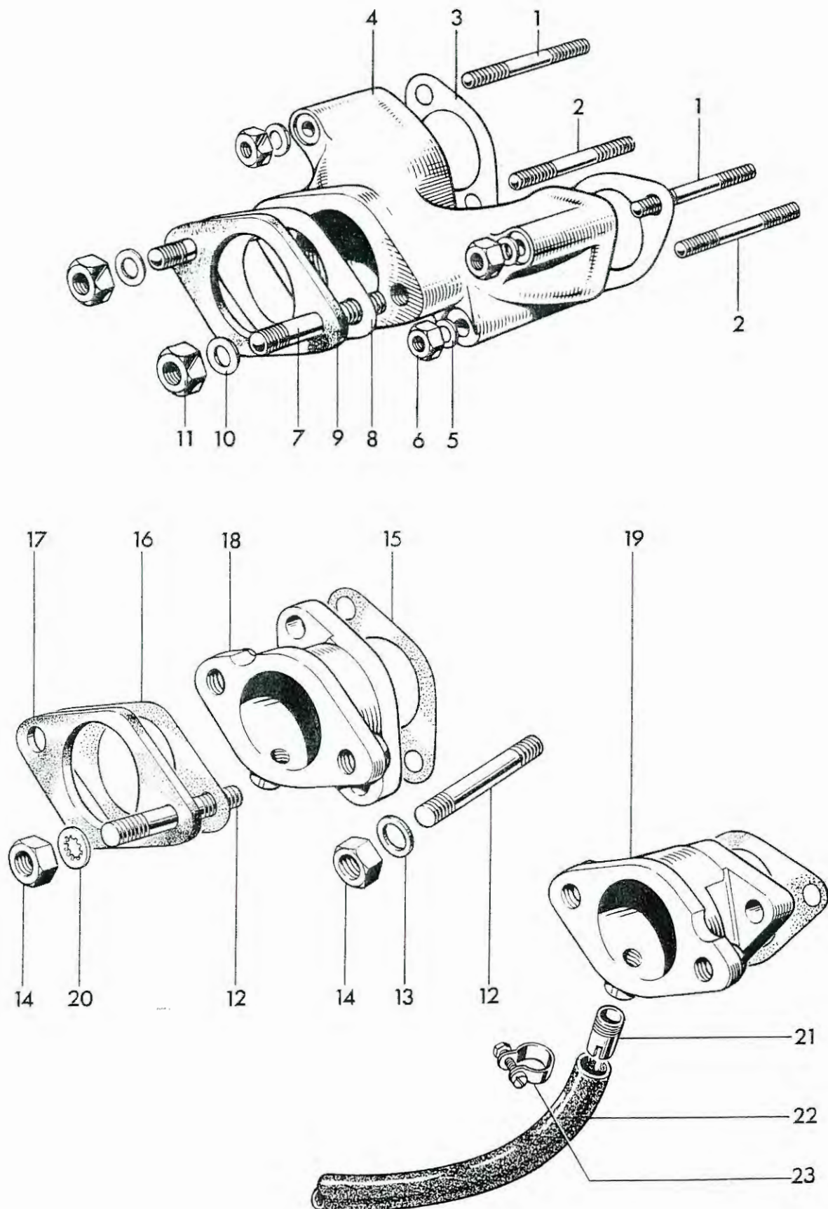
Fig. 4. INLET MANIFOLDS
