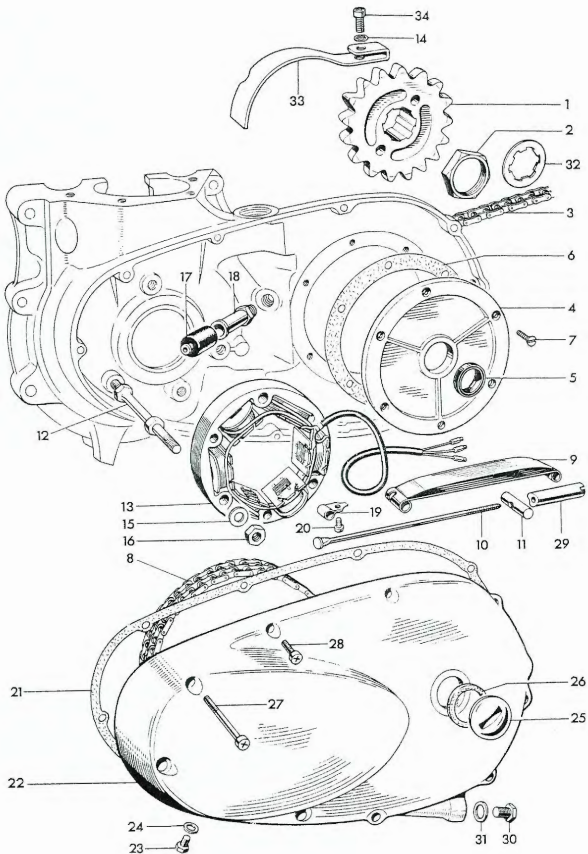
Fig. 12. CHAINCASE AND CHAINS
