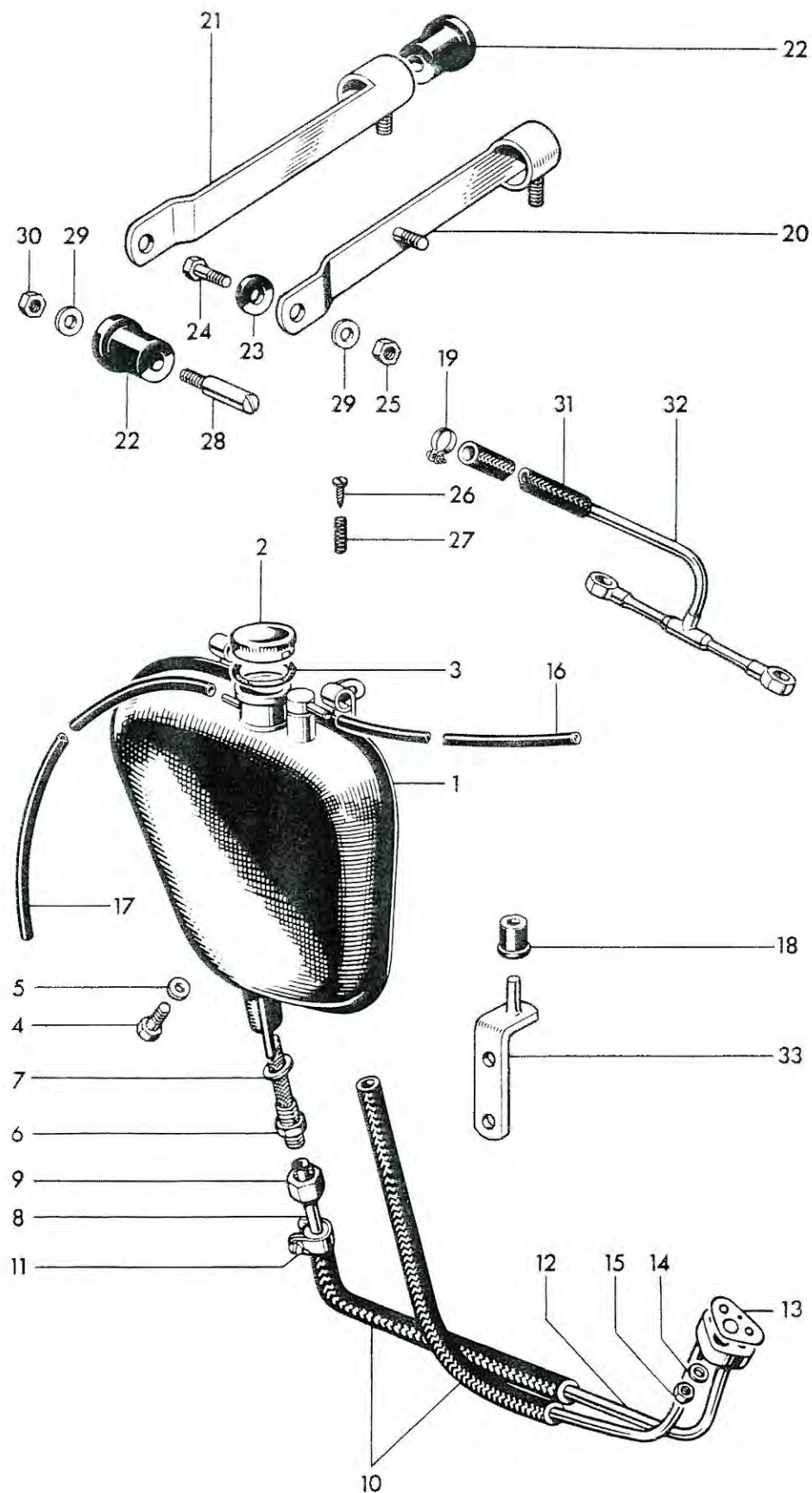
Fig. 25. OIL TANK
