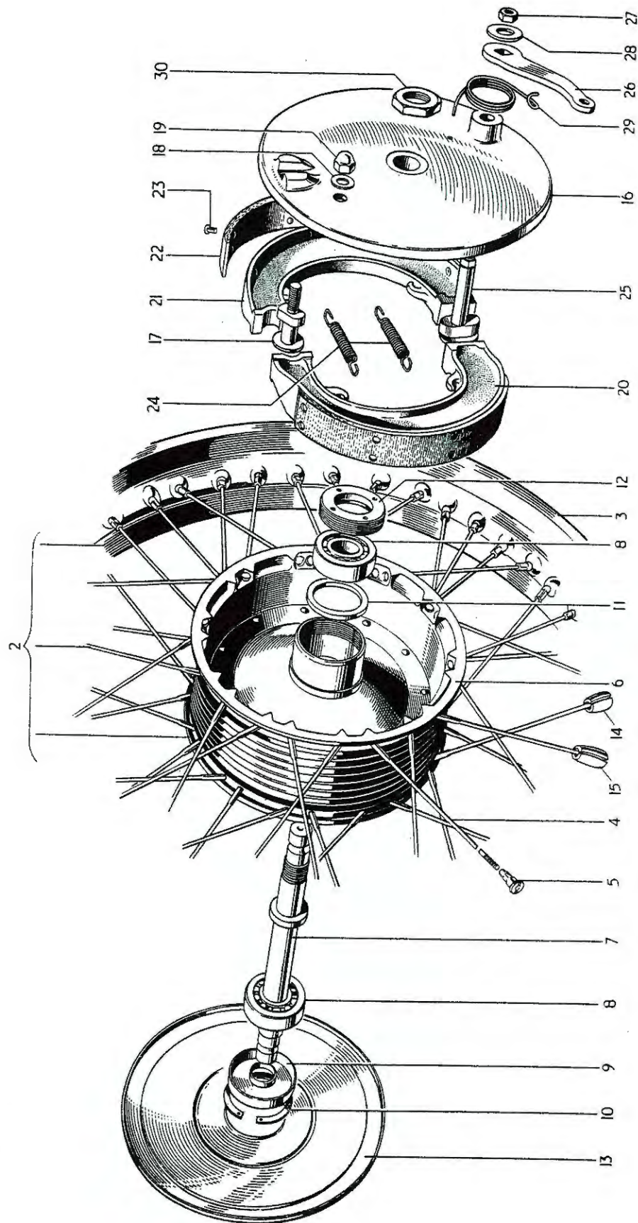
Fig. 15. FRONT WHEEL
