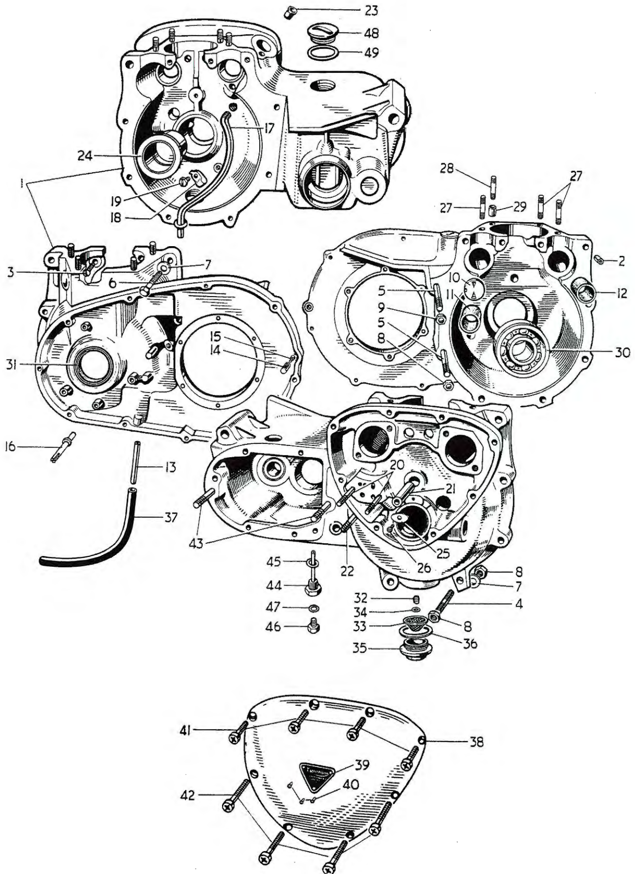
Fig 2. CRANKCASE
