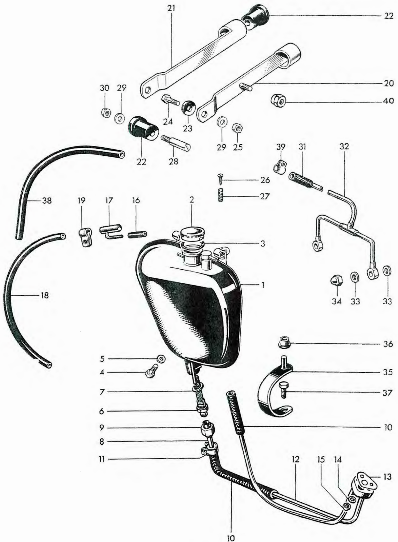
Fig. 23. OIL TANK
