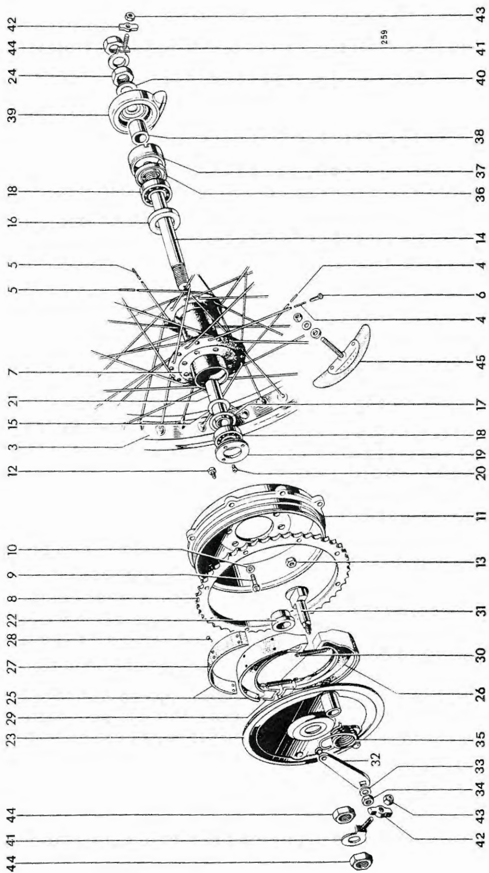
Fig. 20. REAR WHEEL
