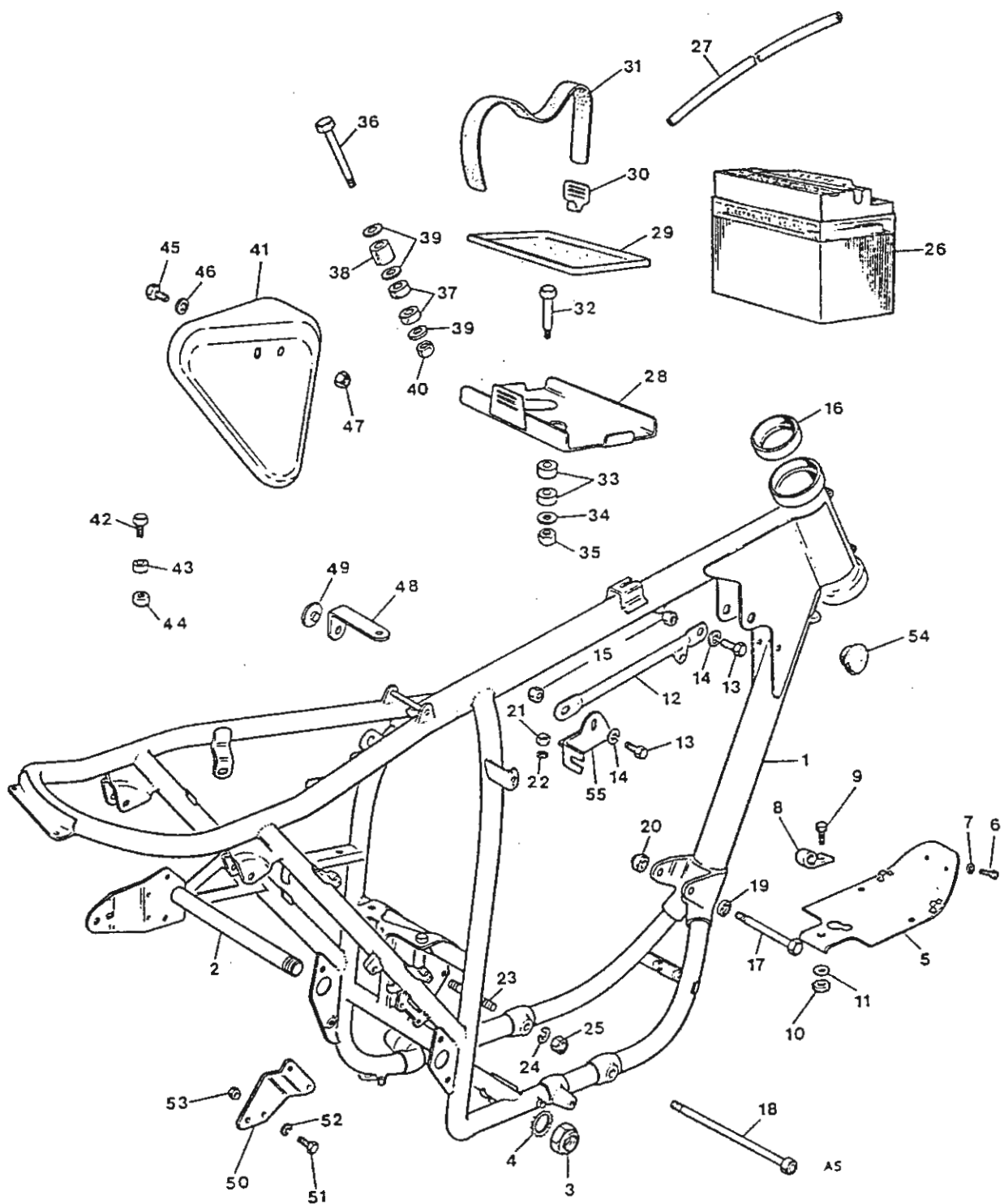
Fig. 5. FRAME COMPLETE
