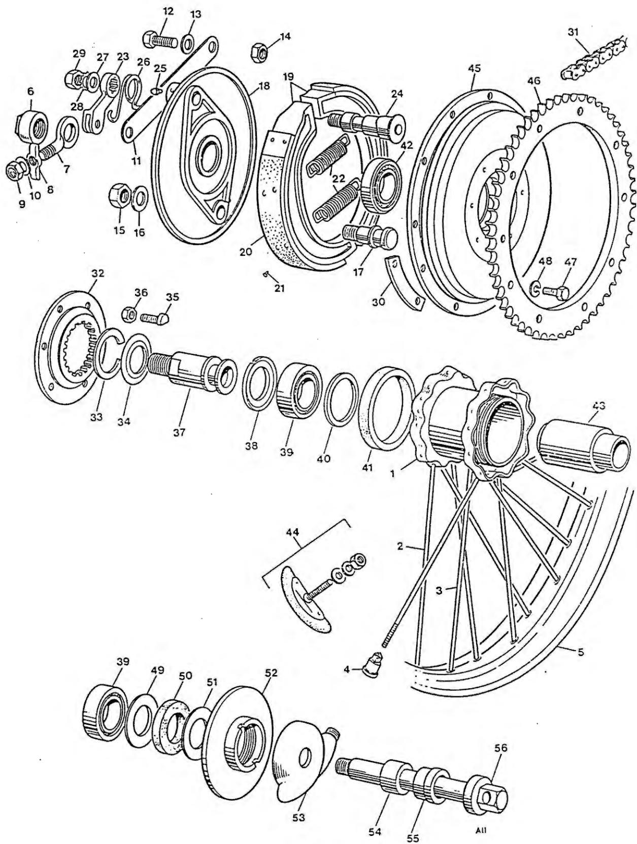
Fig. 11. REAR WHEEL
