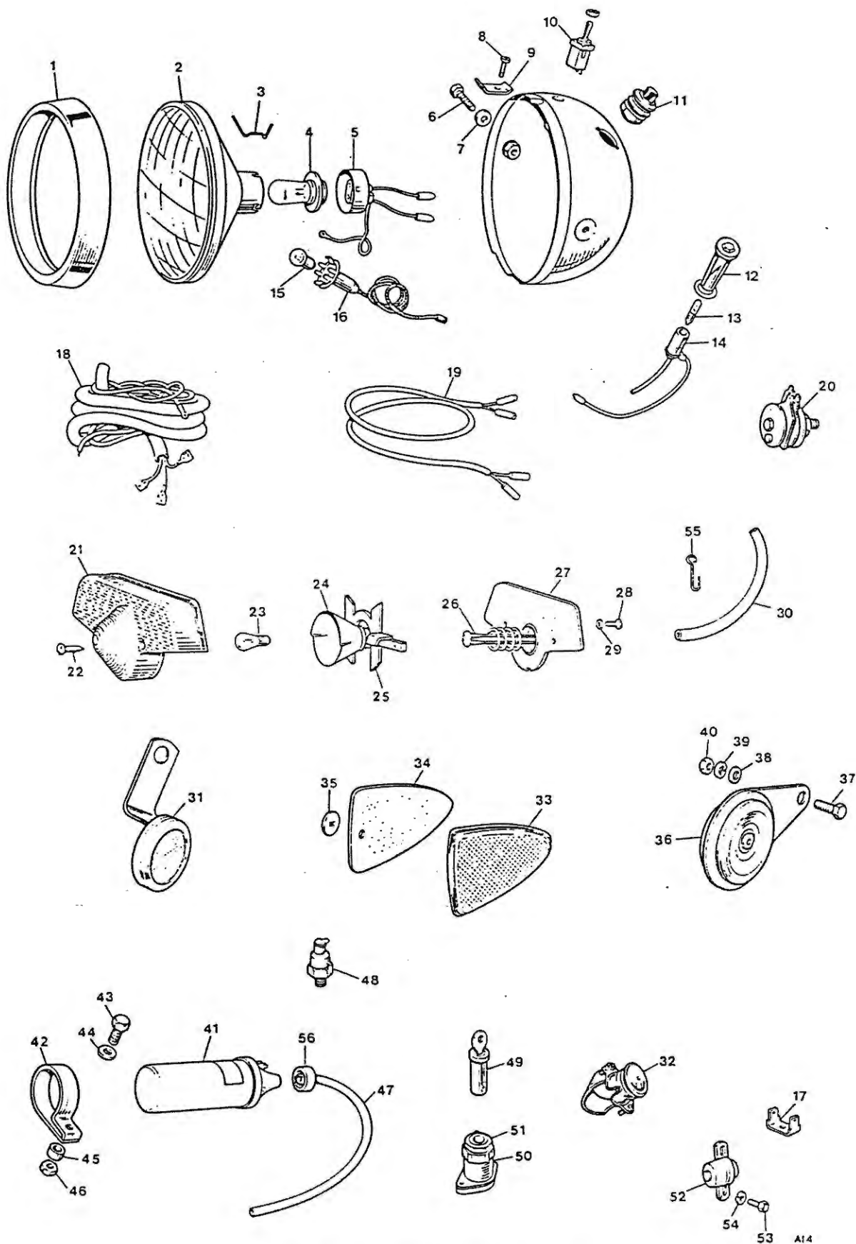
Fig. 16. ELECTRICAL EQUIPMENT
