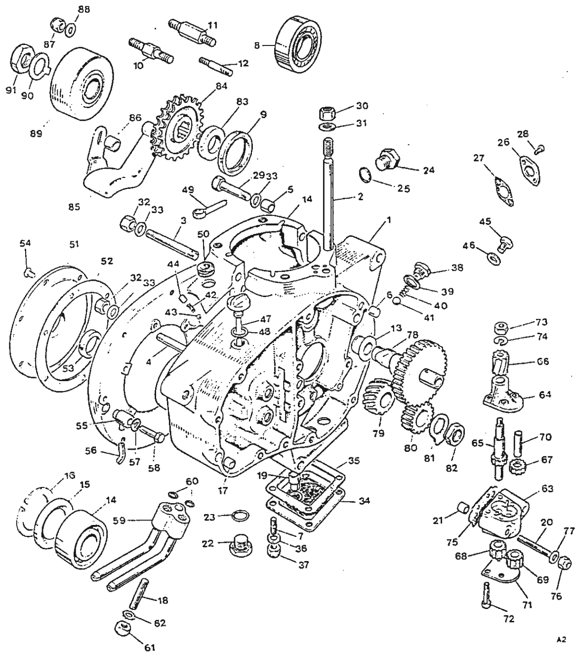
Fig. 2 CRANKCASE
