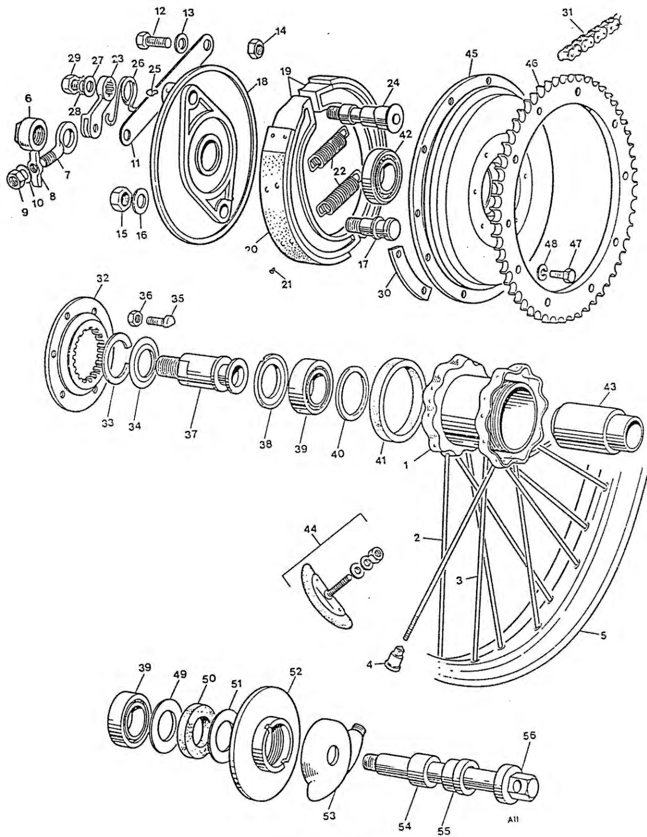
Fig. 11. REAR WHEEL
