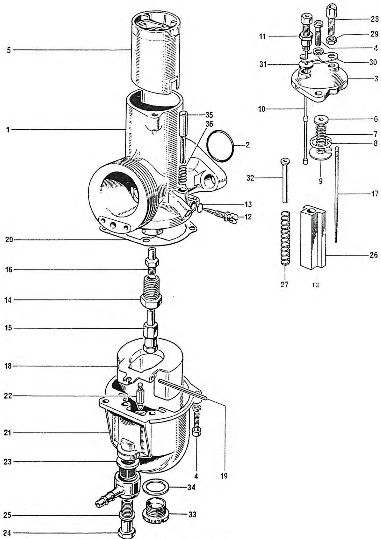
Fig. 5. CARBURETORS
