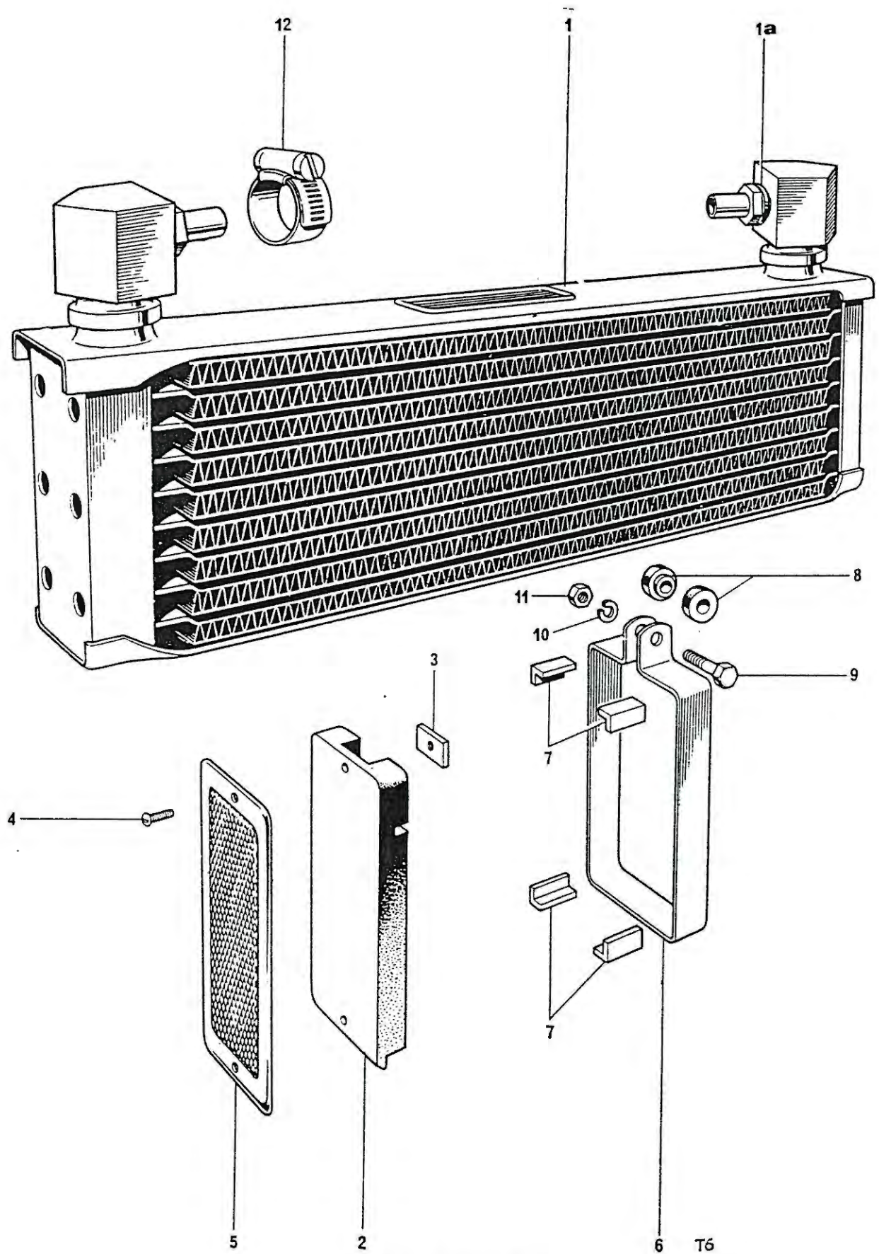
Fig. 24. OIL COOLER
