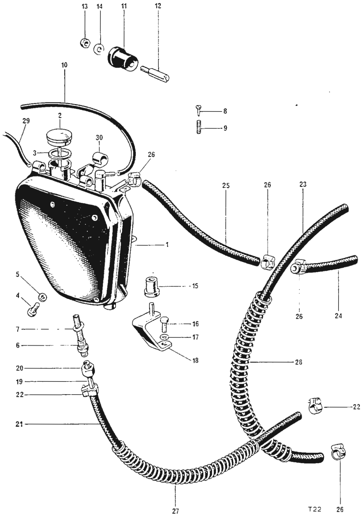
Fig. 26. OIL TANK
