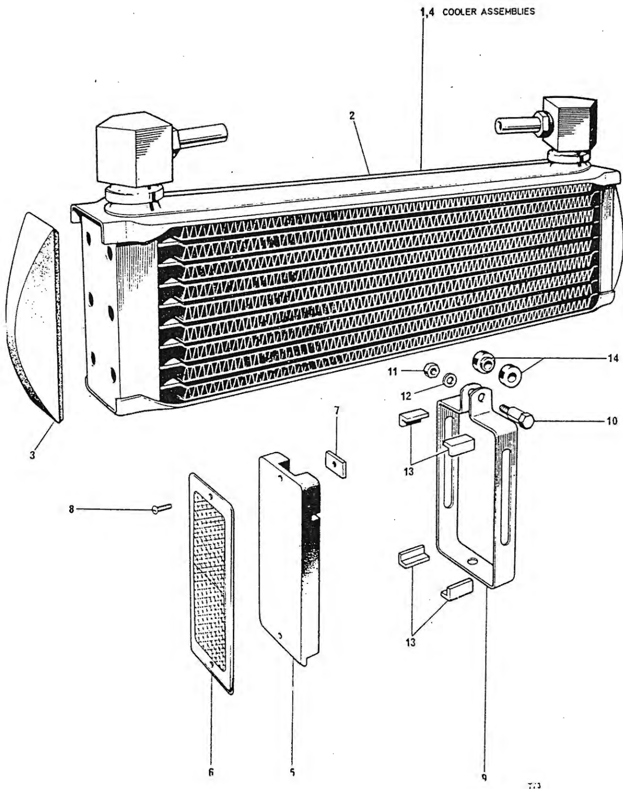
Fig. 26. OIL COOLER
