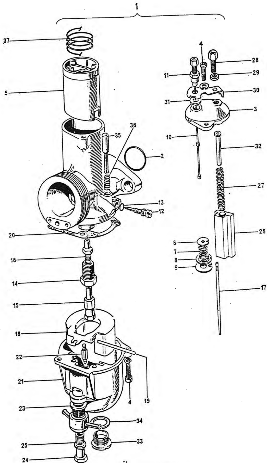
Fig. 5. CARBURETORS
