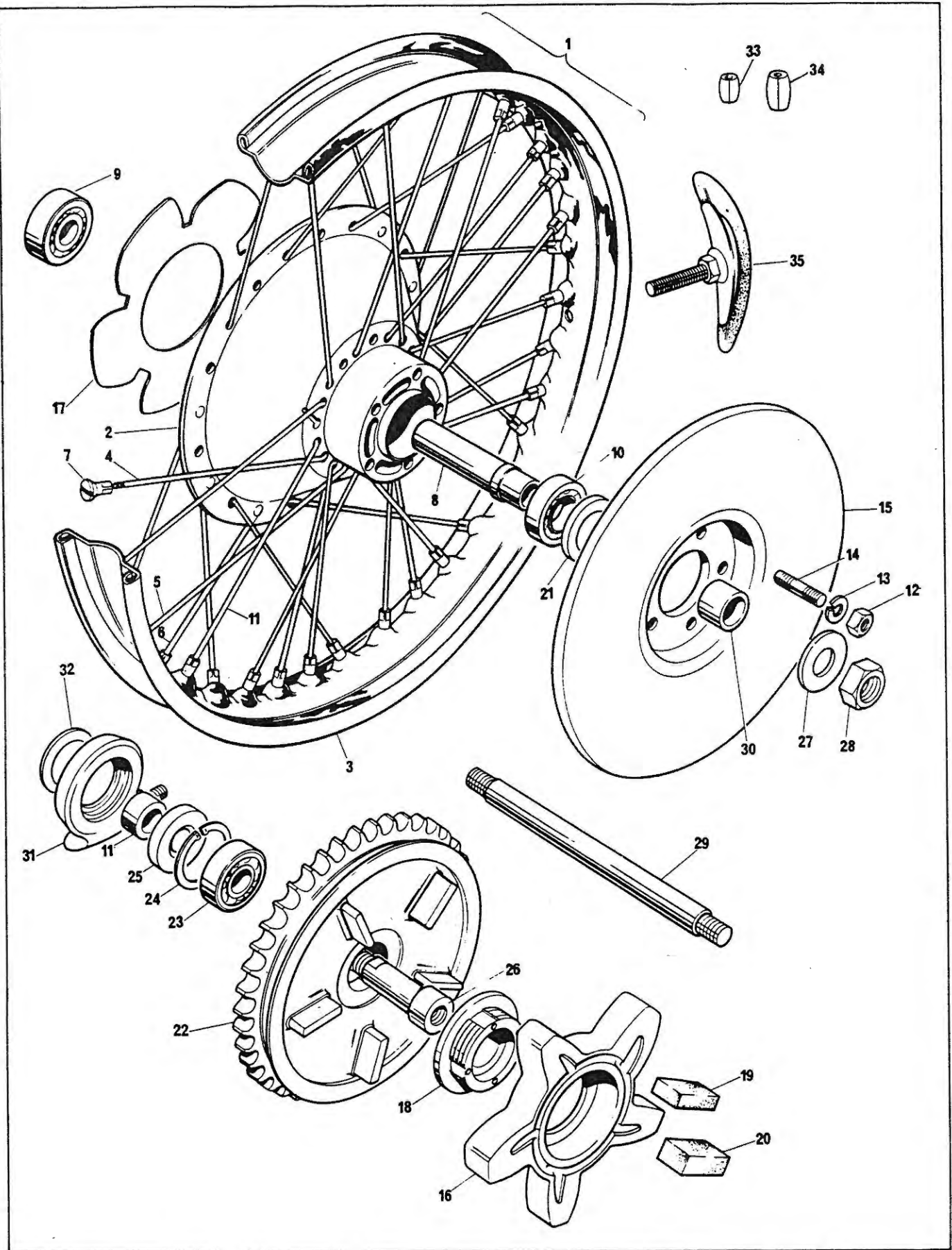
Rear Wheel : (Disc Type)
