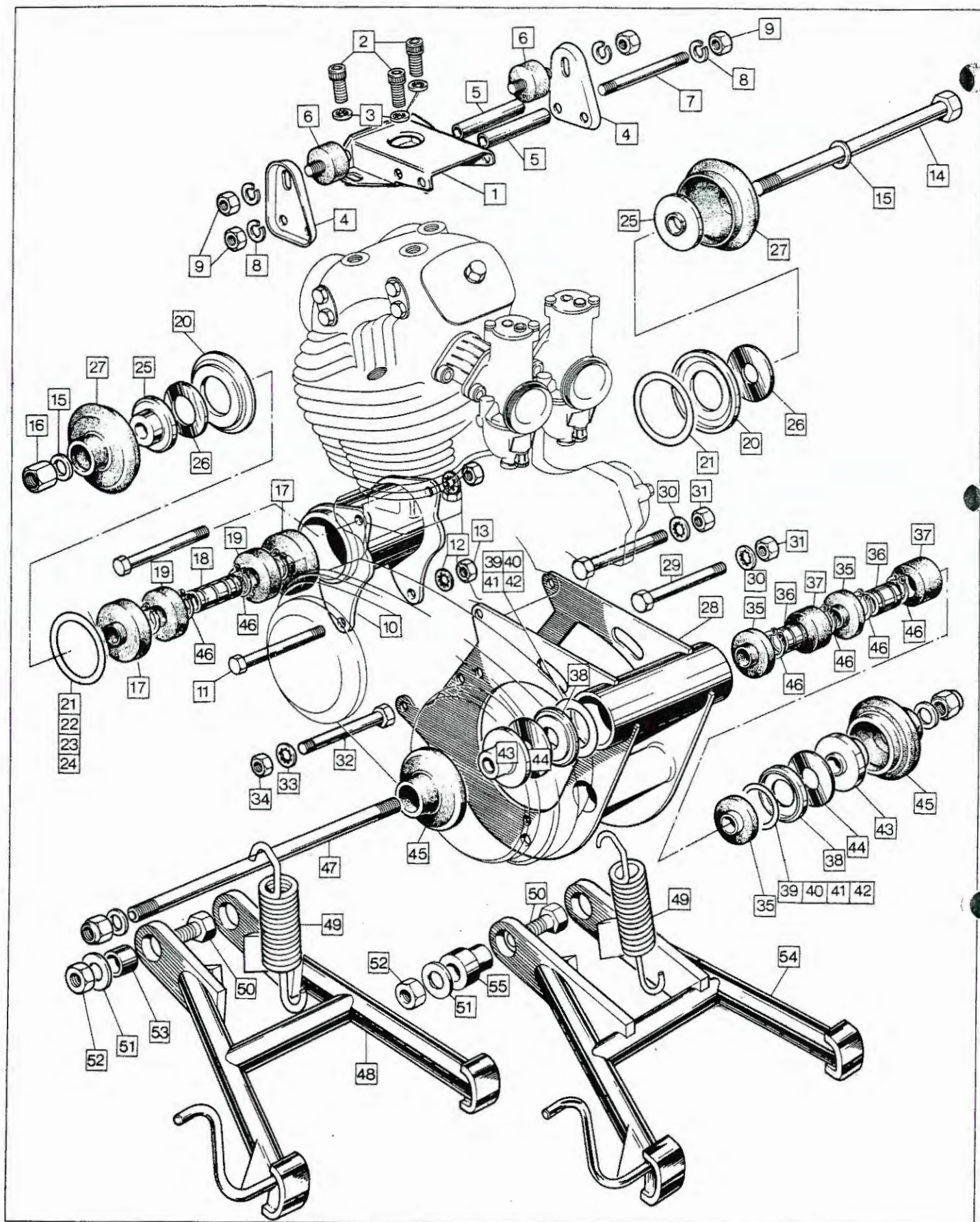
Engine Mountings, Head Steady, Centre Stand
