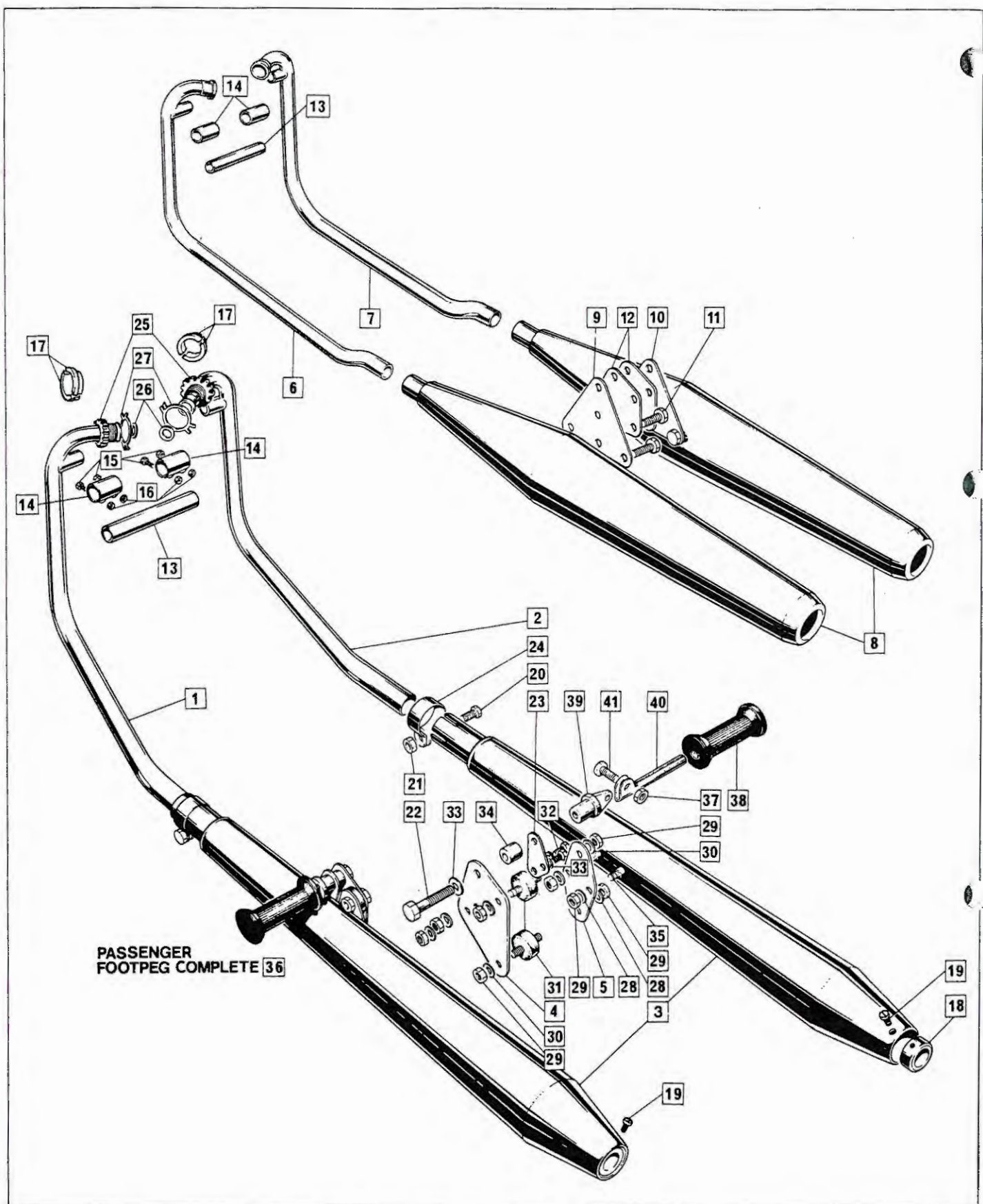
850 Exhausts, Mufflers, Mutes, Passenger Footpegs
