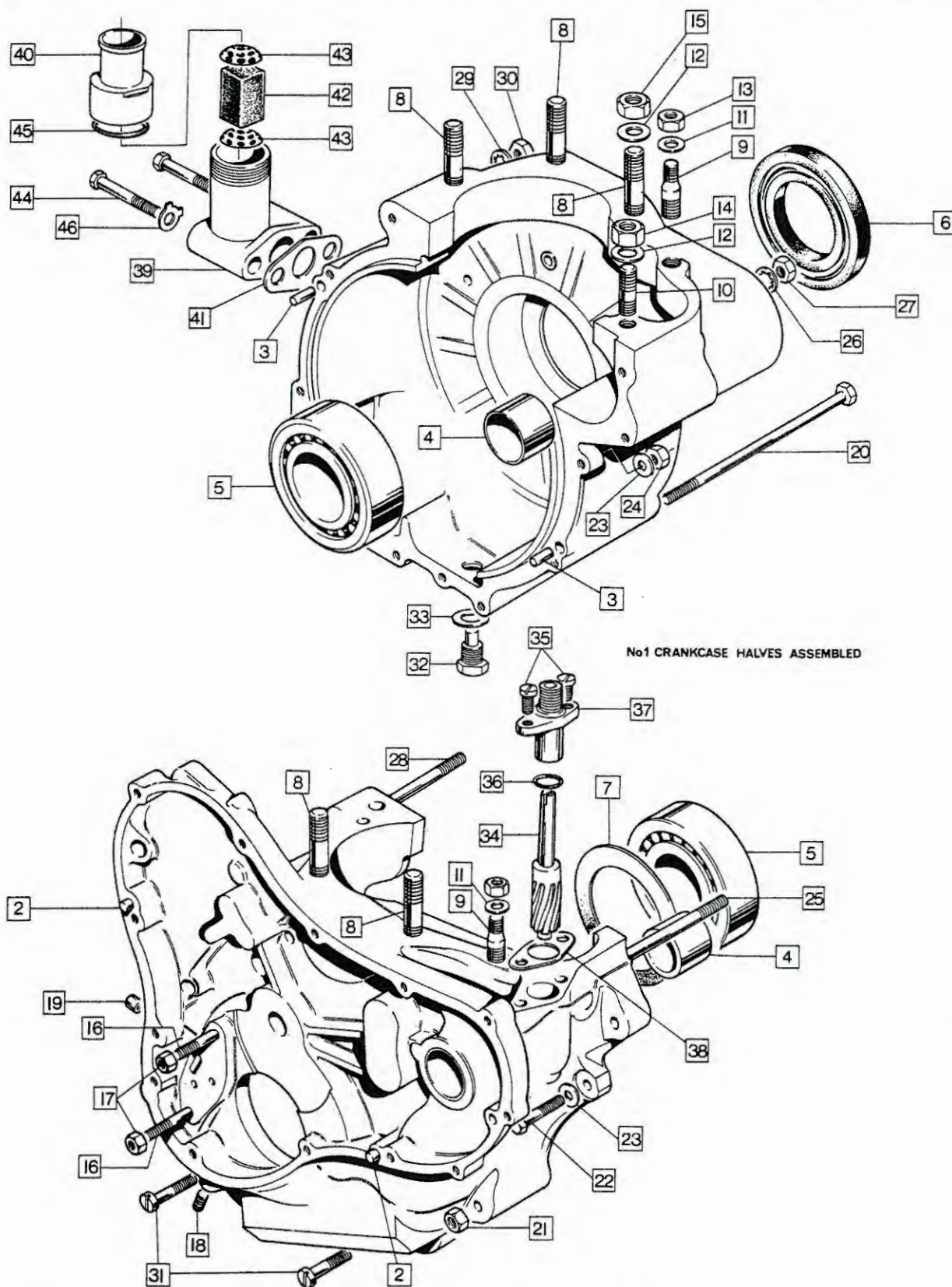
750 Engine: Crankcases, Crankcase Breather, Tachometer Drive
