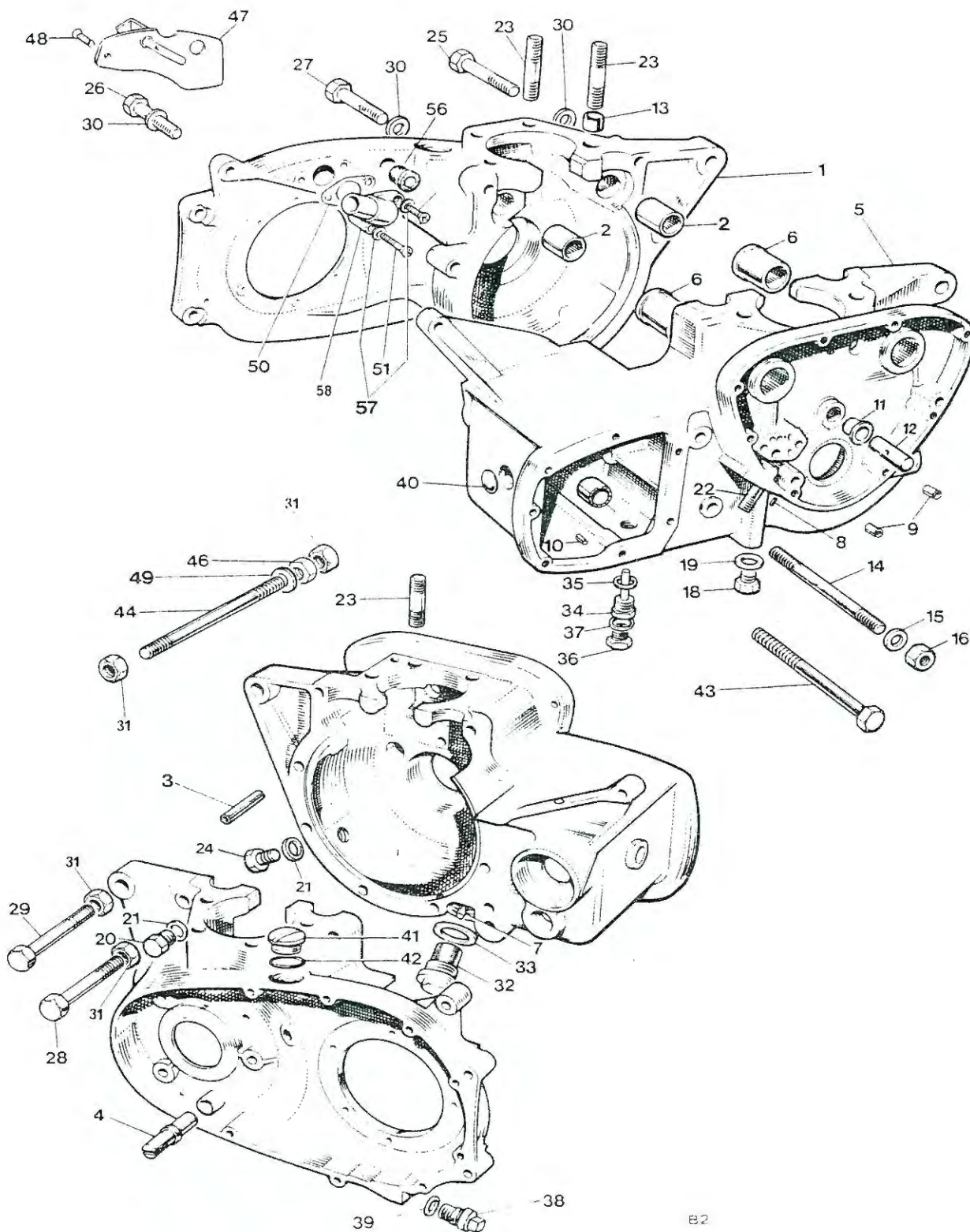
CRANKCASE
