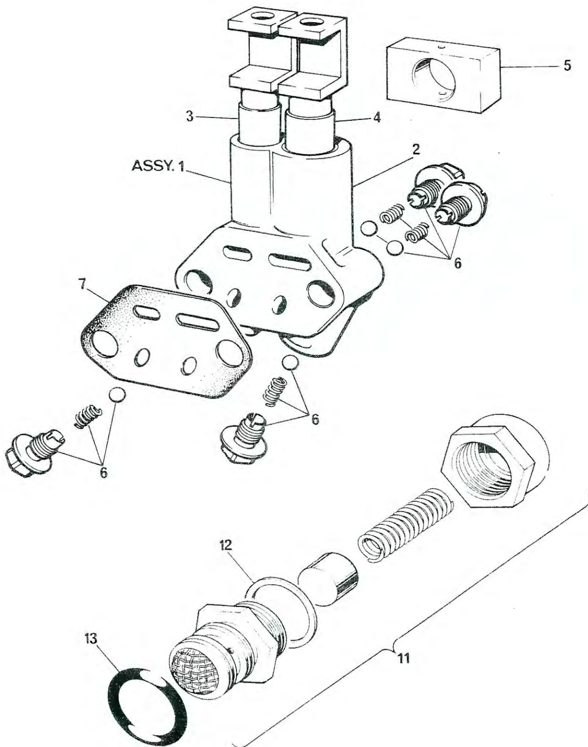
OIL PUMP AND RELEASE VALVE
