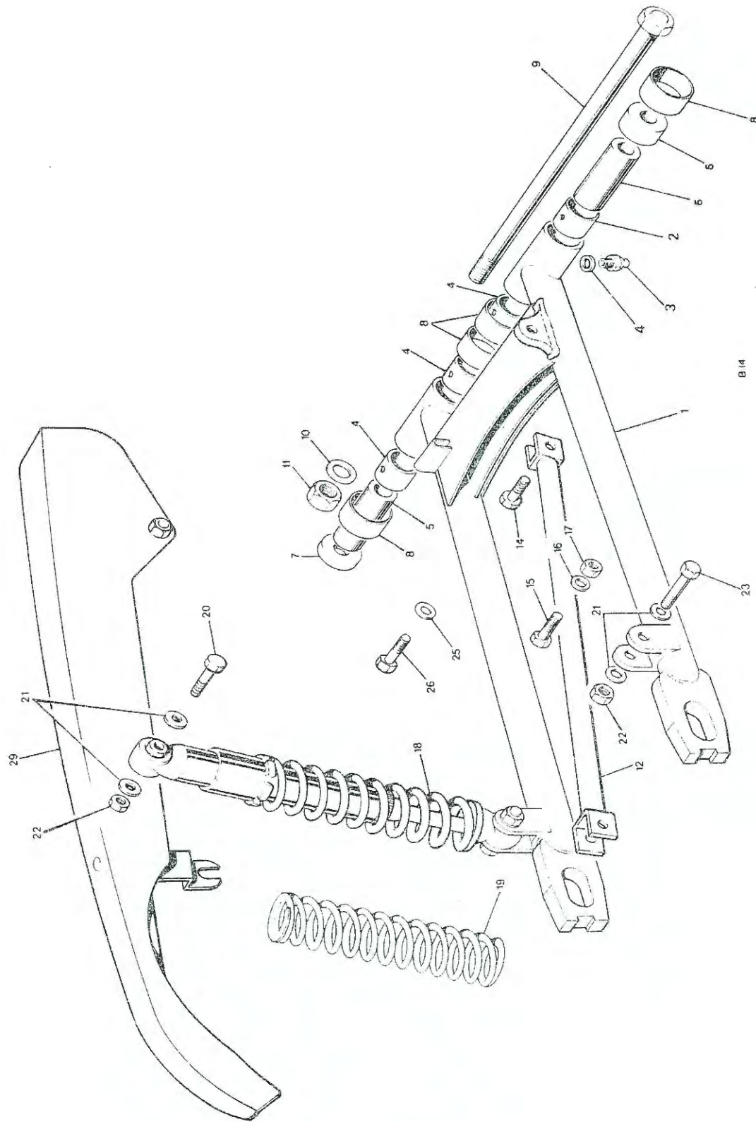
SWINGING ARM AND SUSPENSION UNITS
