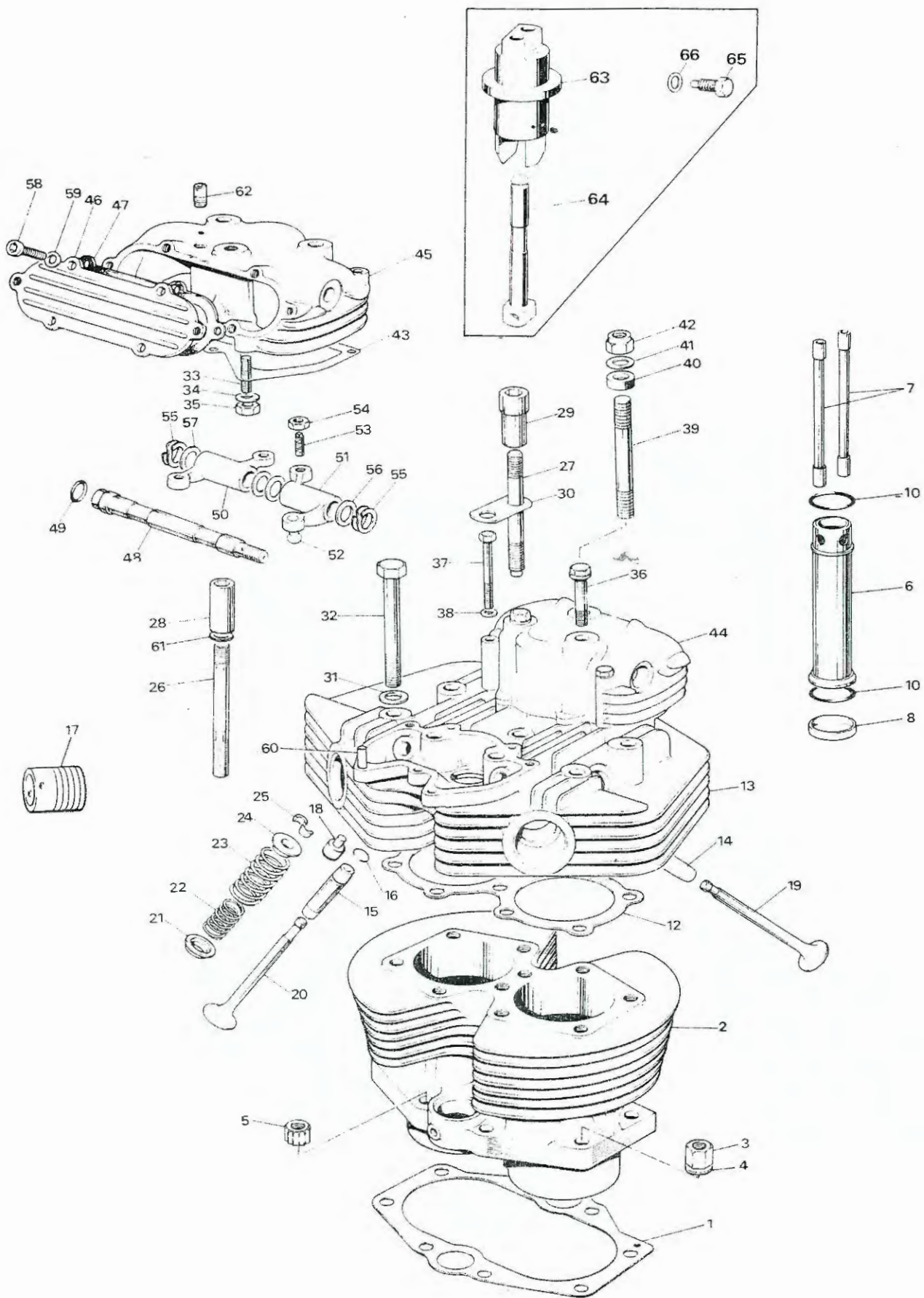
CYLINDER BLOCK AND HEAD
