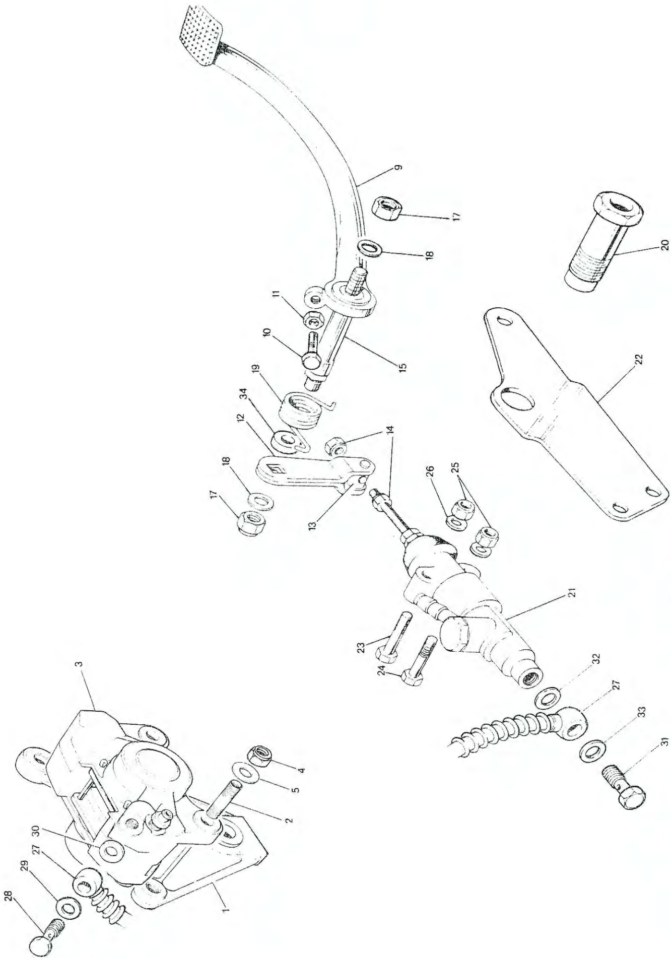
REAR BRAKE
