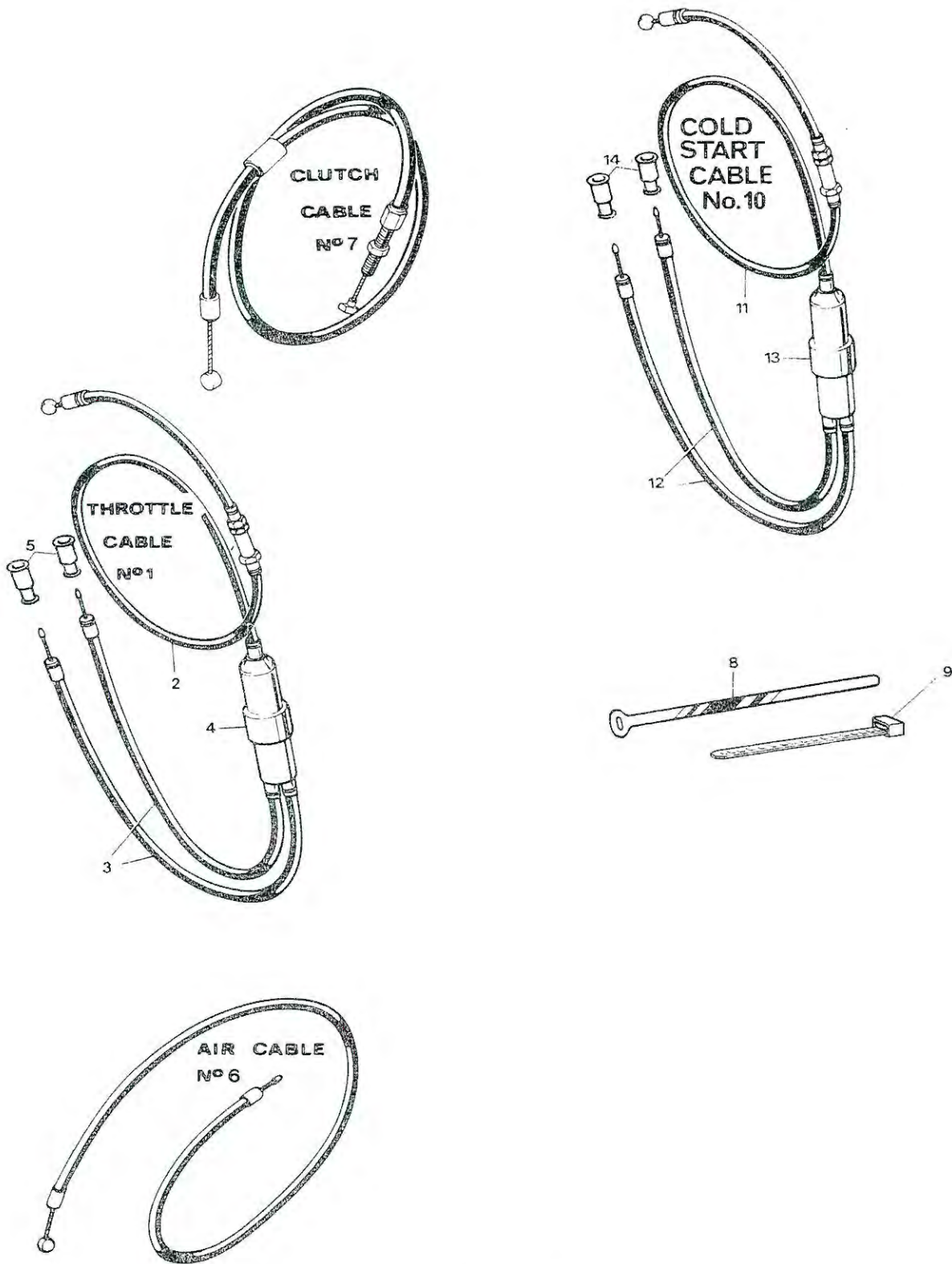
CONTROL CABLES
