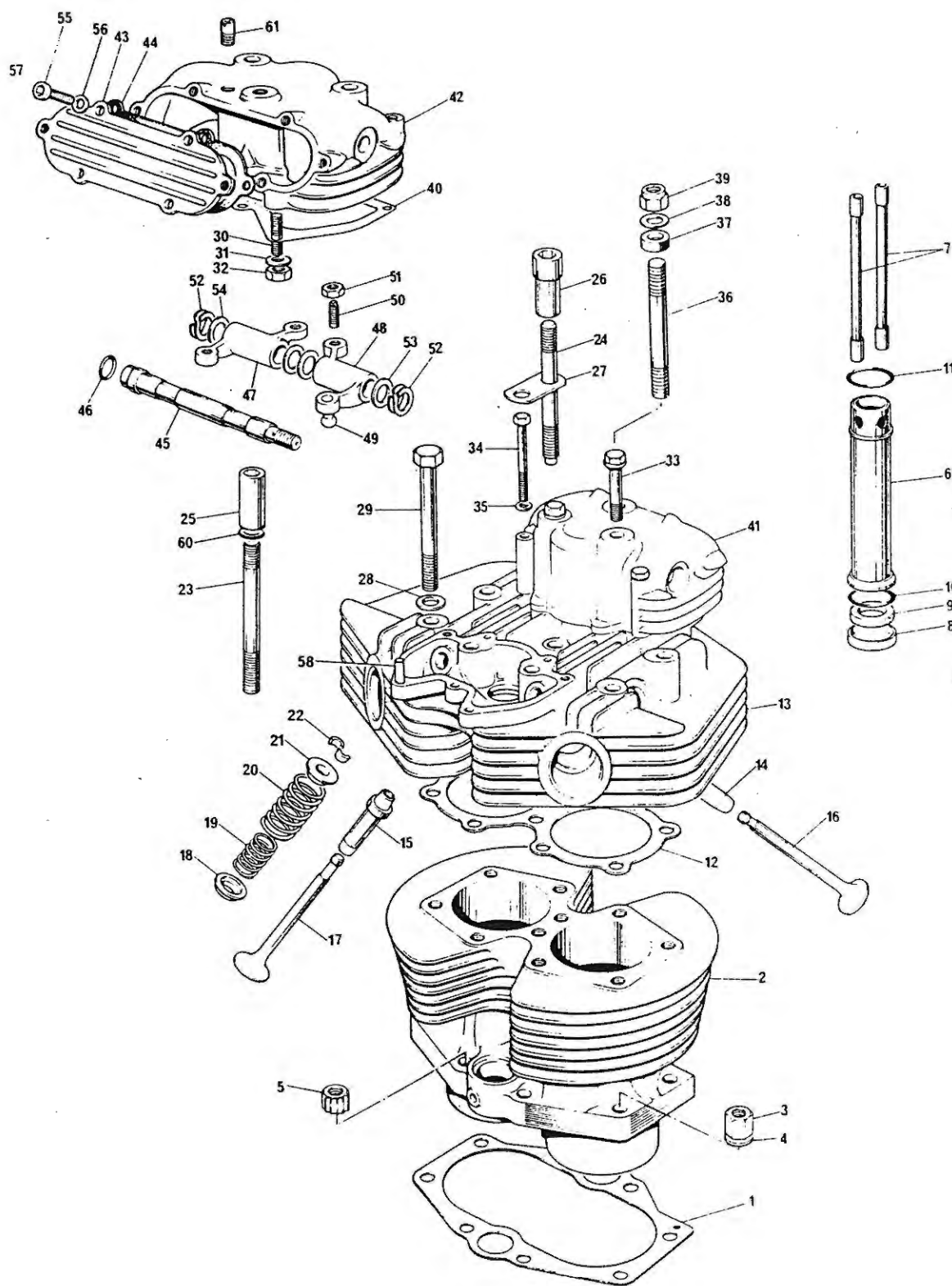
CYLINDER BLOCK & HEAD, TR7
