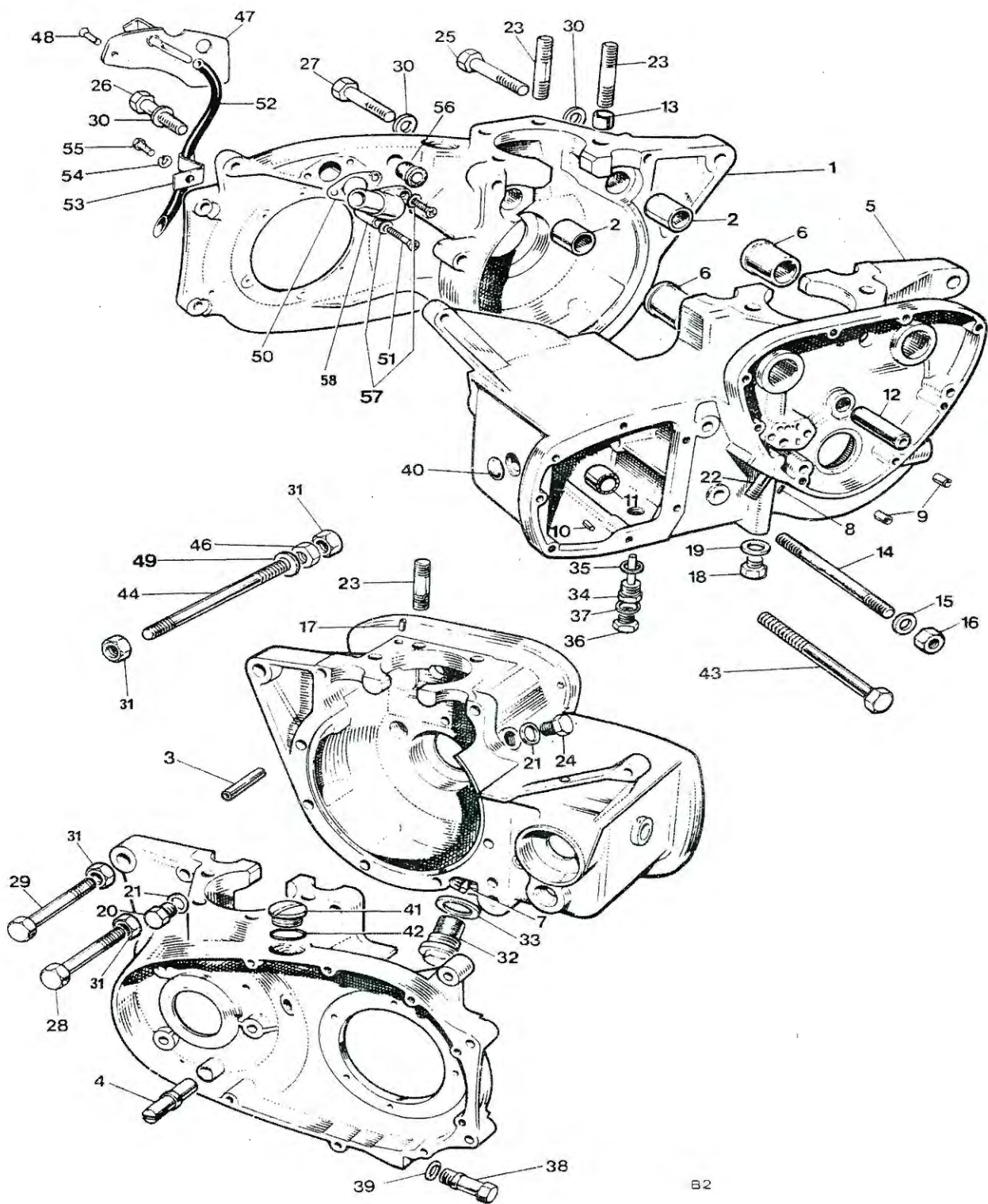
Fig. 2 CRANKCASE
