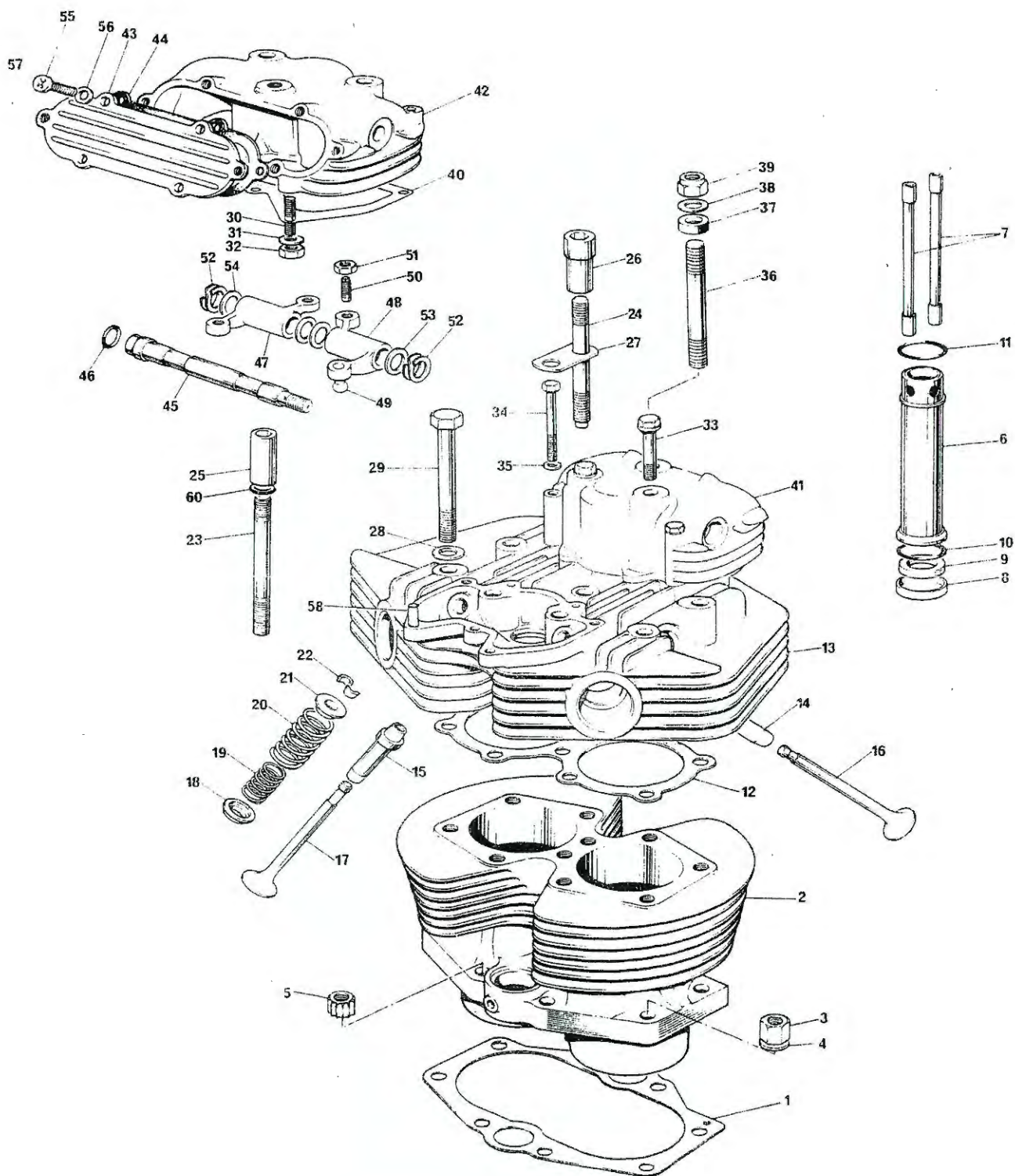
CYLINDER BLOCK & HEAD, T140V
