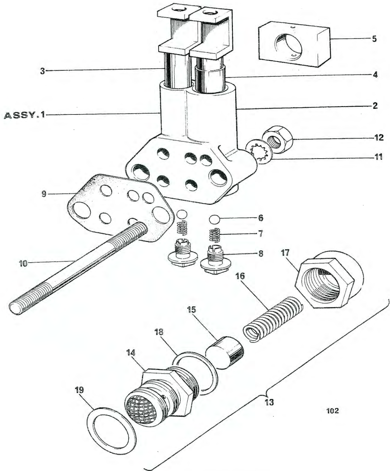
Fig. 3. OIL PUMP AND RELEASE VALVE
