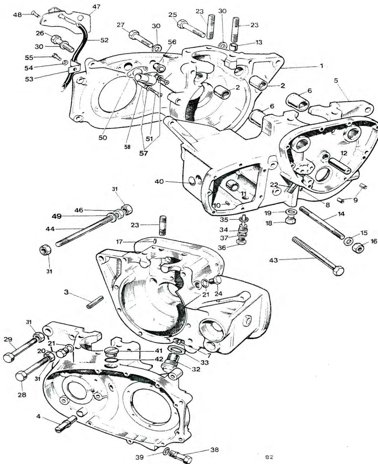
Fig. 2 CRANKCASE
