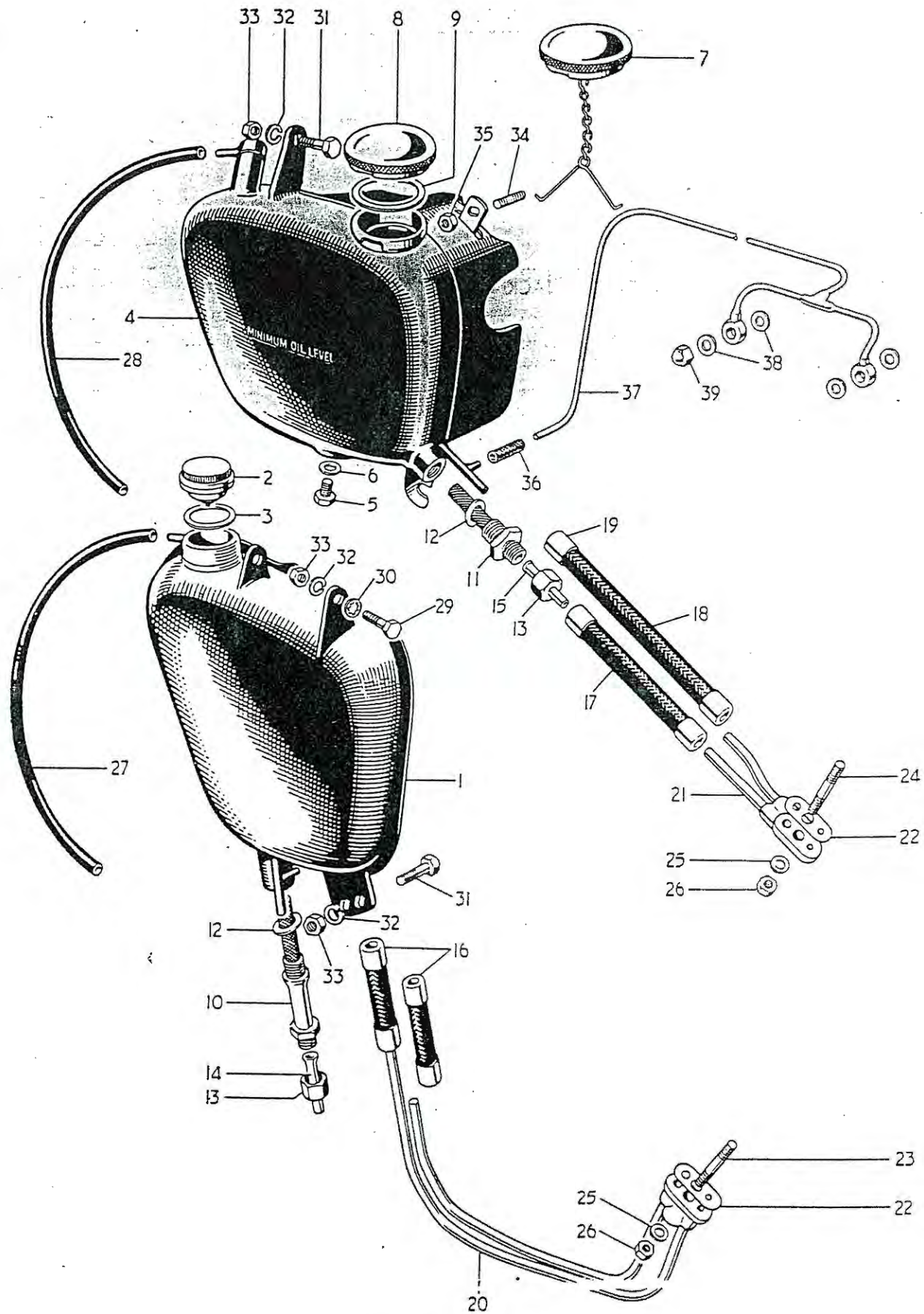
FIG. 24 OIL TANKS
