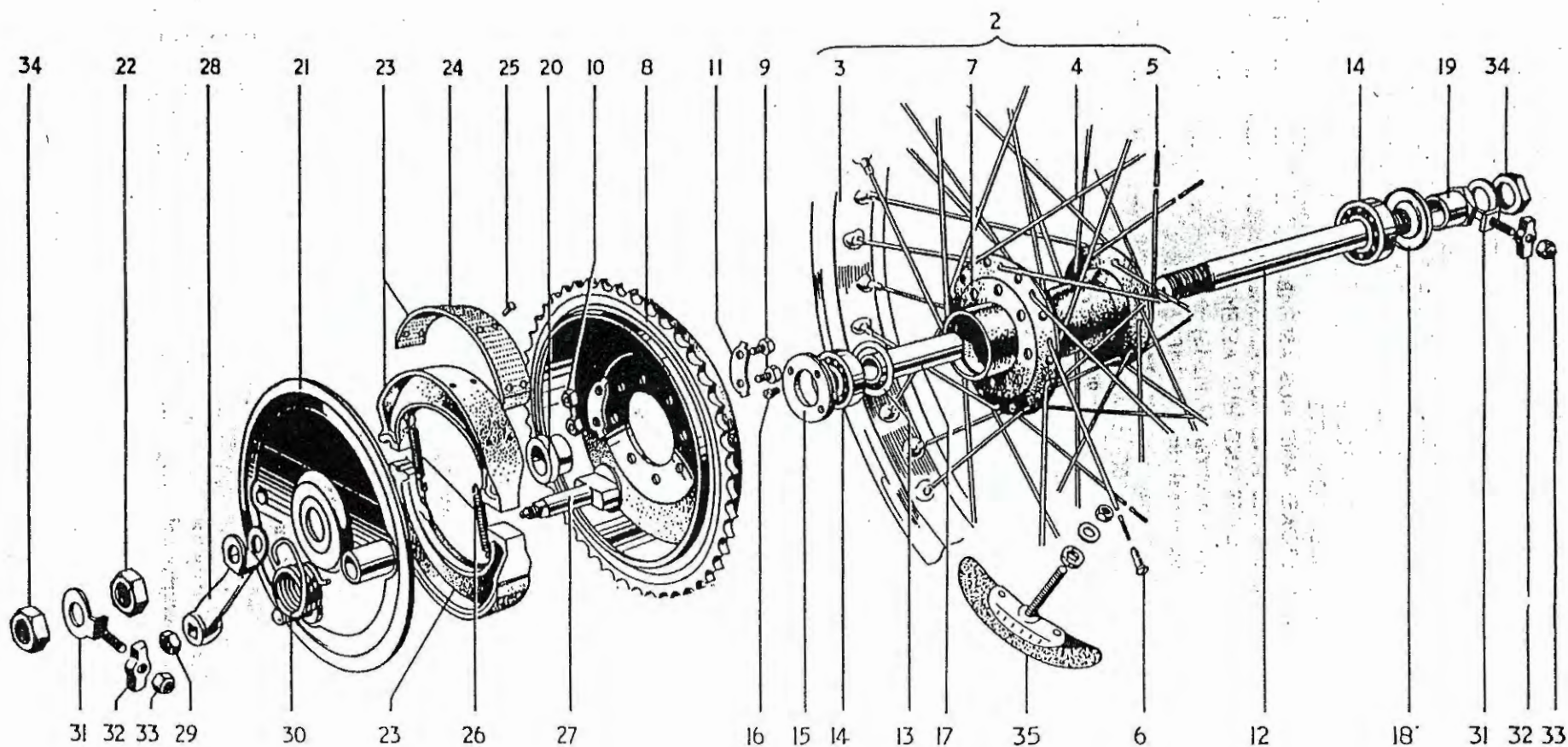
FIG. 21 REAR WHEEL
