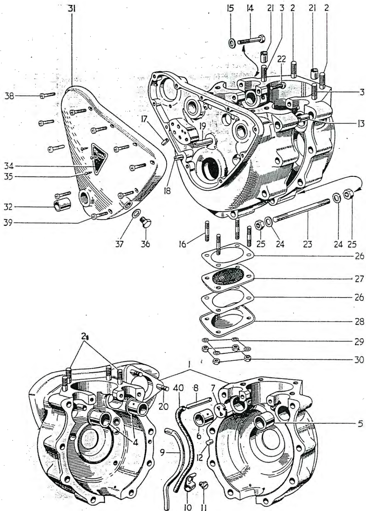
FIG. 2 CRANKCASE
