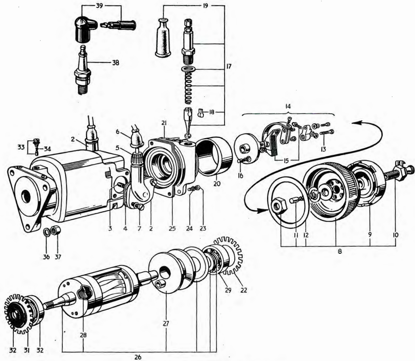
FIG. 35 MAGNETO WITH MANUAL CONTROL
