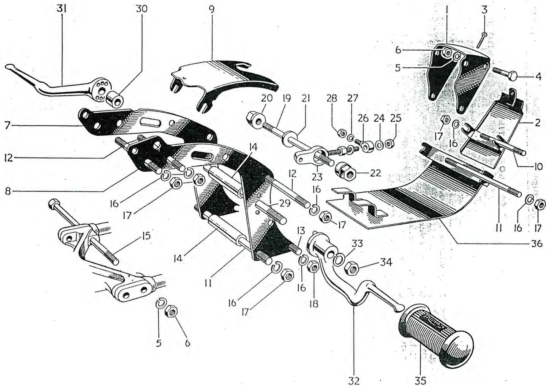
FIG. 13 ENGINE AND GEARBOX FITTINGS
