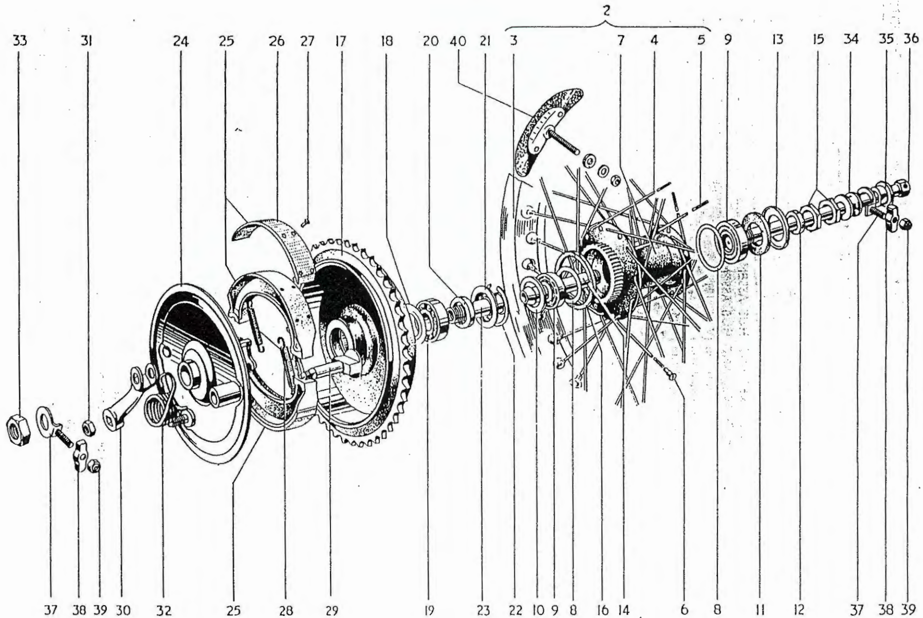
FIG. 22 QUICKLY DETACHABLE REAR WHEEL
