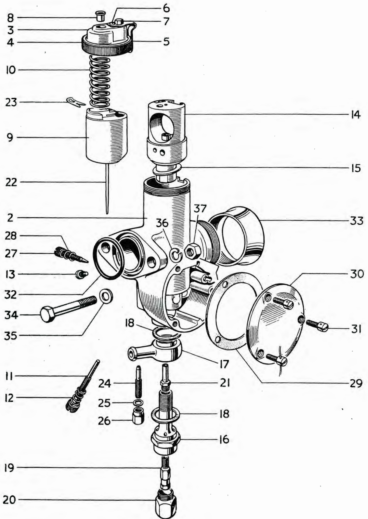
FIG. 32 BONNEVILLE 120 CARBURETTERS
