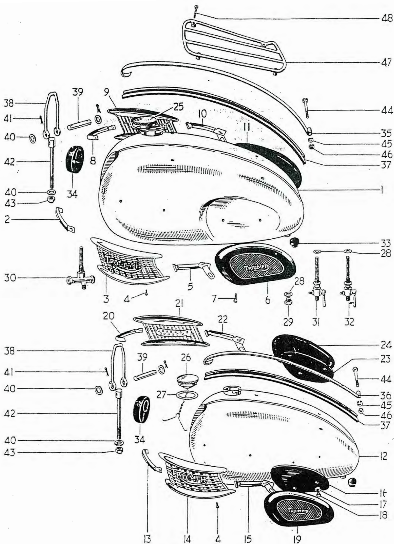
FIG. 23 PETROL TANKS
