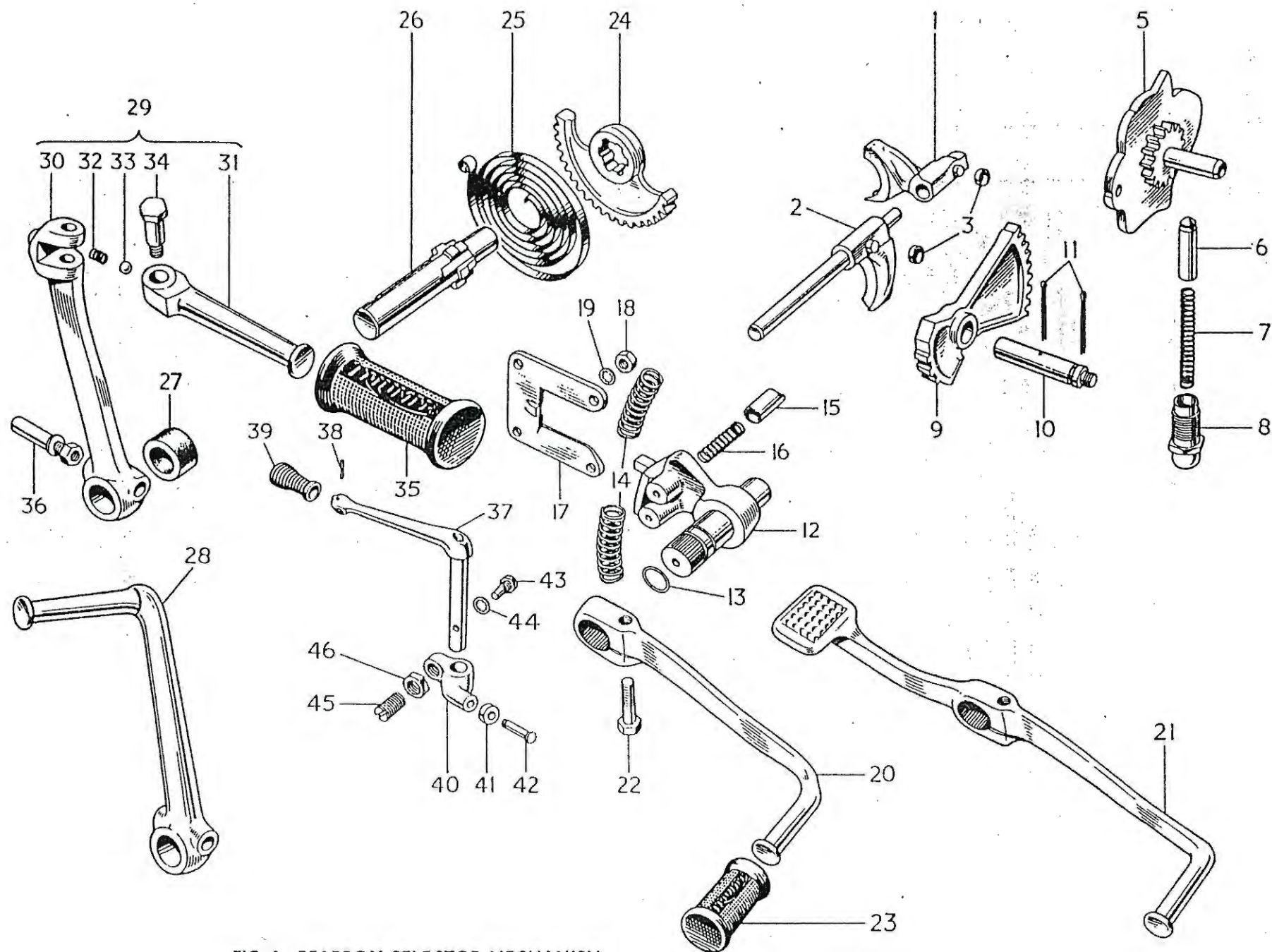
FIG. 9 GEARBOX SELECTOR MECHANISM
