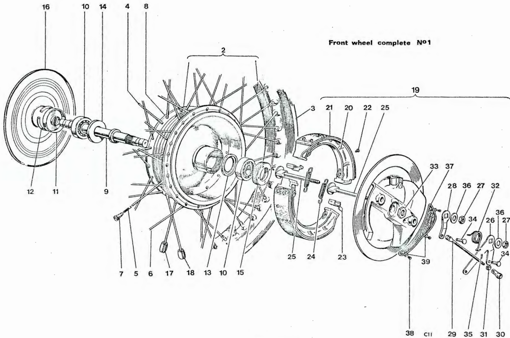
Fig. 17. FRONT WHEEL
