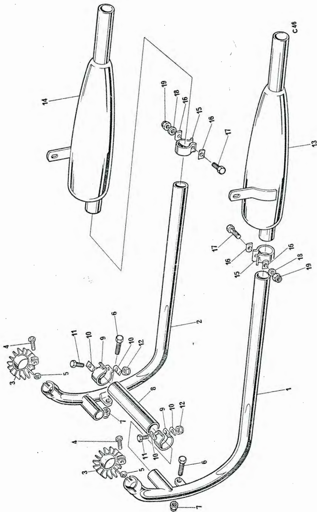
Fig. 12. EXHAUST SYSTEM
