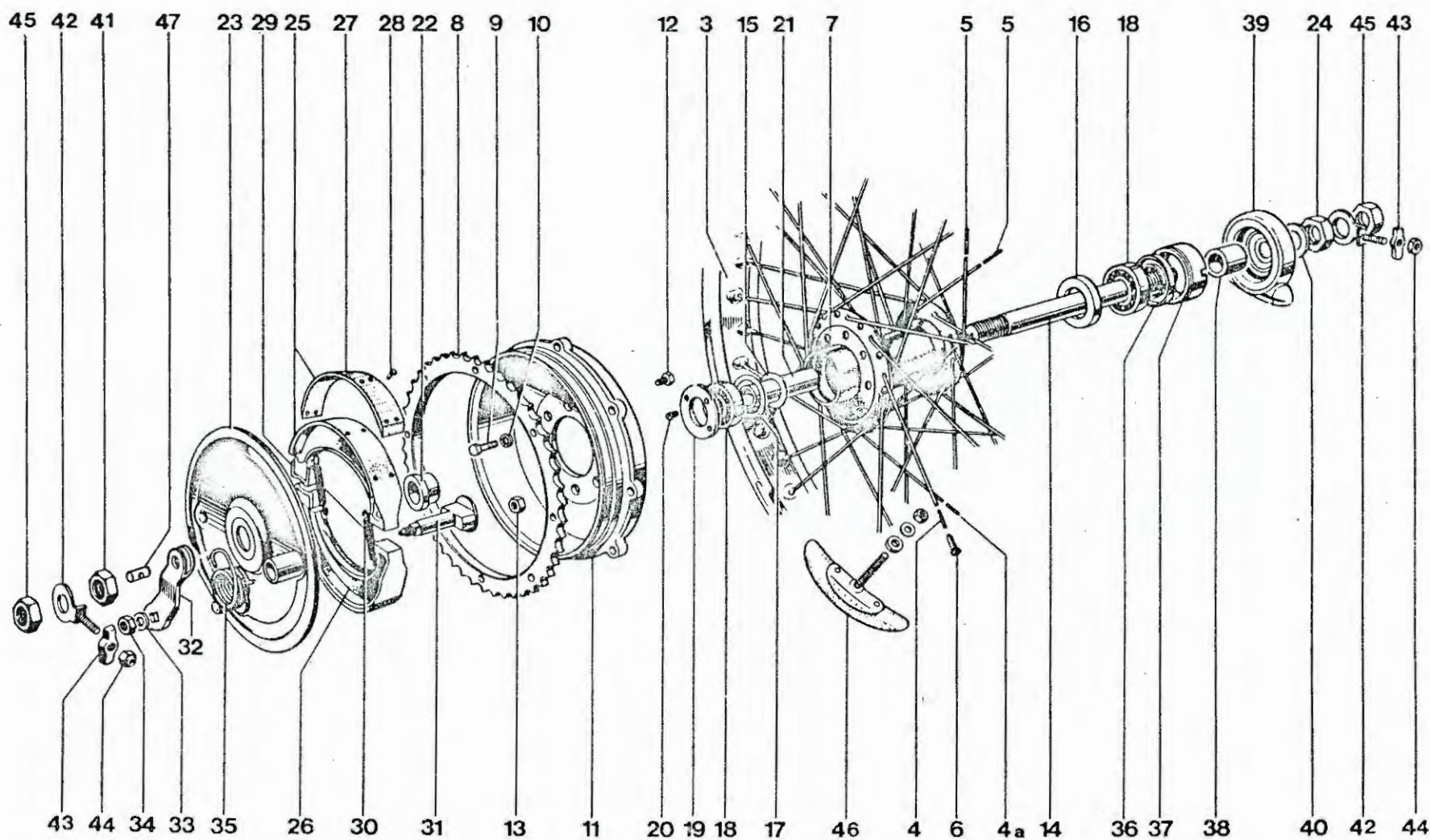
Fig. 18. REAR WHEEL
