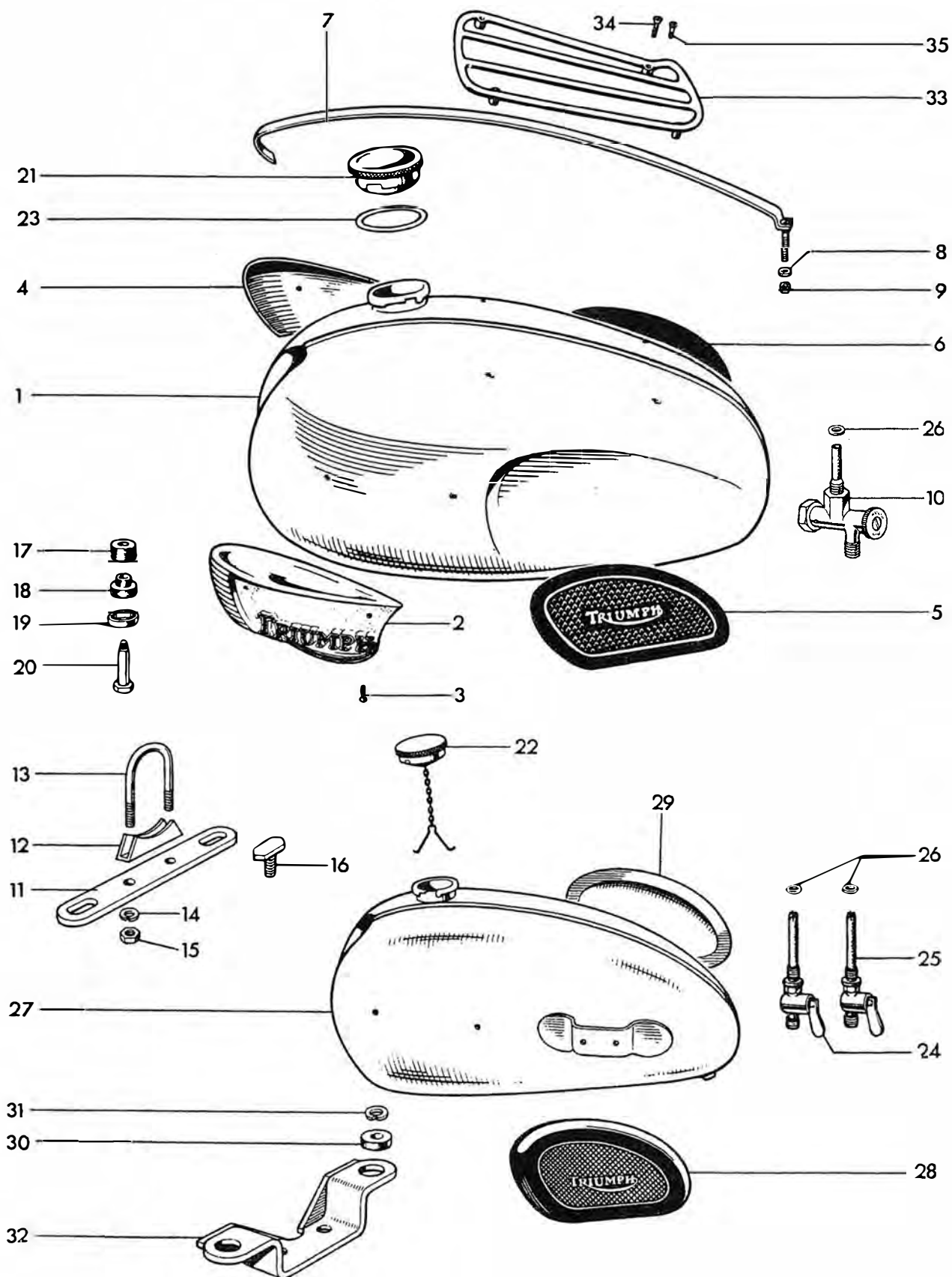
Fig. 25. PETROL TANK
