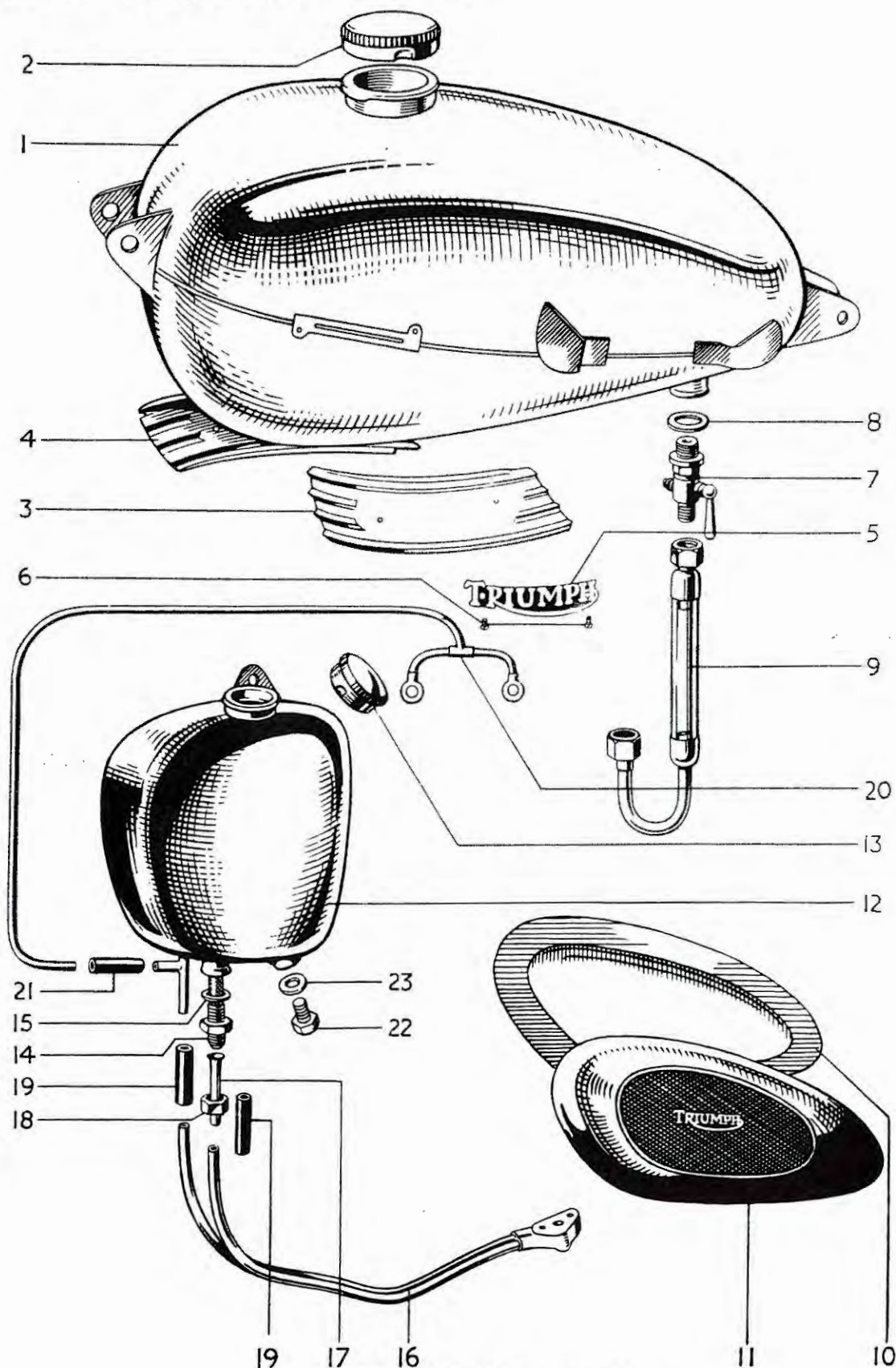
FIG. 12. PETROL AND OIL TANKS. For Index See Page 39.
