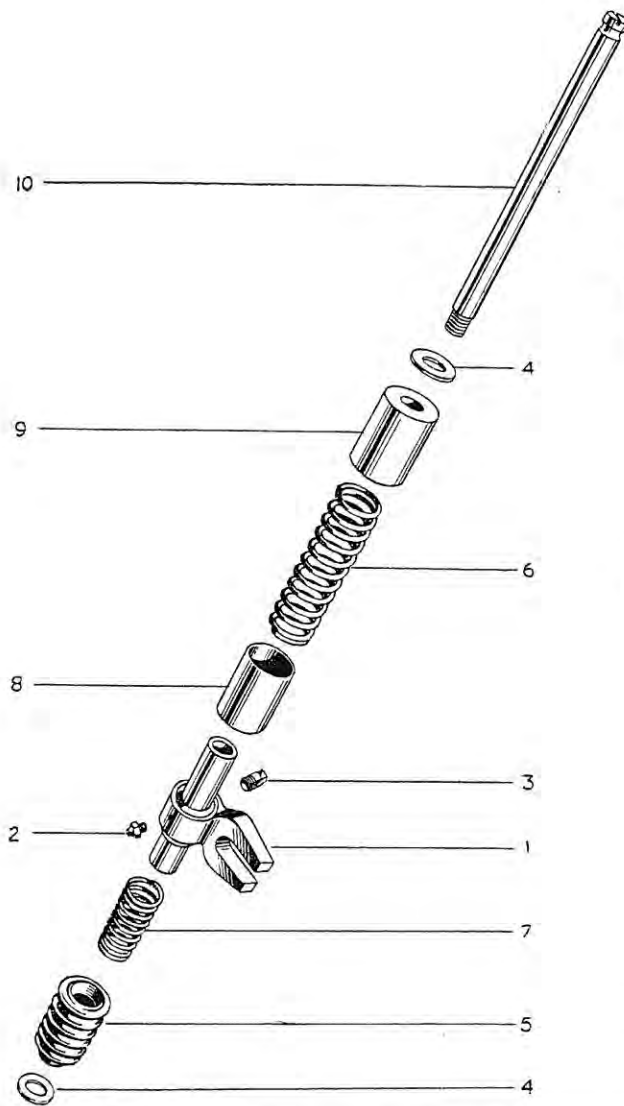
FIG. 5. REAR SUSPENSION.
