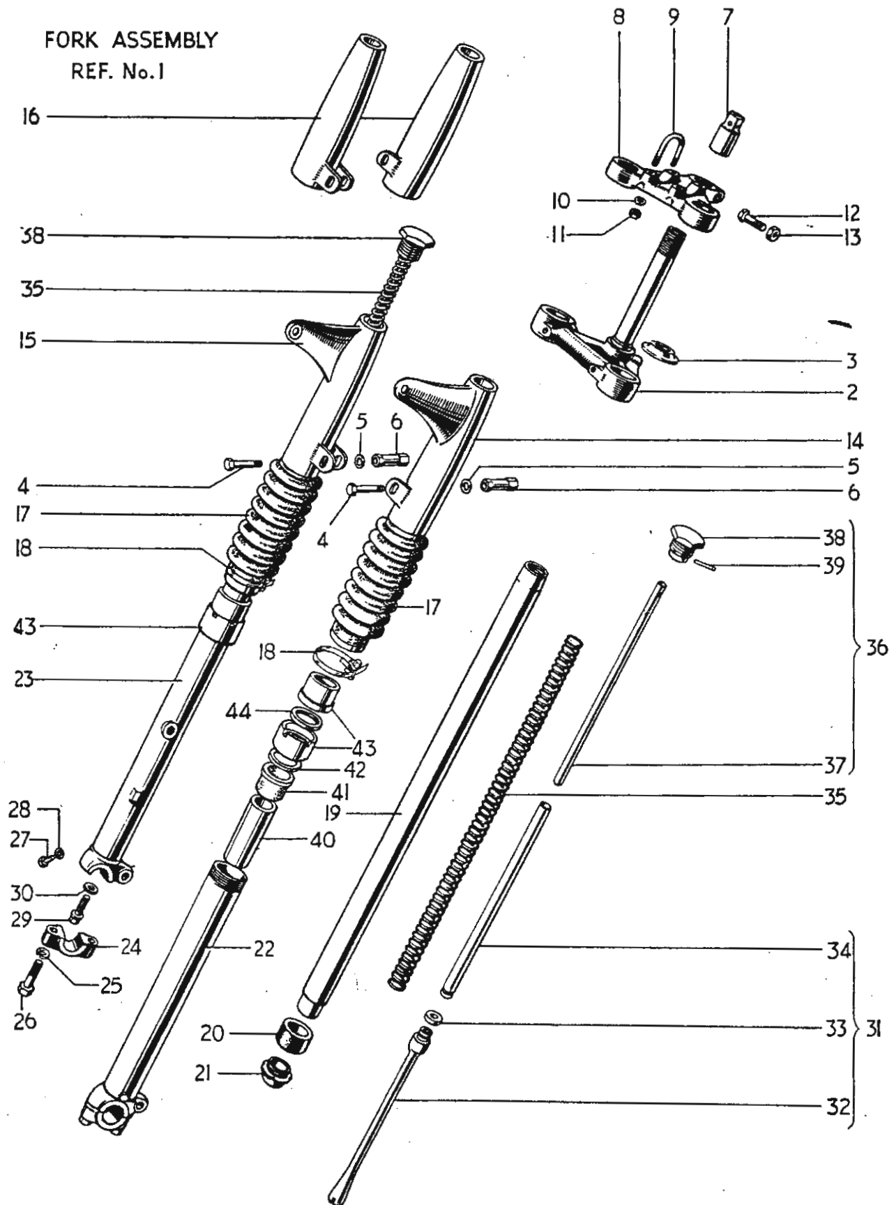
Fig. 10. TELESCOPIC FRONT FORK T20SS and T20SH
