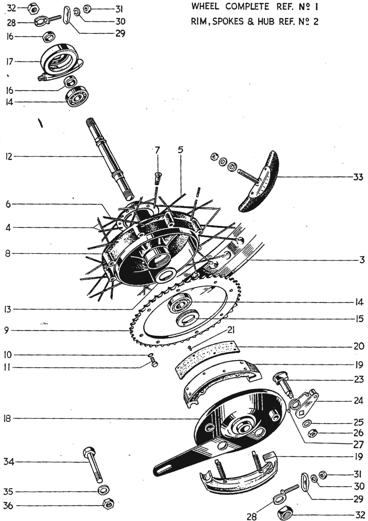
Fig. 13. REAR WHEEL
