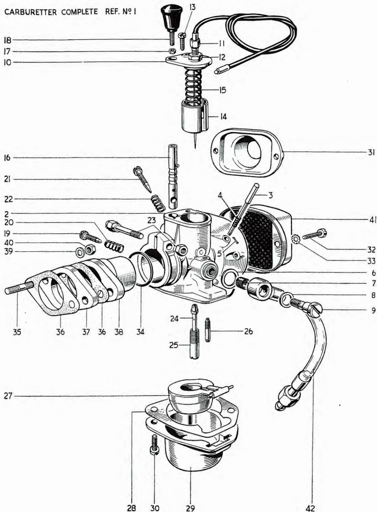
Fig. 25. ZENITH CARBURETTER.
