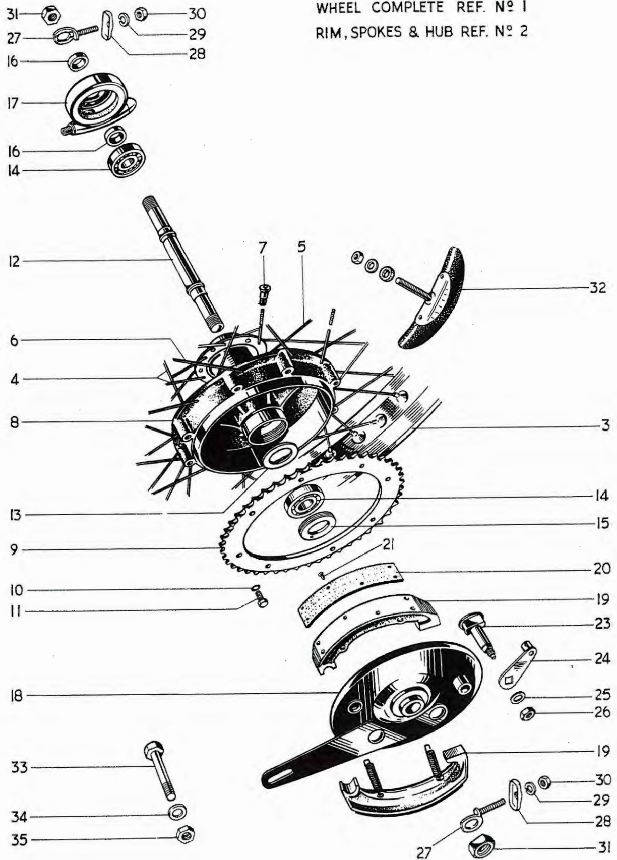
Fig. 17. REAR WHEEL.
