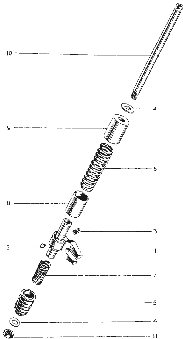
FIG. 5. REAR SUSPENSION.
