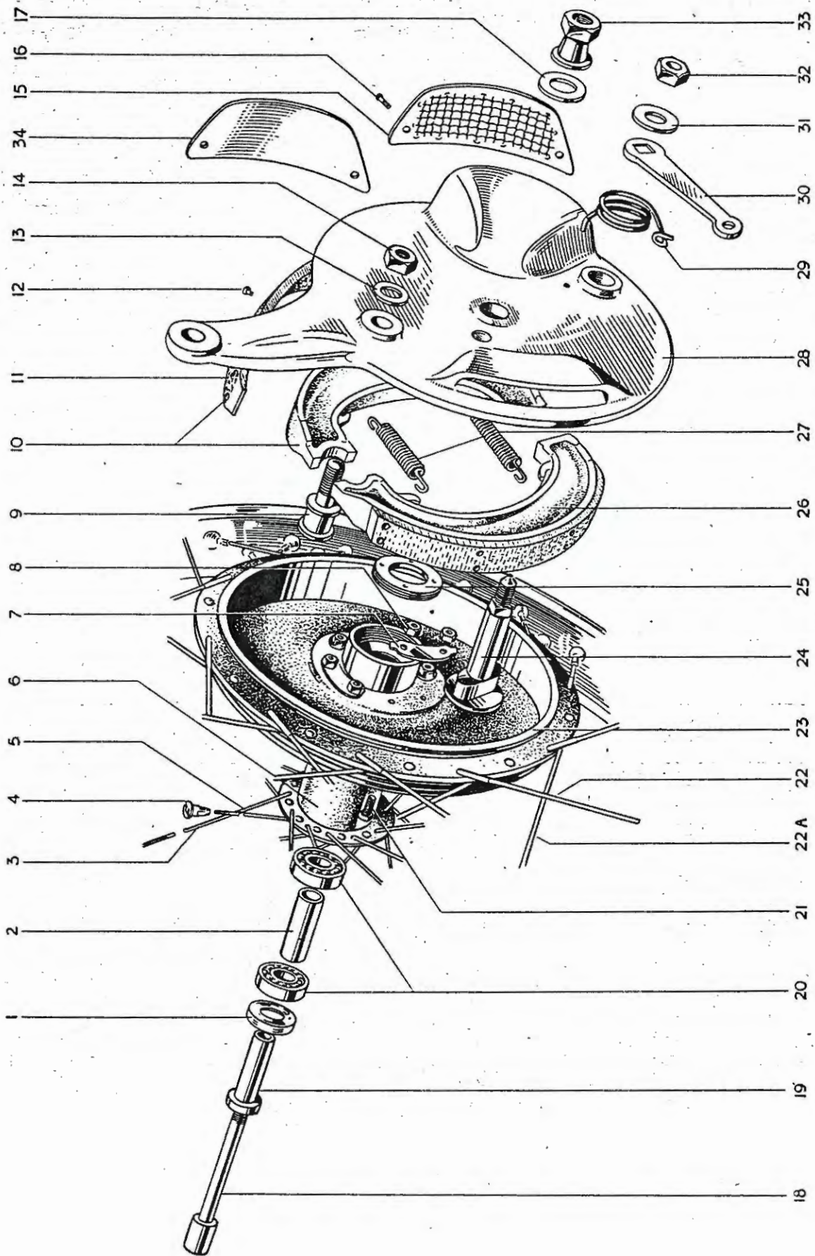
FIG. 19. FRONT WHEEL—TIGER 100 (T100) AND TIGER 110 (T110)
