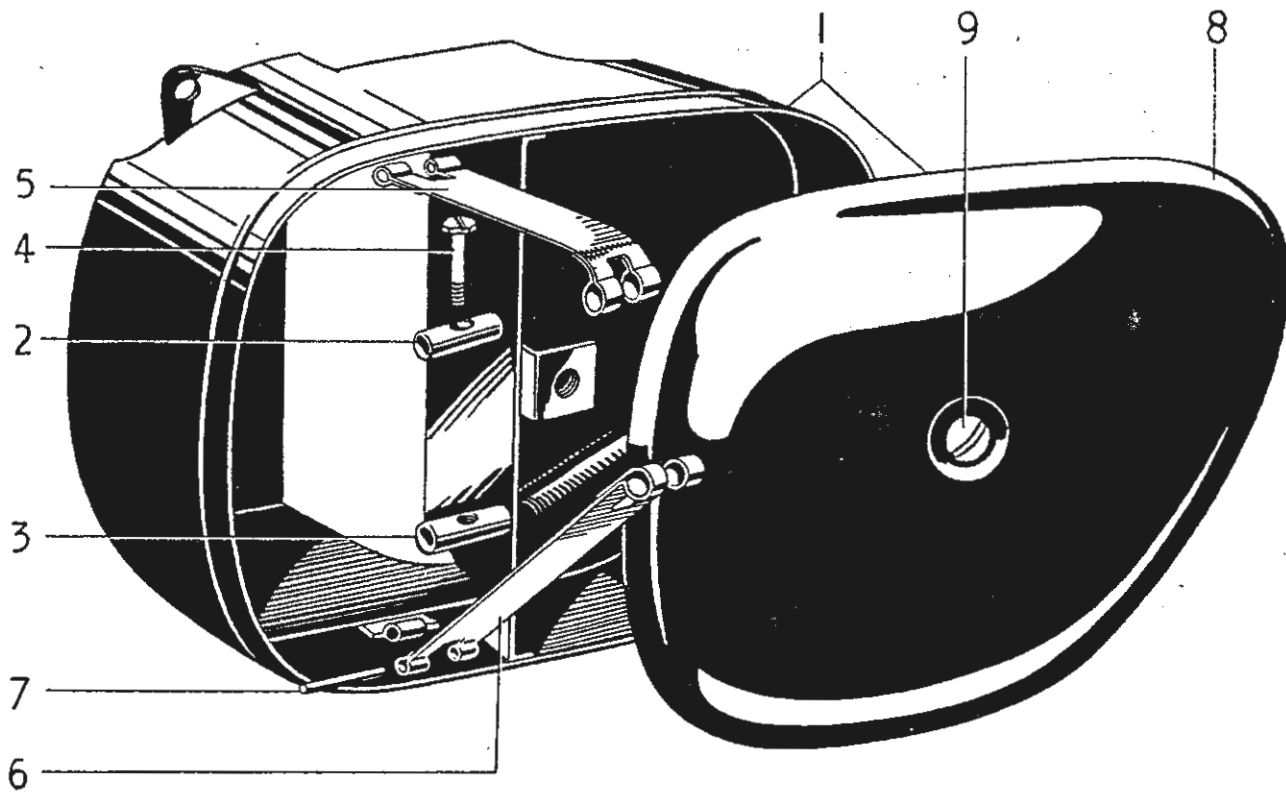
FIG. 27. BATTERY CARRIER AND TOOL BOX
