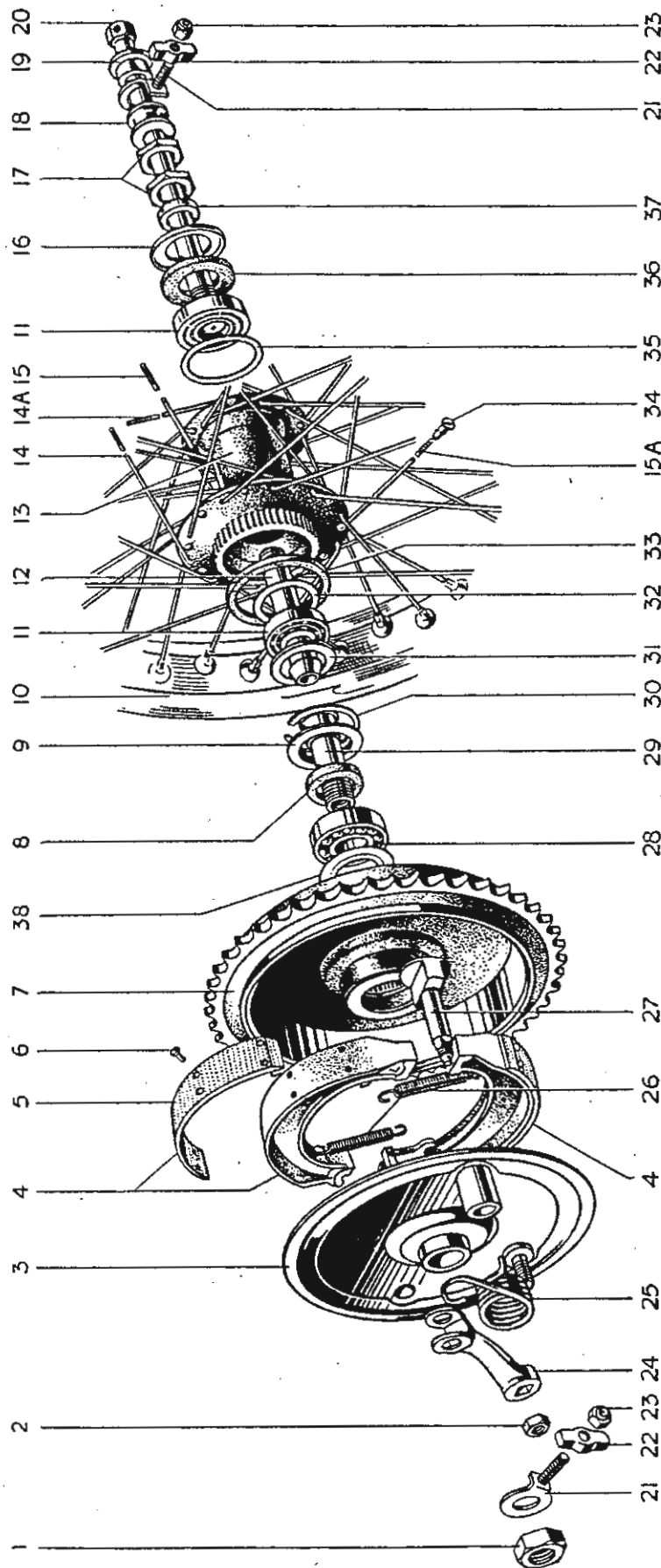
FIG. 21. REAR WHEEL (QUICKLY DETACHABLE)
