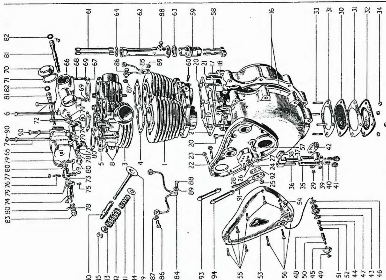
FIG. 2. CRANKCASE, CYLINDER BLOCK, CYLINDER HEAD, etc.
