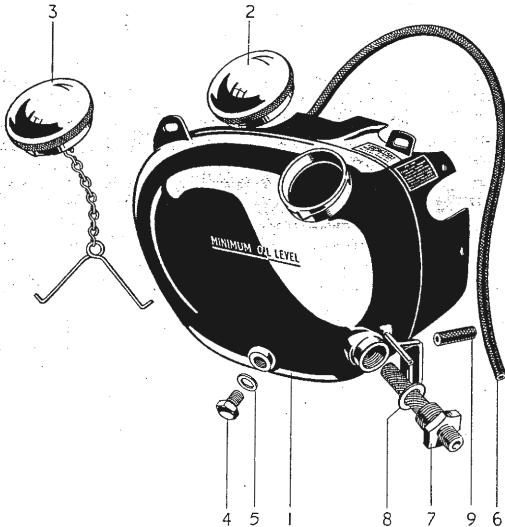
FIG. 24. OIL TANK
