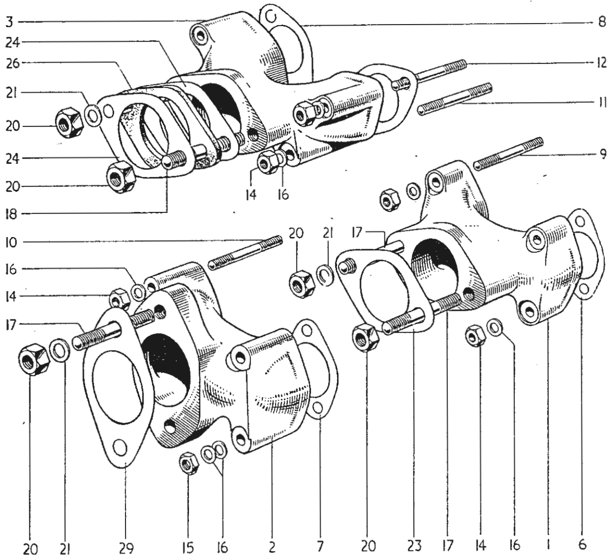
FIG. 1. INLET MANIFOLDS
