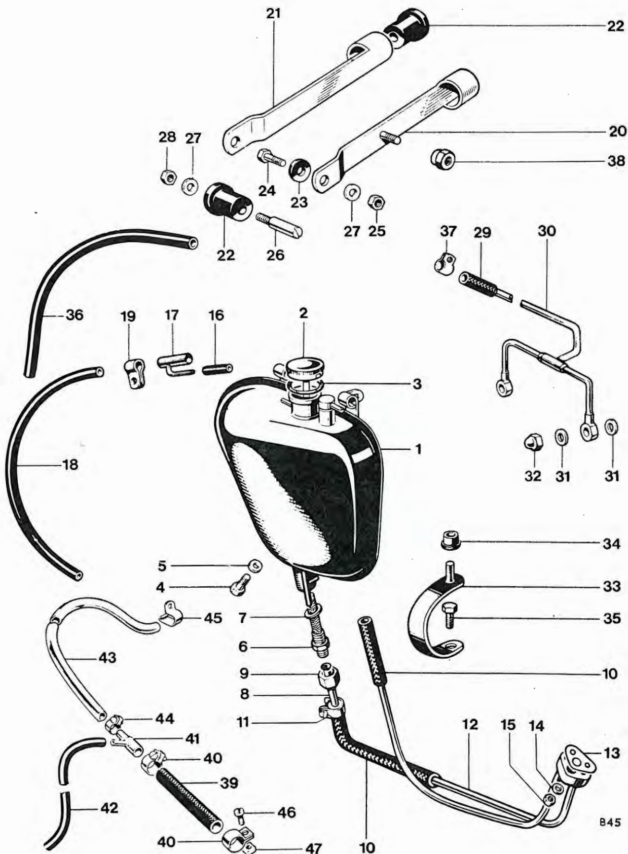
Fig. 22. OIL TANK
