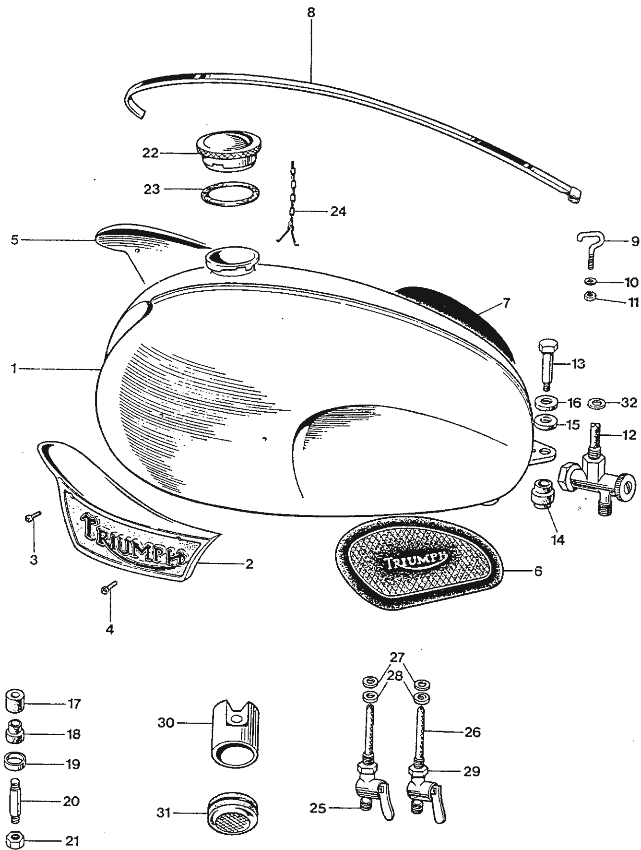
Fig. 25. PETROL TANK
