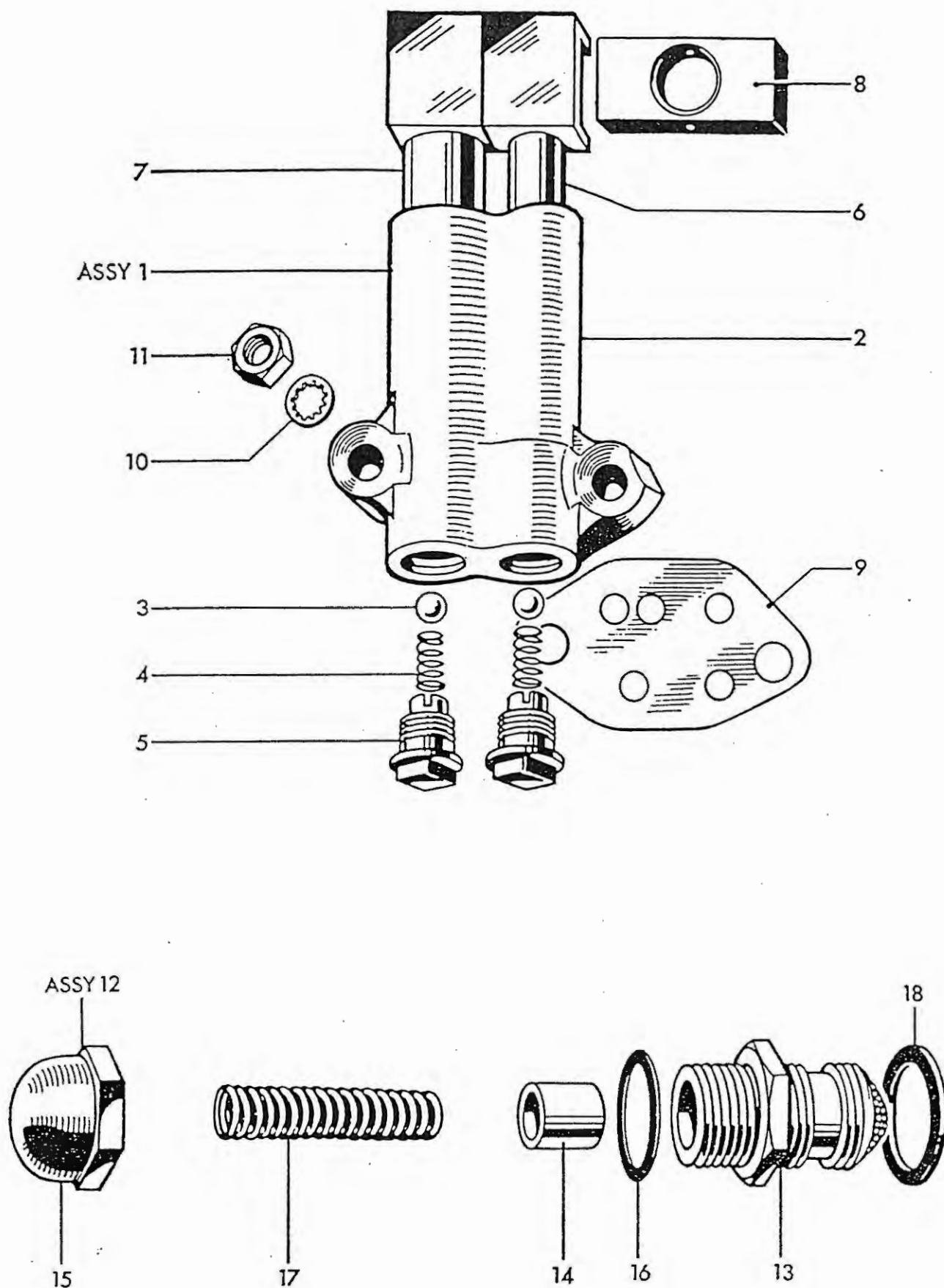
Fig. 3. OIL PUMP AND RELEASE VALVE
