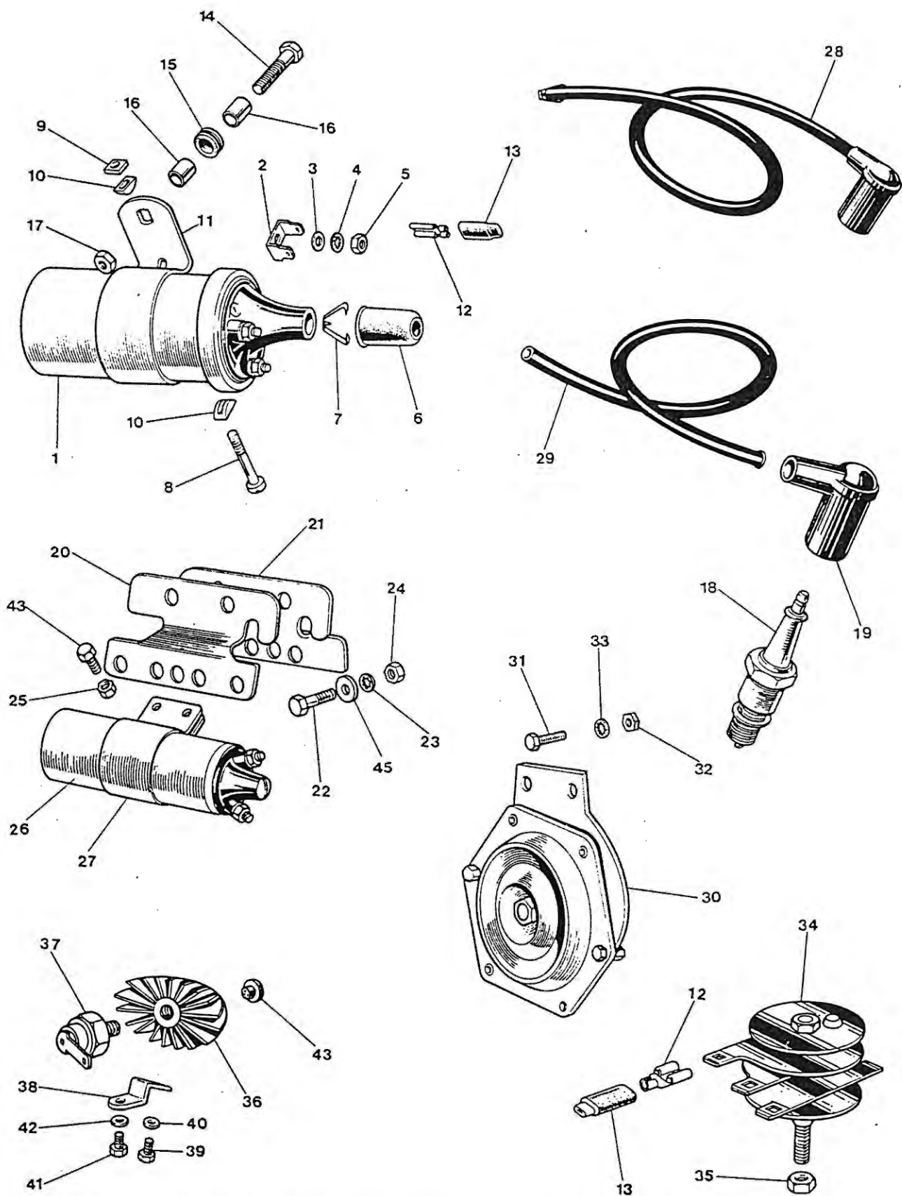
Fig. 32. IGNITION COILS, HORN, RECTIFIER AND ZENER DIODE
