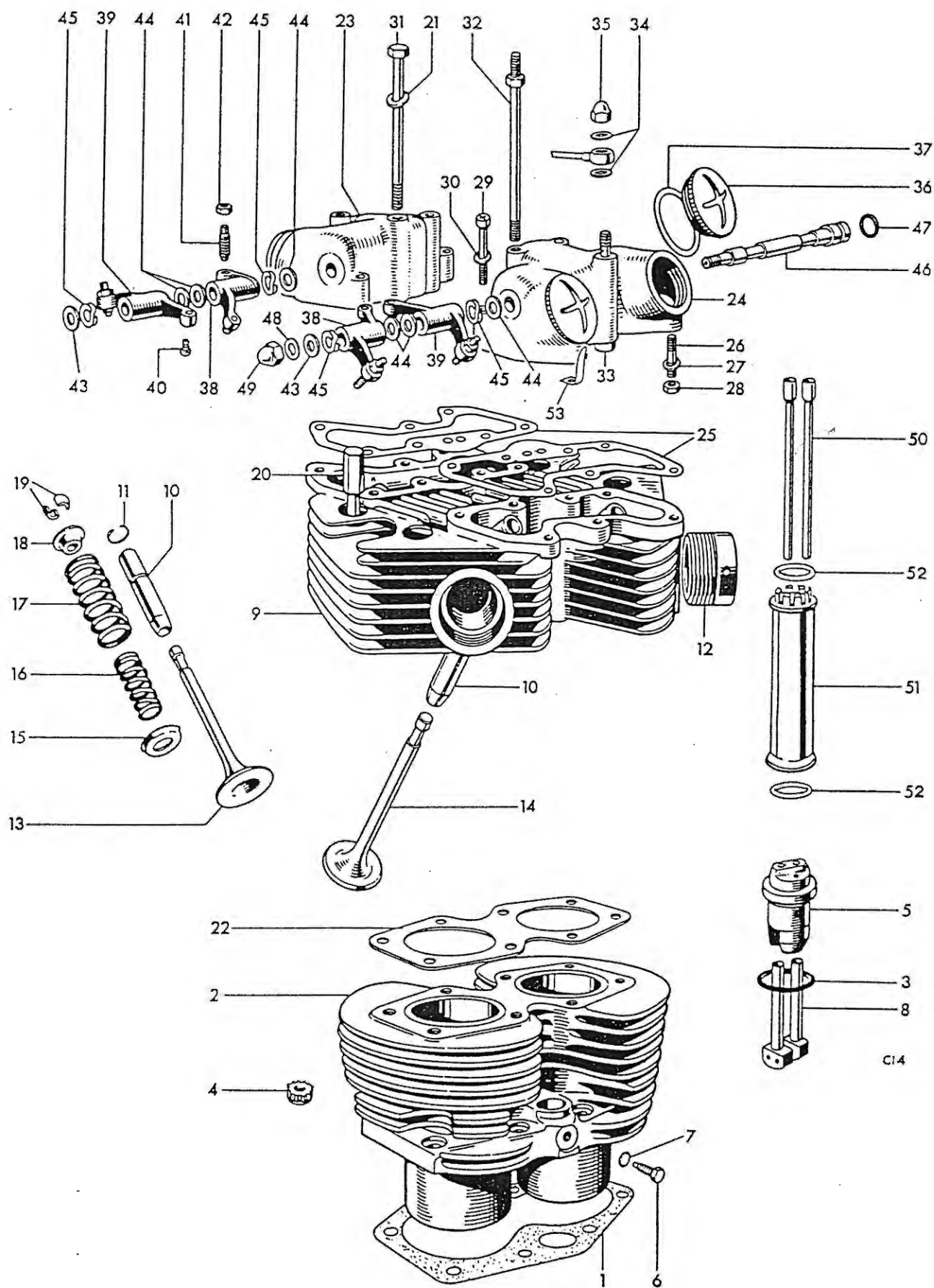
Fig. 7. CYLINDER BLOCK AND HEAD, T100R, T100T
