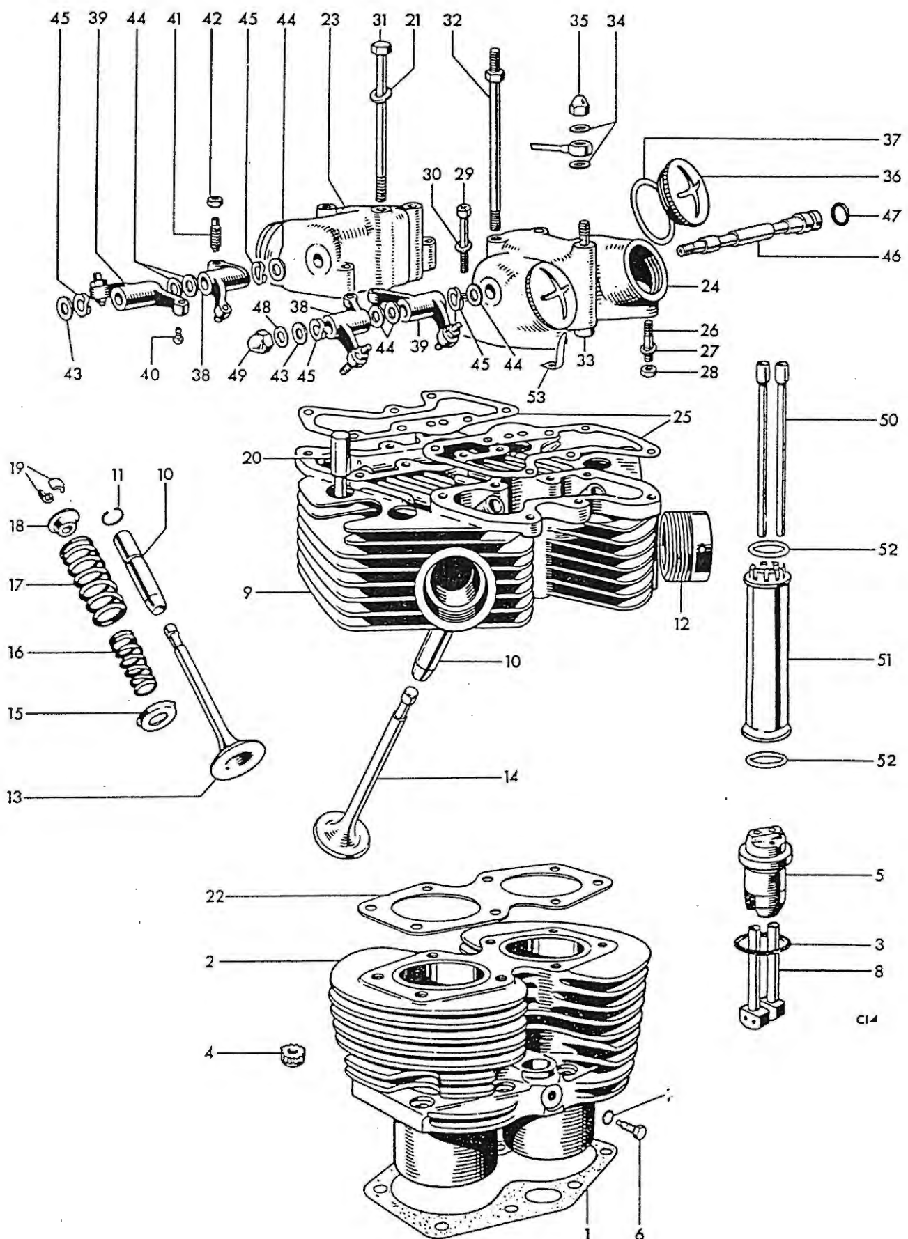
Fig. 6. CYLINDER BLOCK AND HEAD, T100S AND T100C
