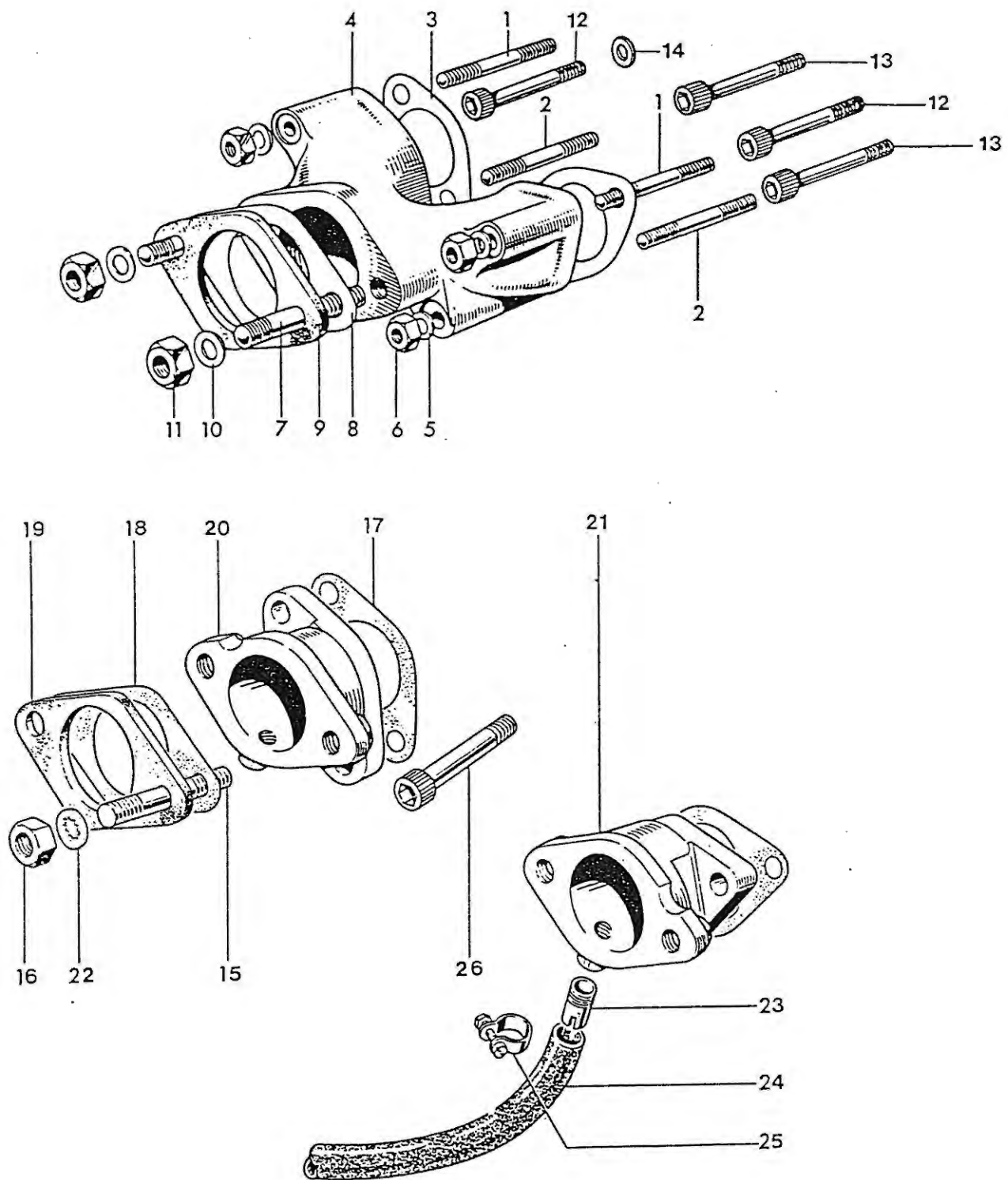
Fig. 4. INLET MANIFOLDS
