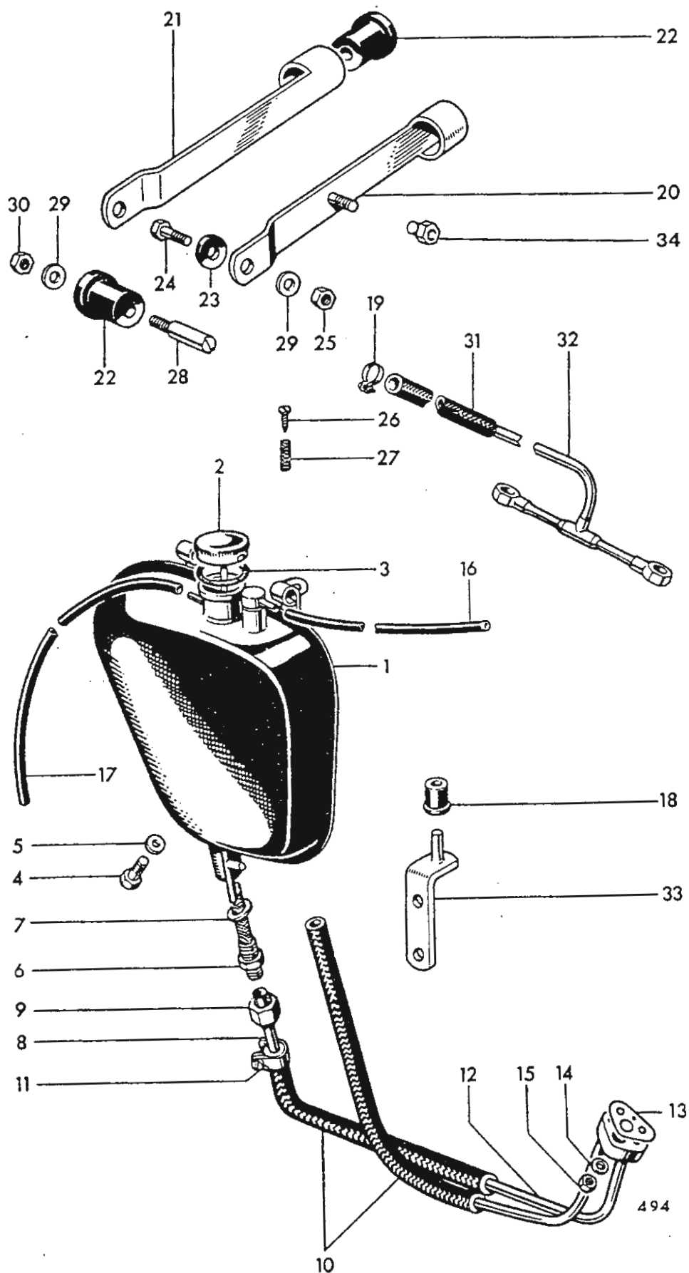
Fig. 26. OIL TANK
