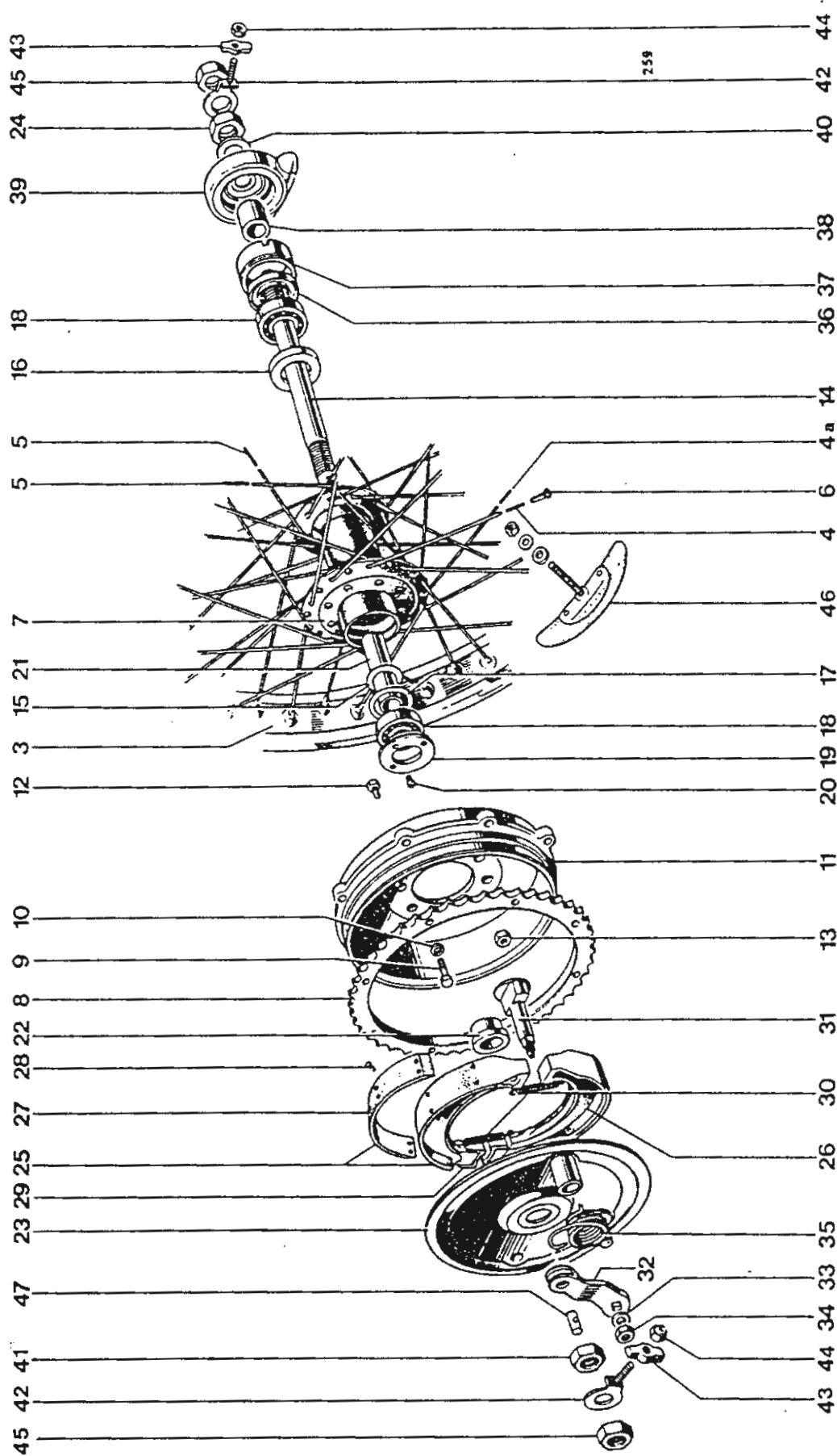
Fig. 21. REAR WHEEL
