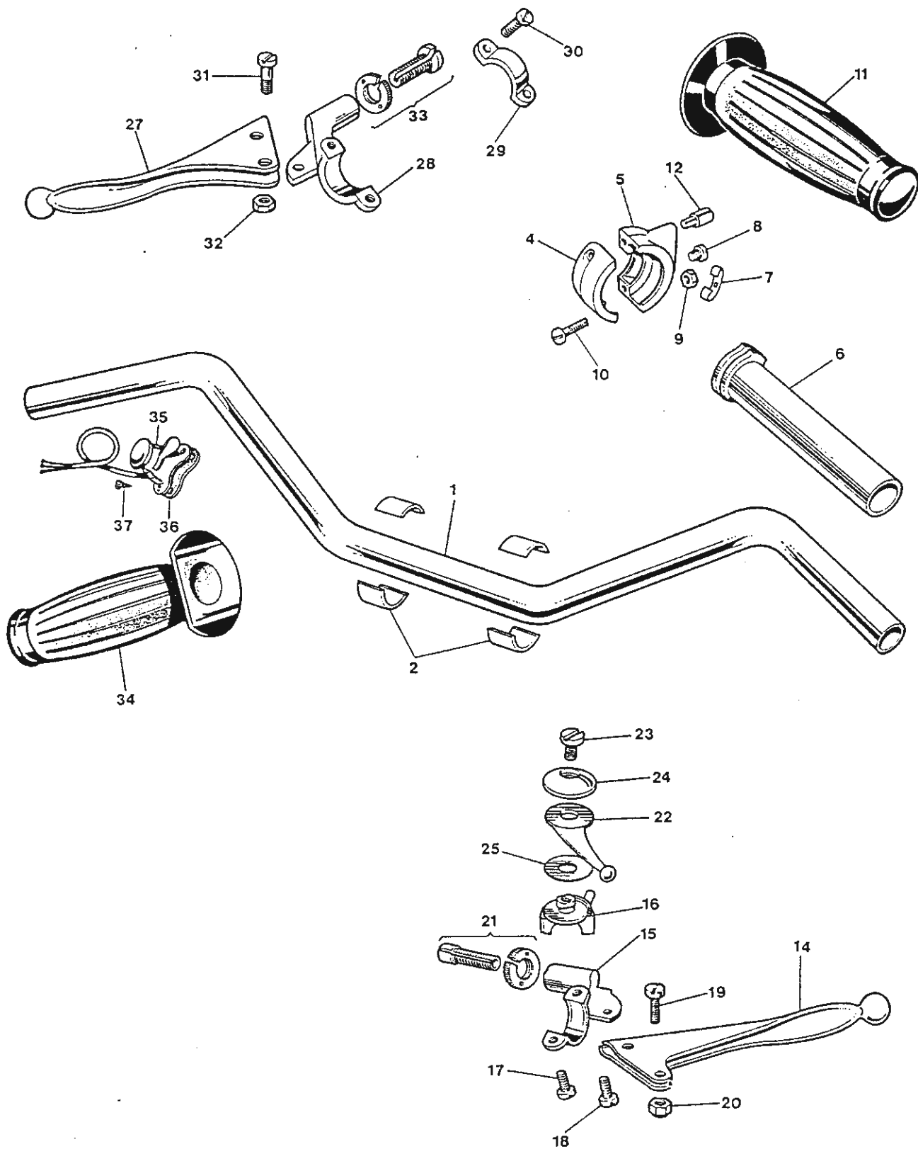
Fig. 28. HANDLEBARS AND CONTROL LEVERS
