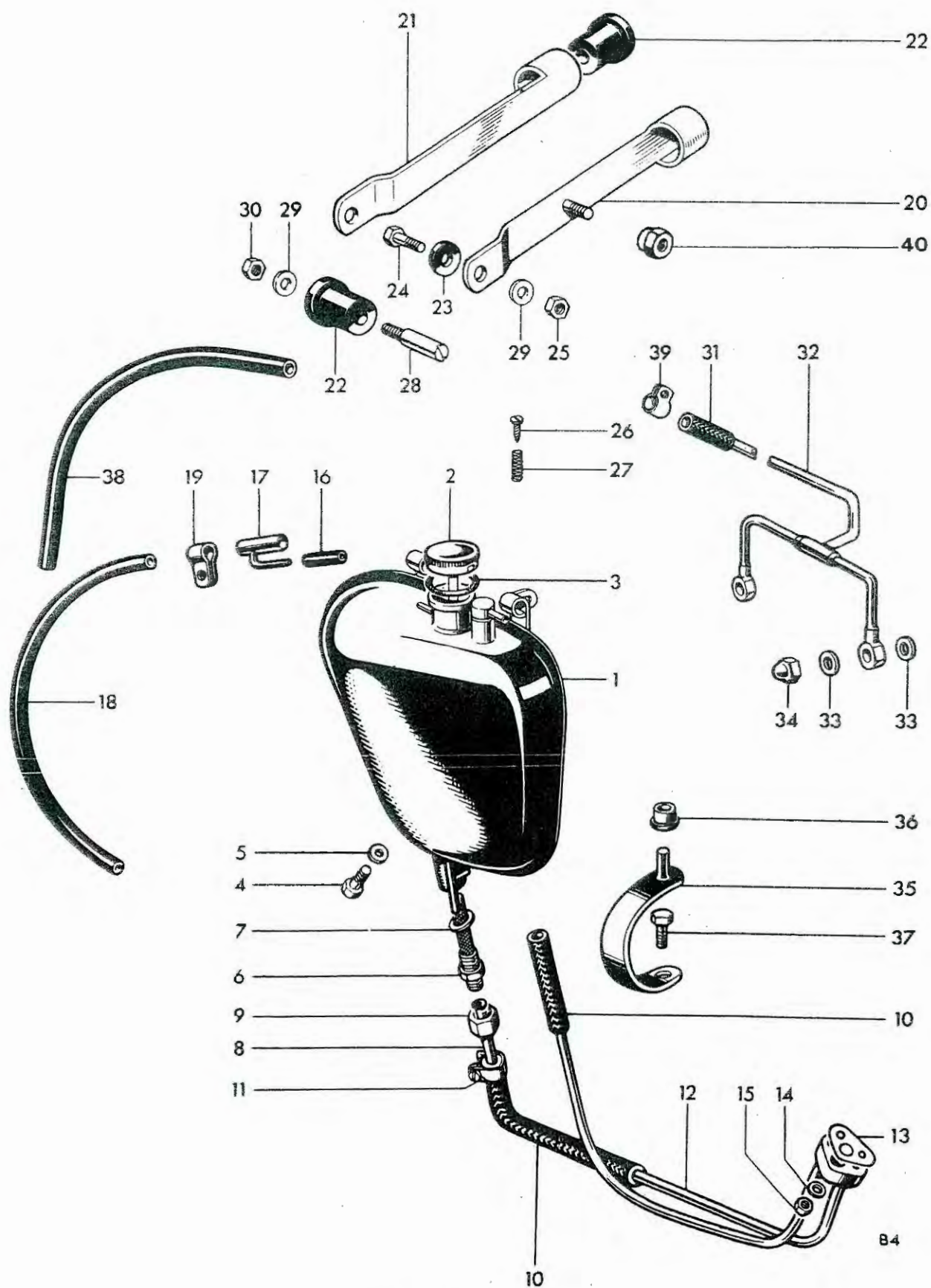
Fig. 23. OIL TANK
