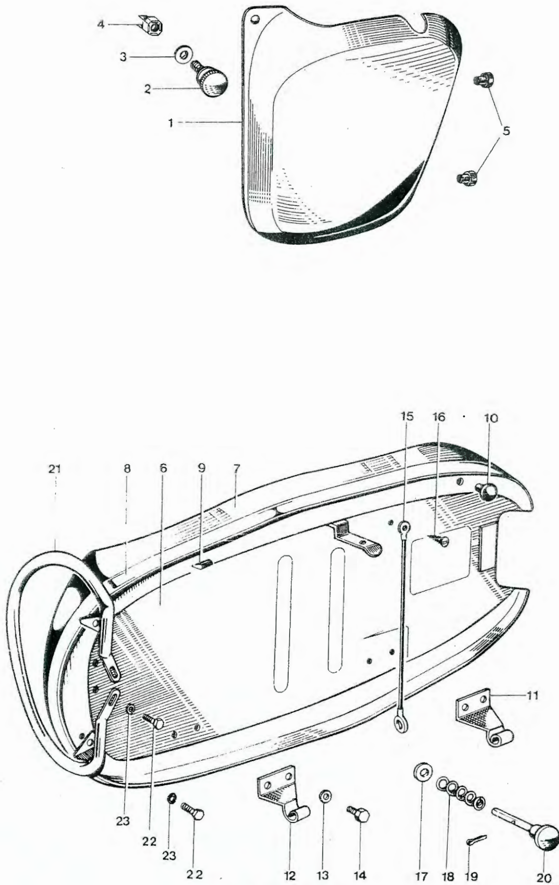
Fig. 24. PANEL AND TWINSEAT
