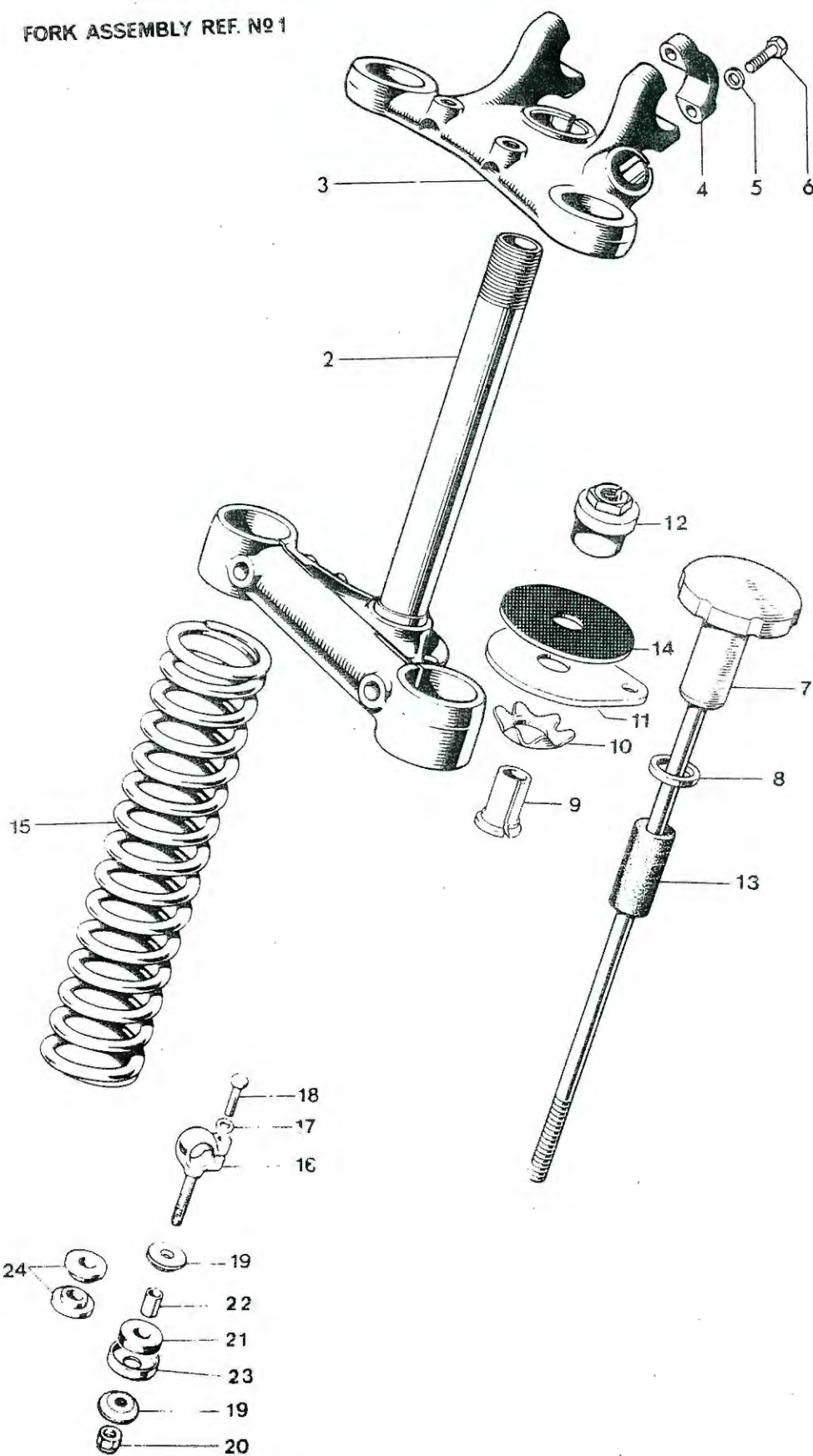
Fig. 18. TR6C FORK PARTS AND STEERING DAMPER
