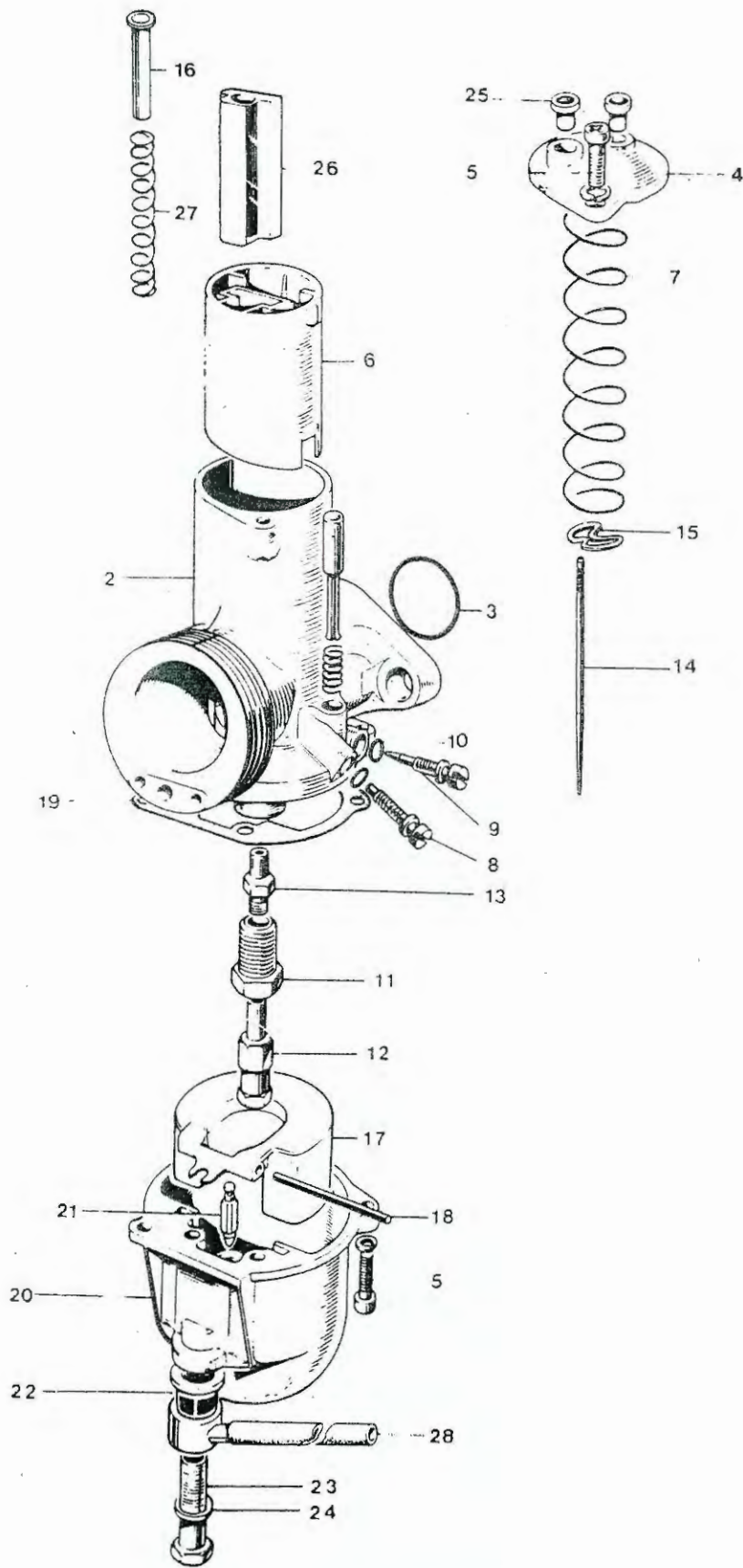
Fig. 30. AMAL CARBURETTOR, TR6R TR6C
