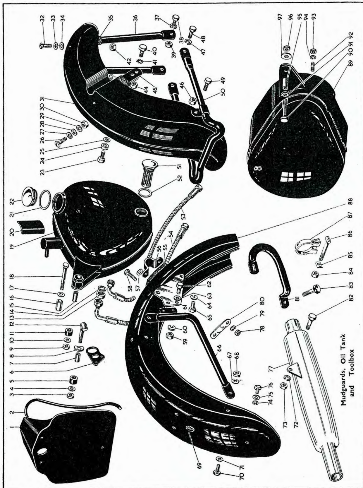
Plate 10 MUDGUARDS, OIL TANK, SILENCER and TOOLBOX B31 B33 (Swinging Arm)
