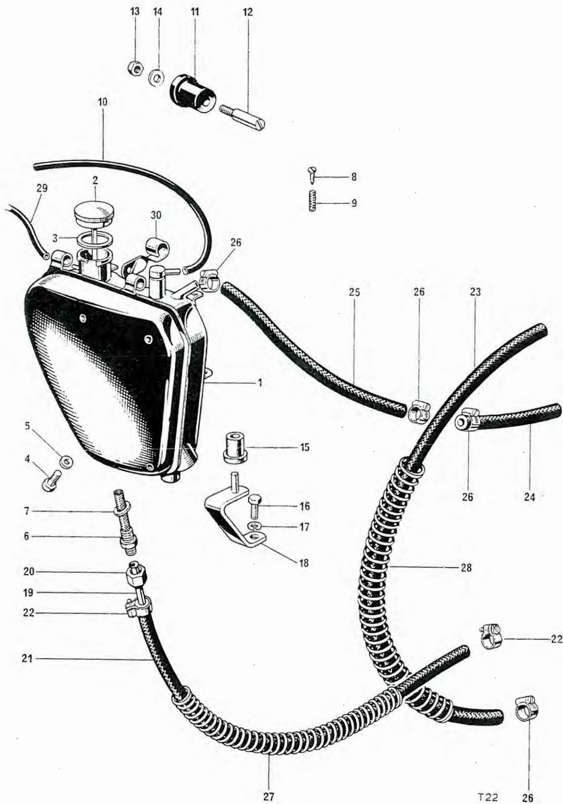
Fig. 24. OIL TANK
