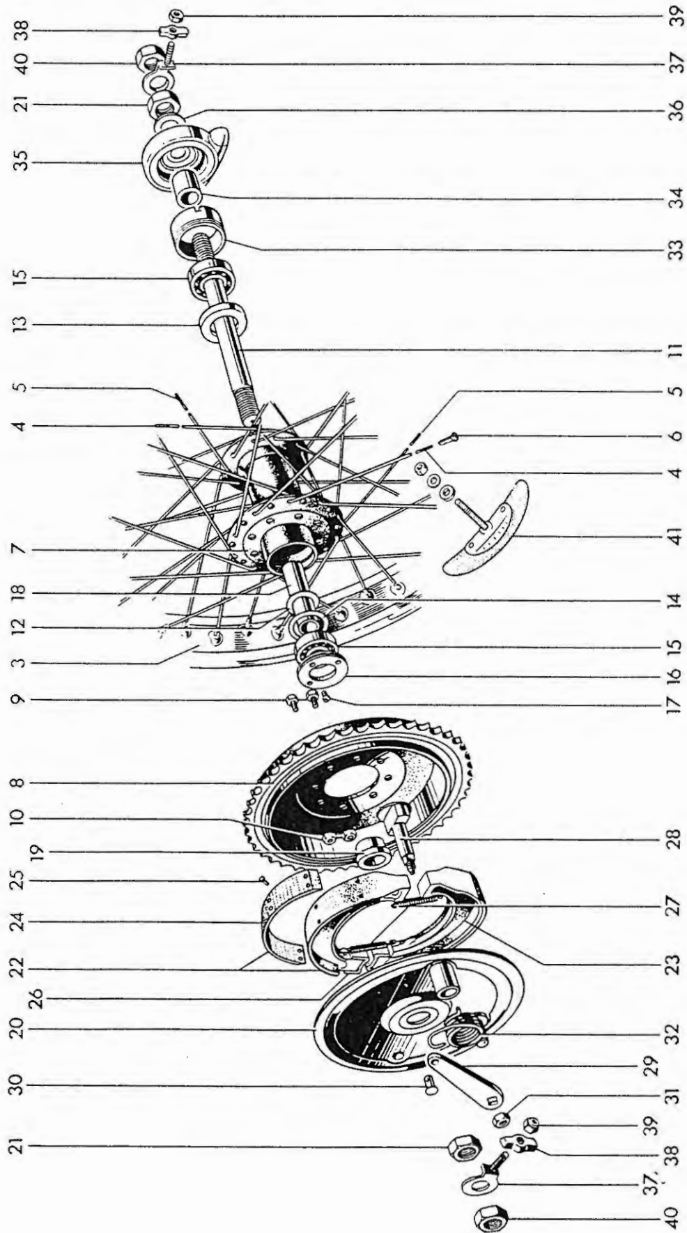
Fig. 18. REAR WHEEL
