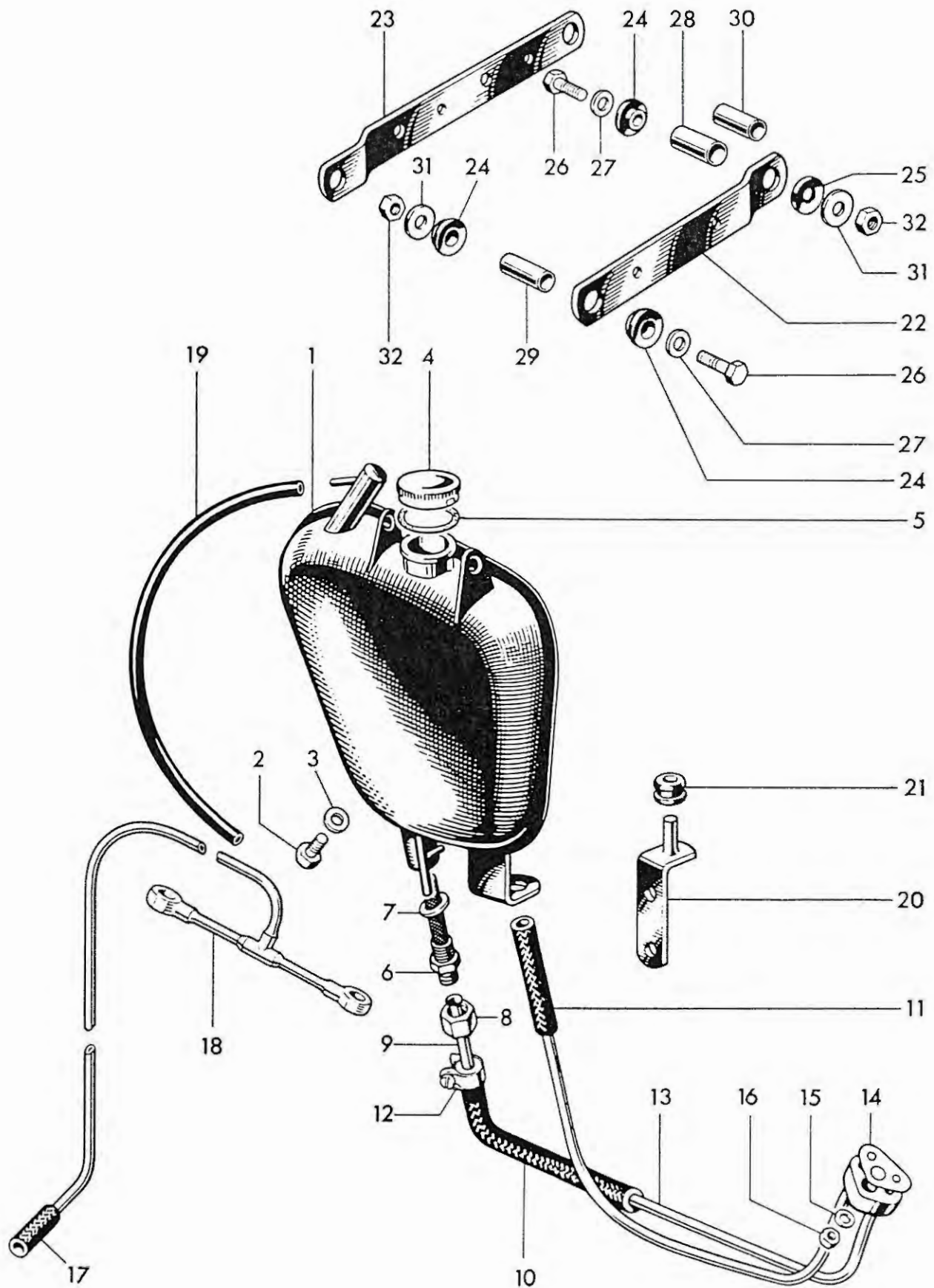
Fig. 23. OIL TANK
