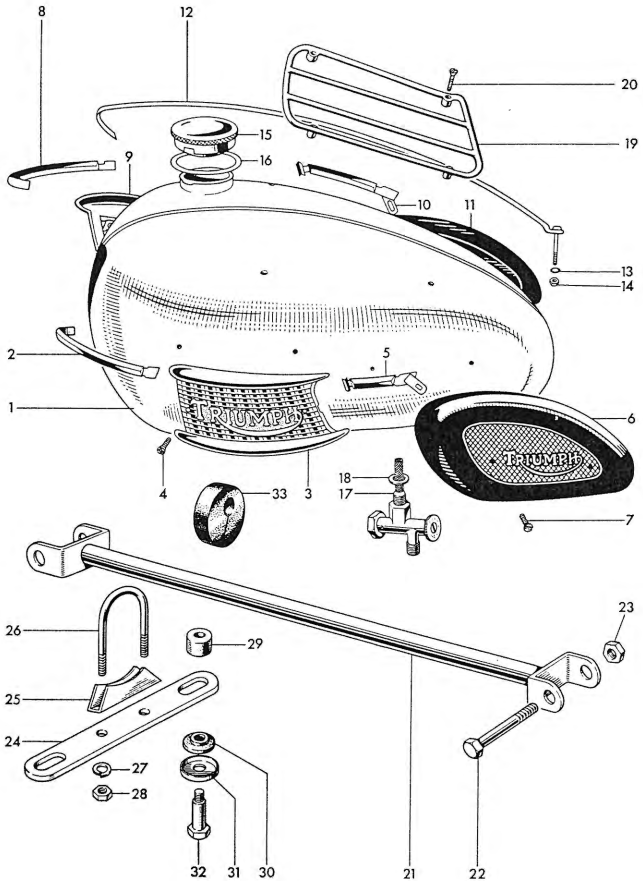
Fig. 22. PETROL TANK
