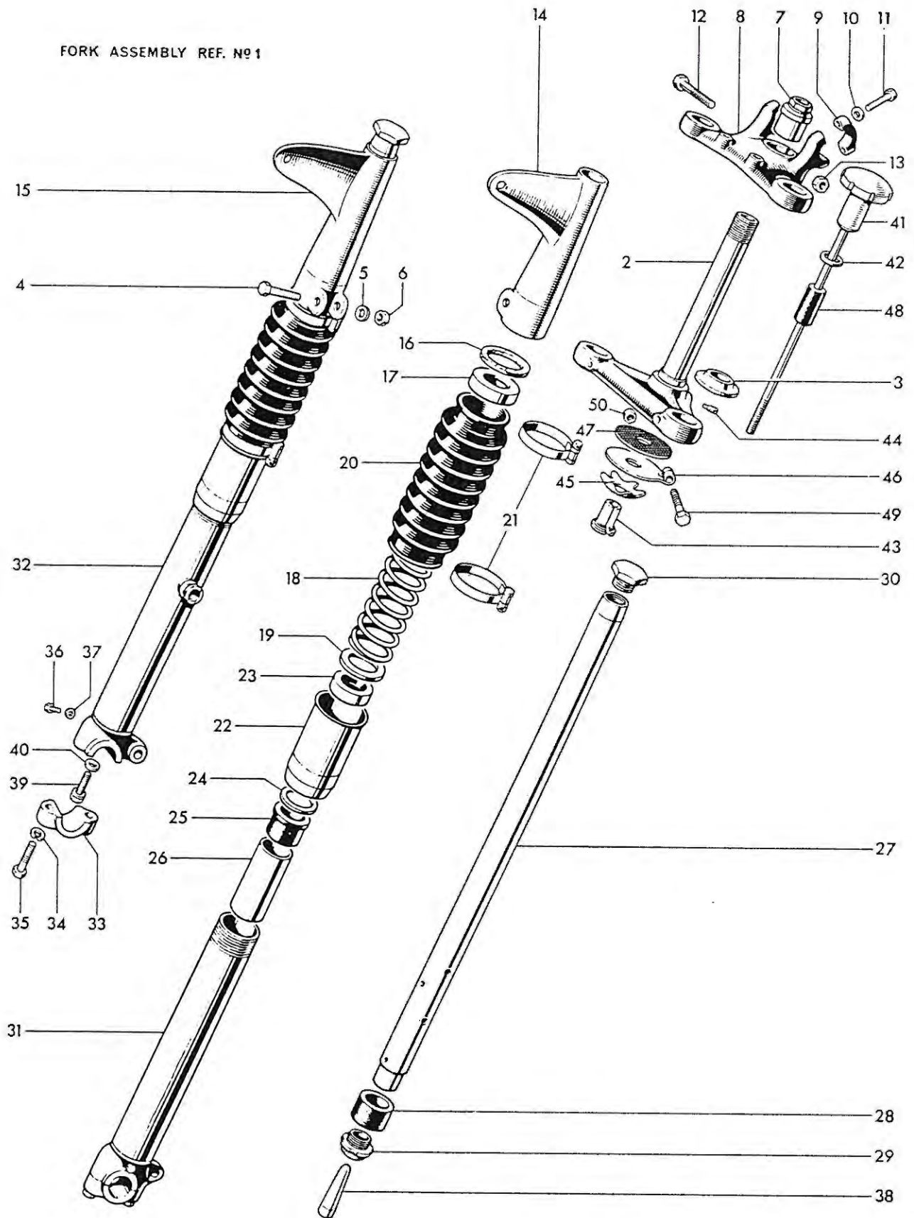
Fig. 16. TELESCOPIC FRONT FORK, T90 AND T10055
