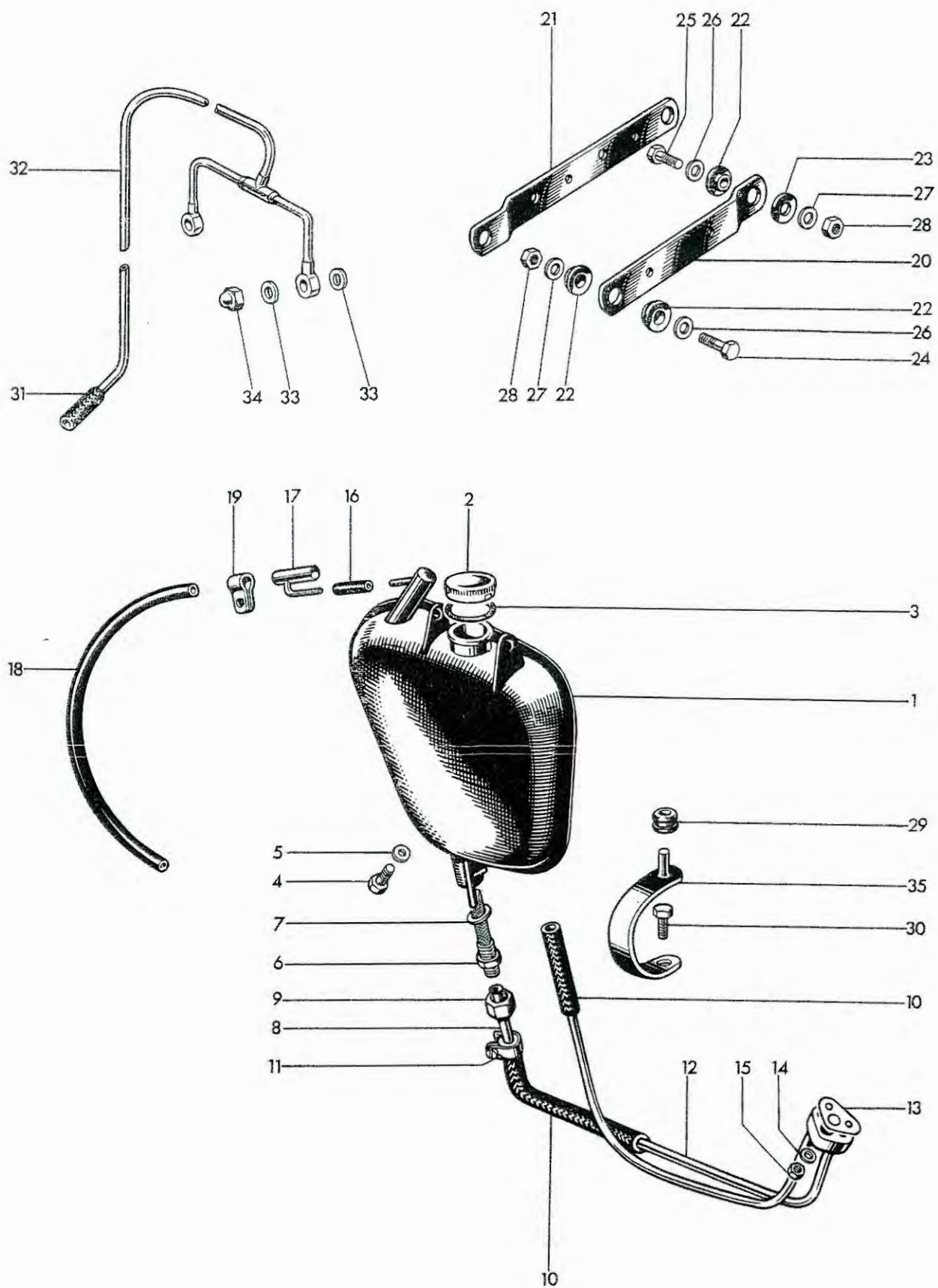
Fig. 23. OIL TANK
