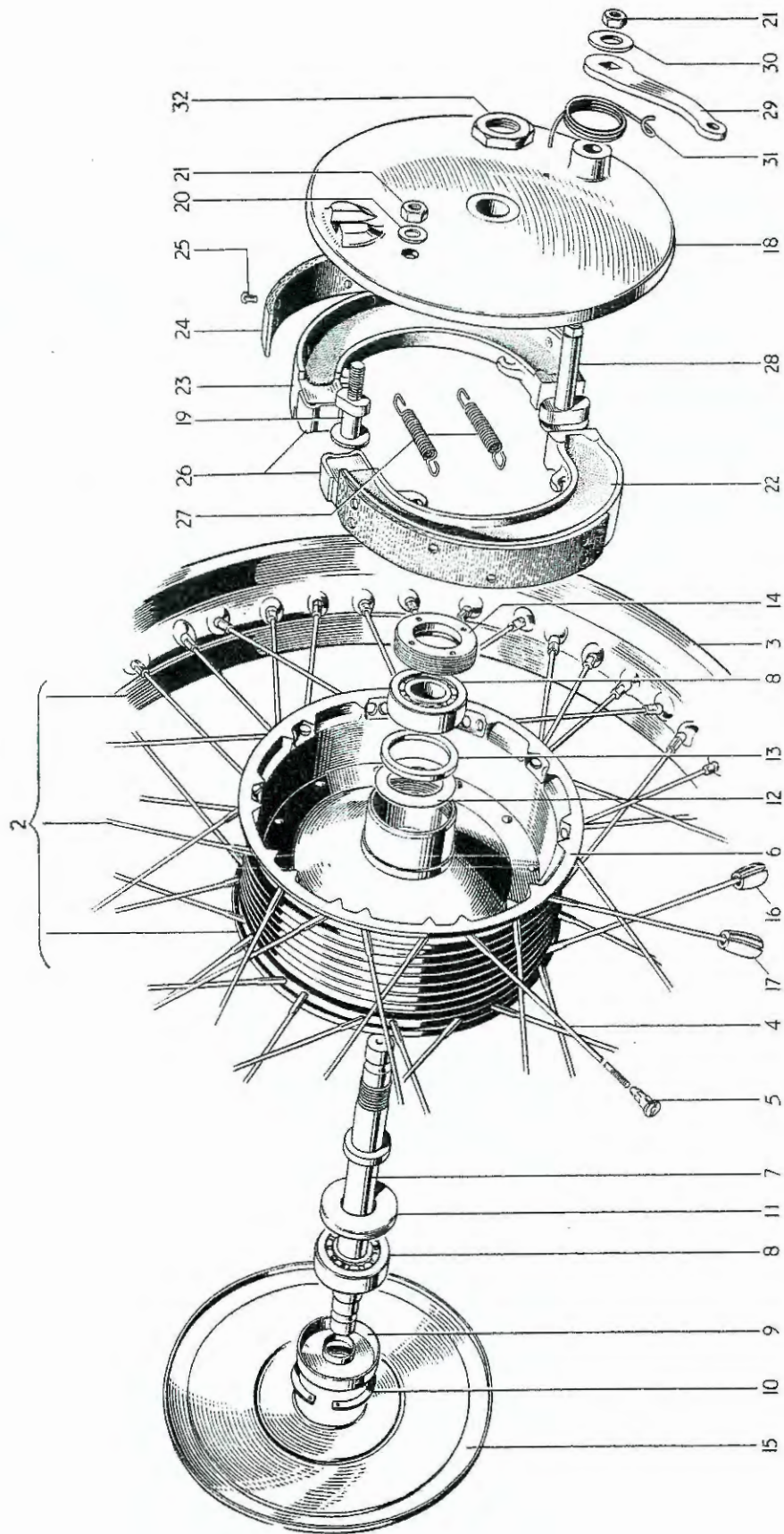
Fig. 19. FRONT WHEEL
