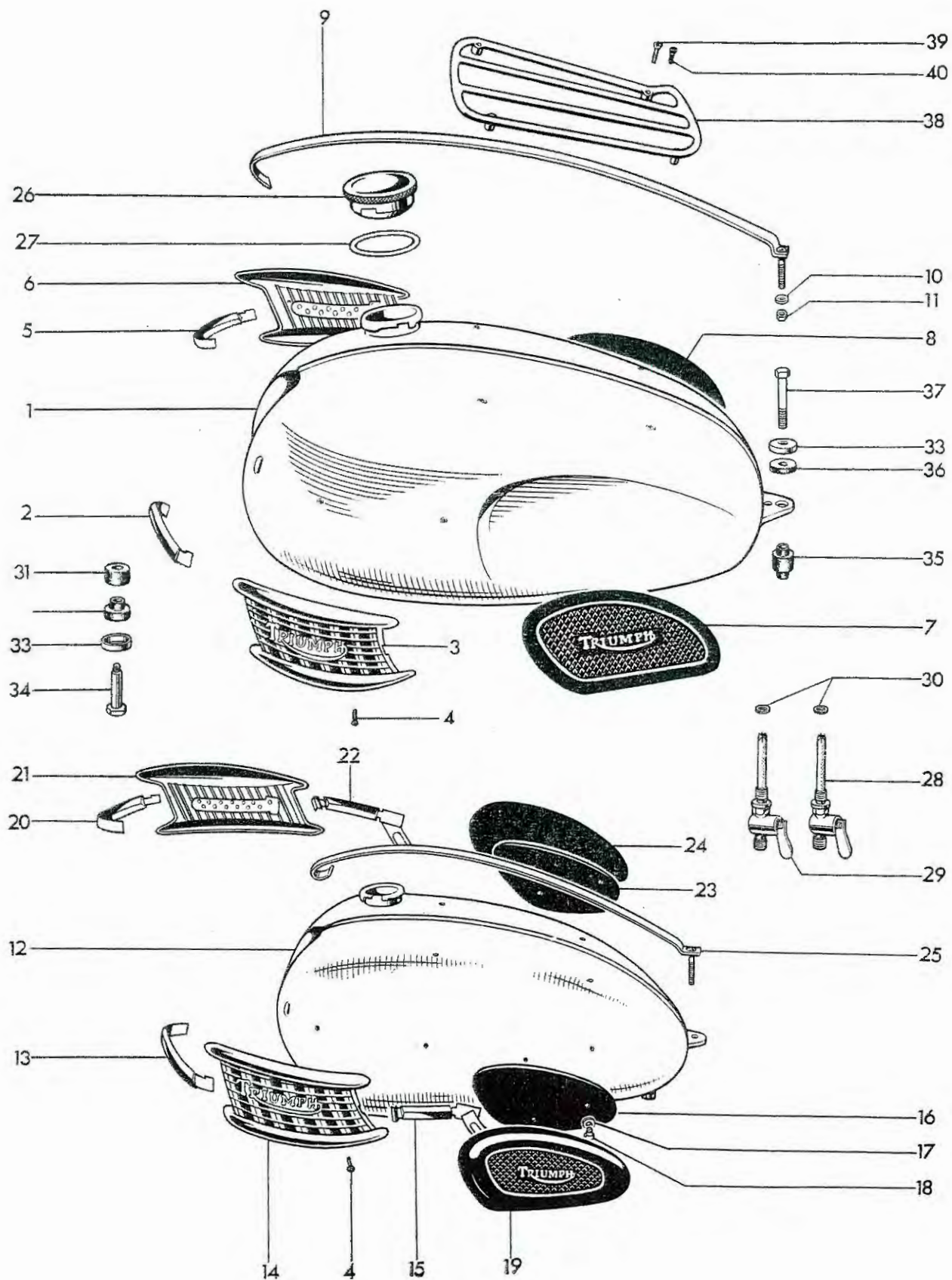
Fig. 22. PETROL TANKS
