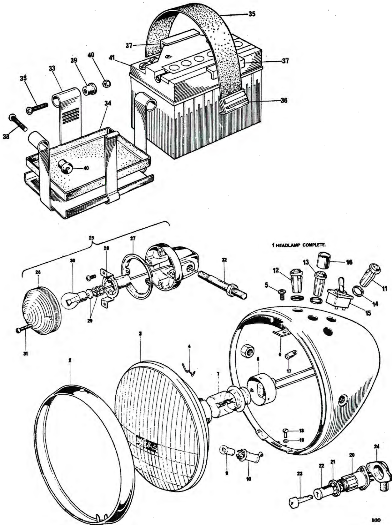
Fig. 14. HEADLAMP AND FLASHER LAMPS
