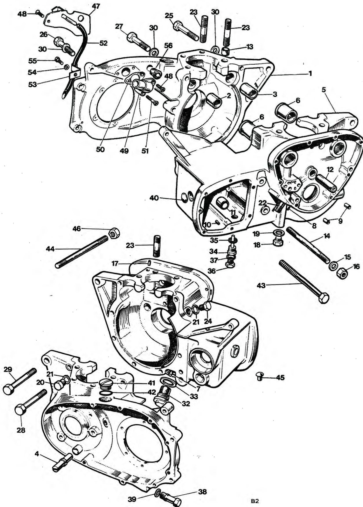
Fig. 2 CRANKCASE
