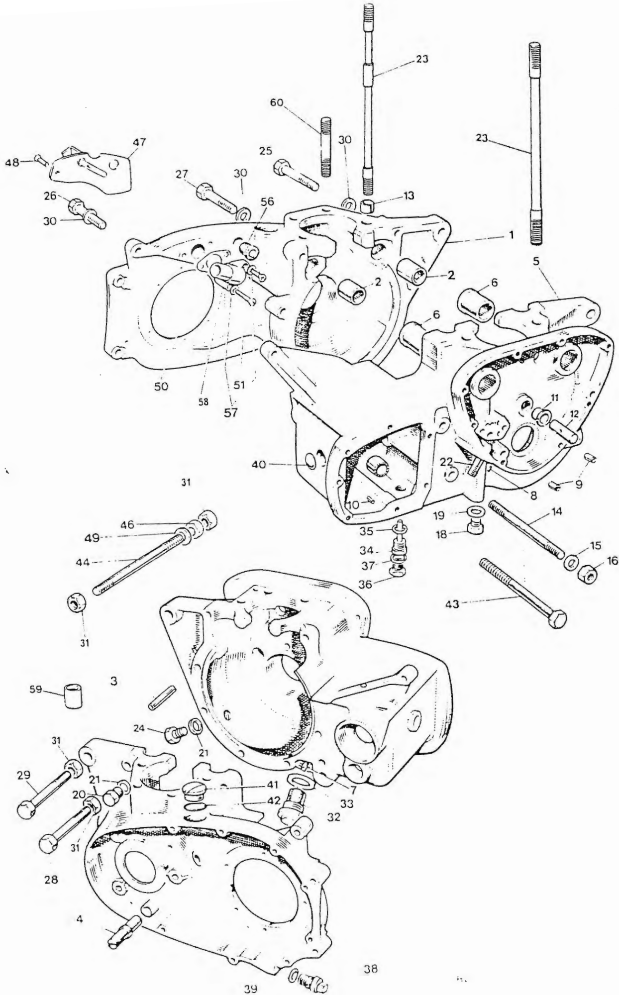
CRANKCASE
