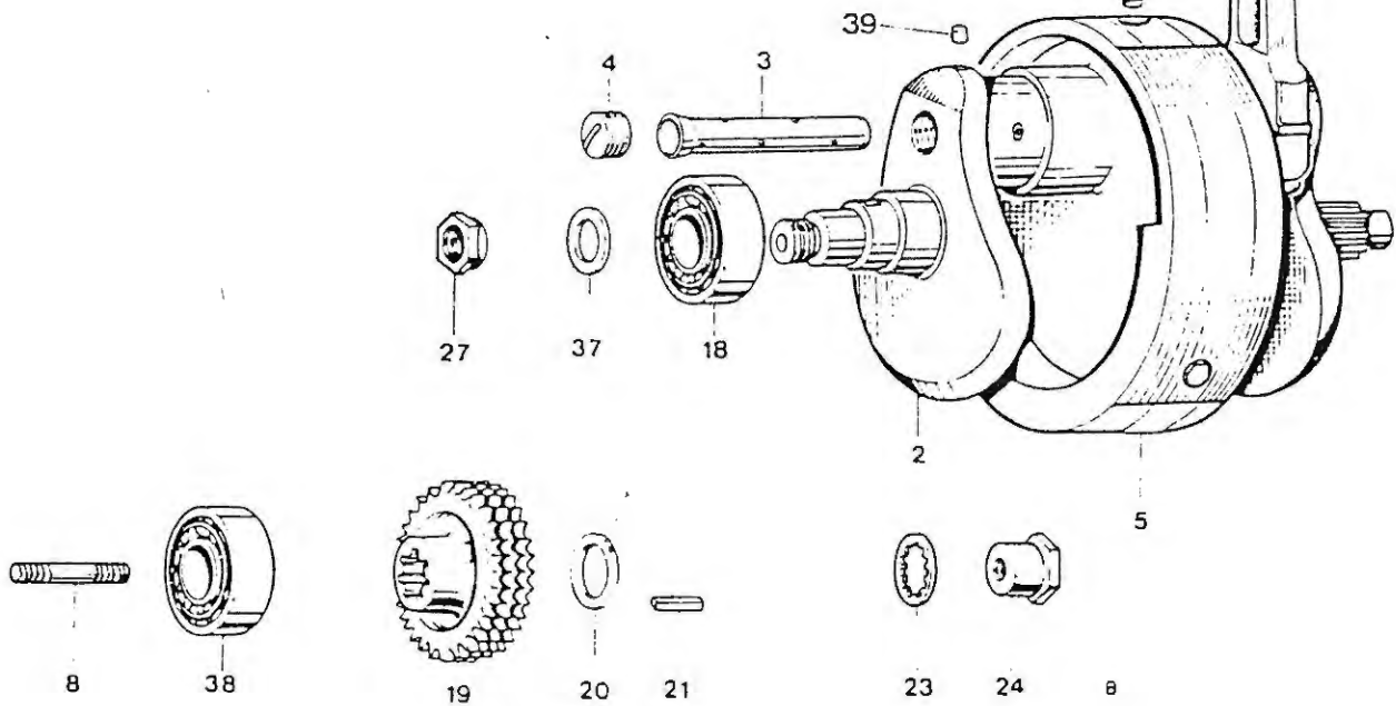
CRANKSHAFT AND CONNECTING RODS
