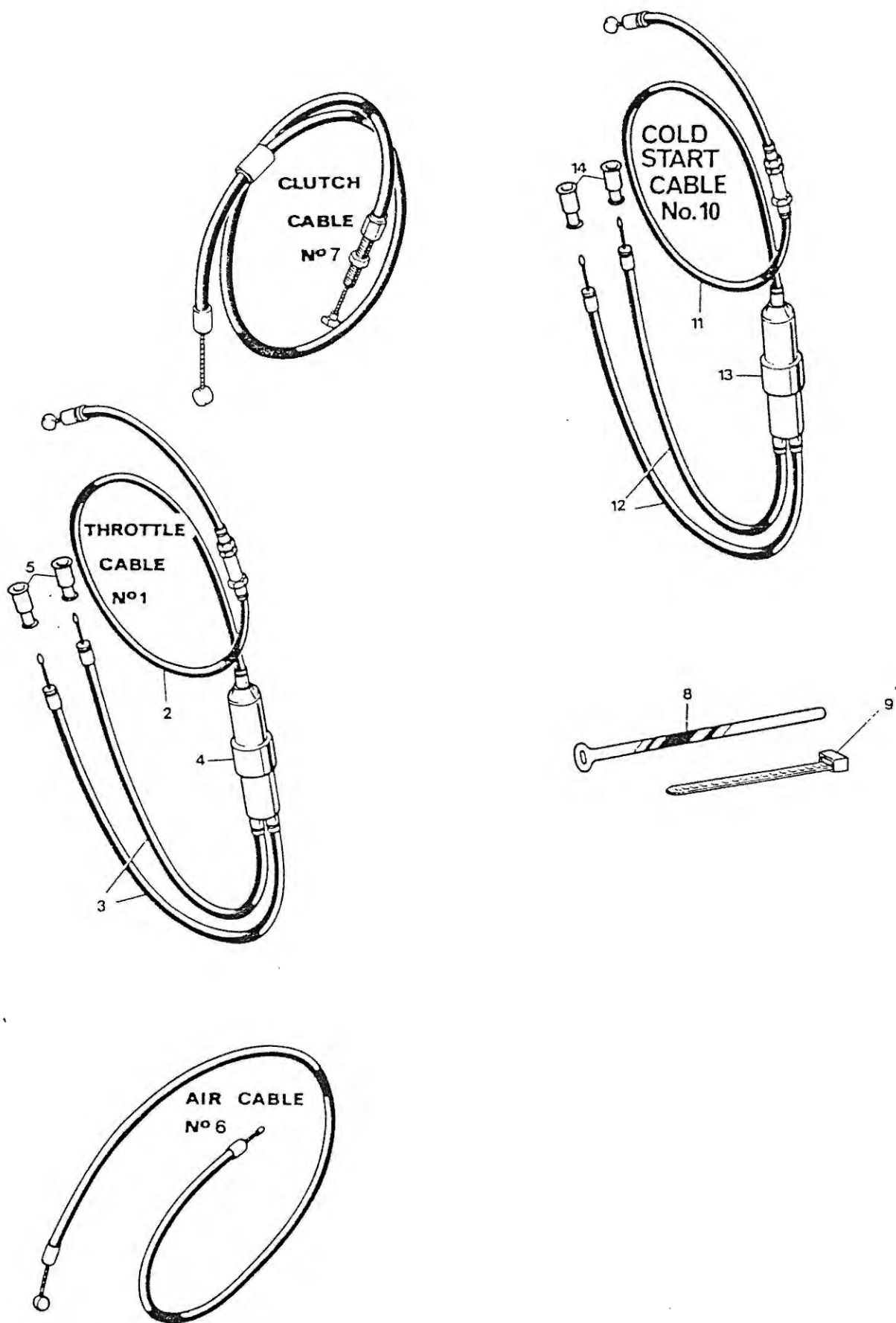
CONTROL CABLES
