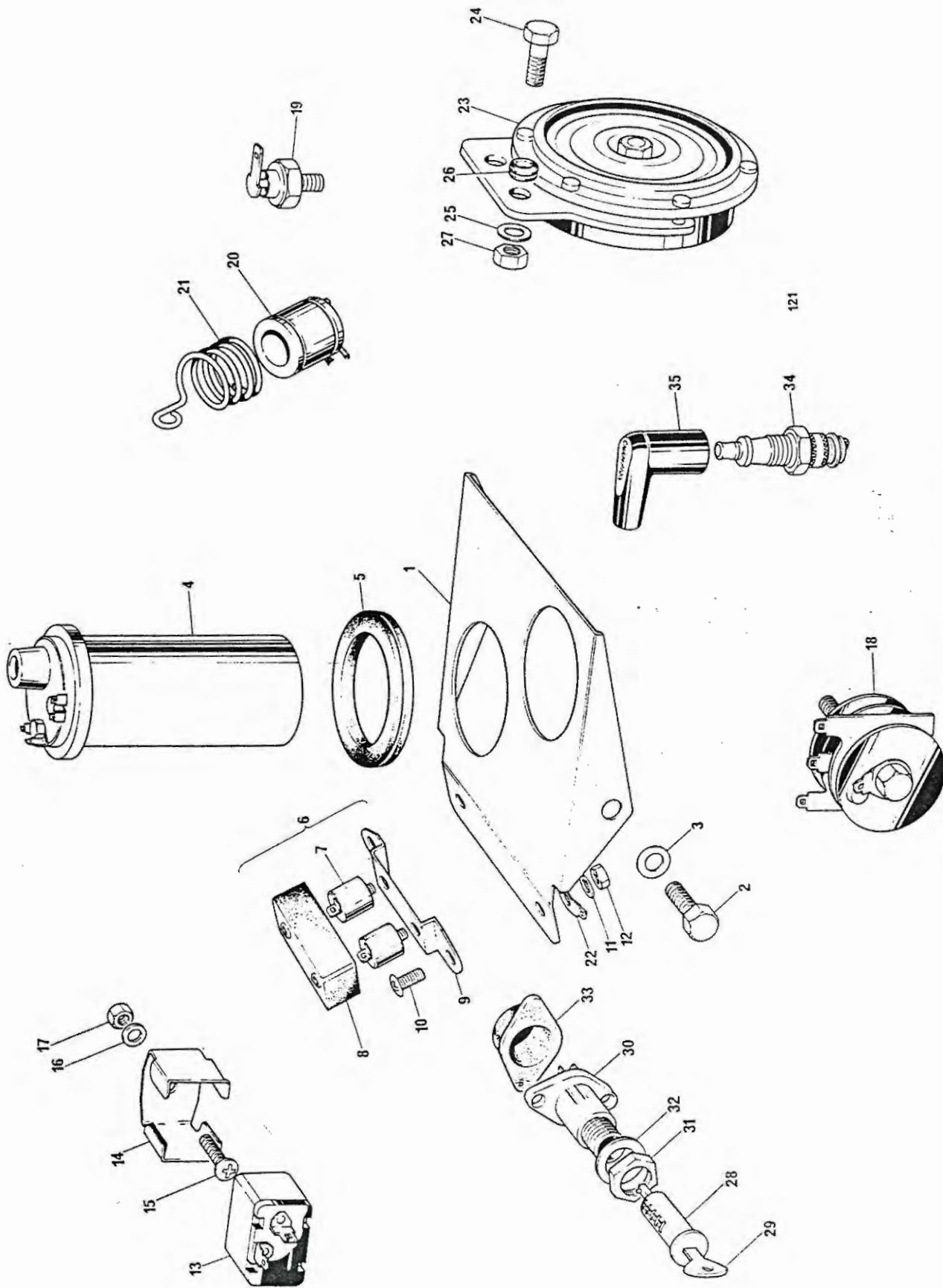
FIG. 23. ELECTRICAL COMPONENTS
