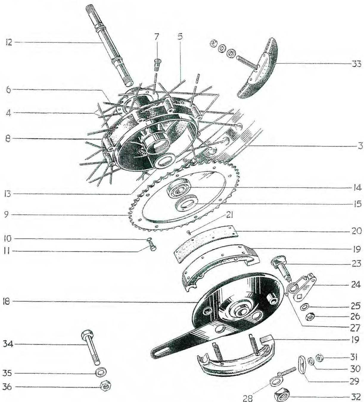
Fig. 13. REAR WHEEL
