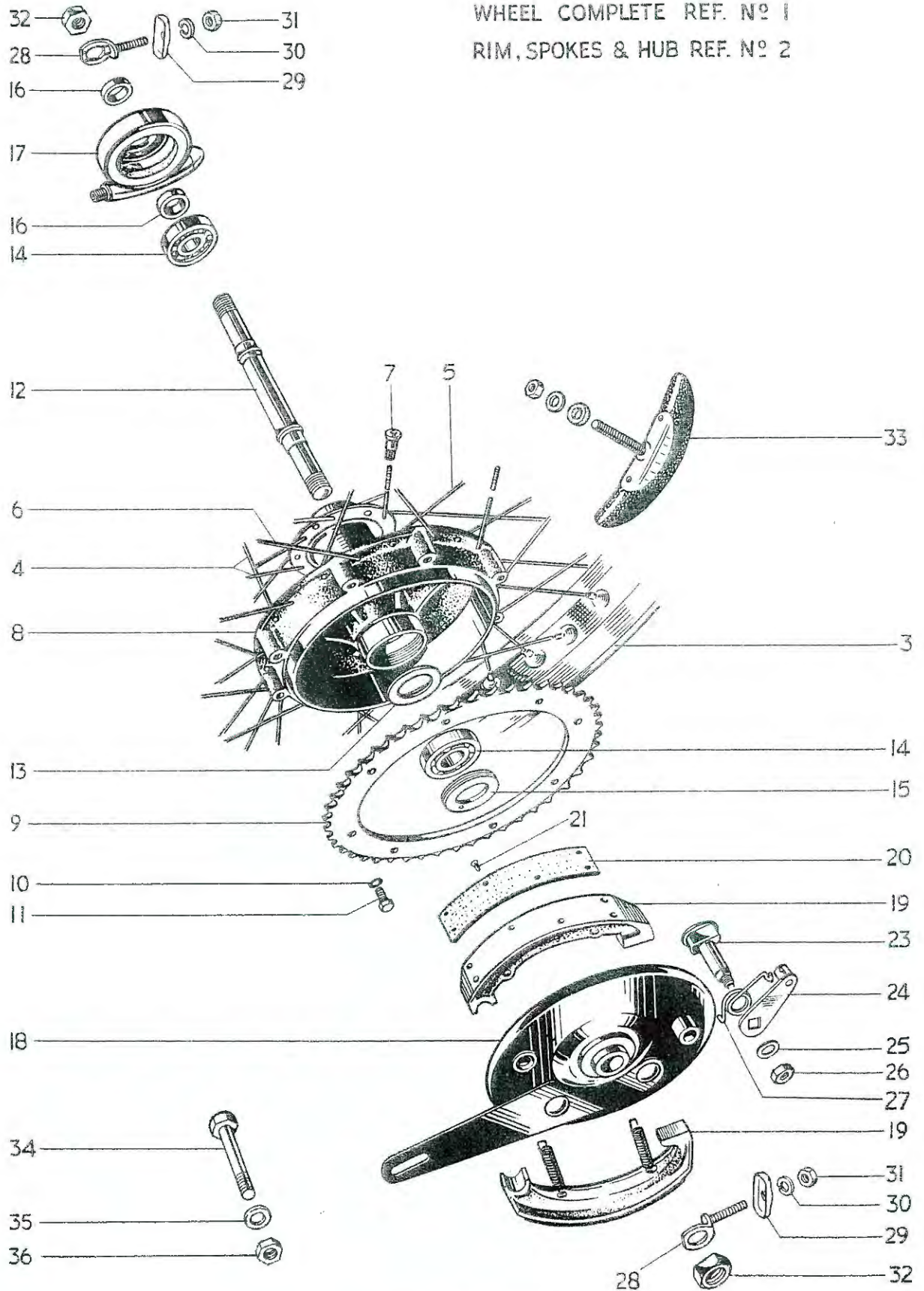
Fig. 13. REAR WHEEL
