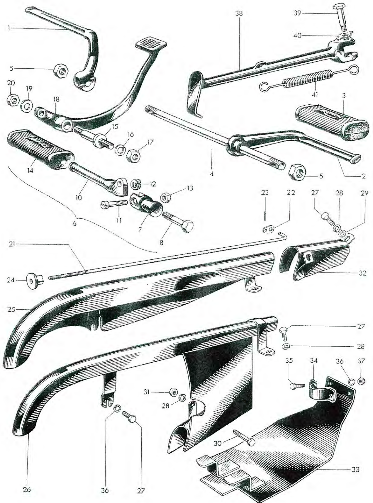
Fig. 8. FOOTRESTS, CHAINGUARD, PROPSTAND, ETC.
