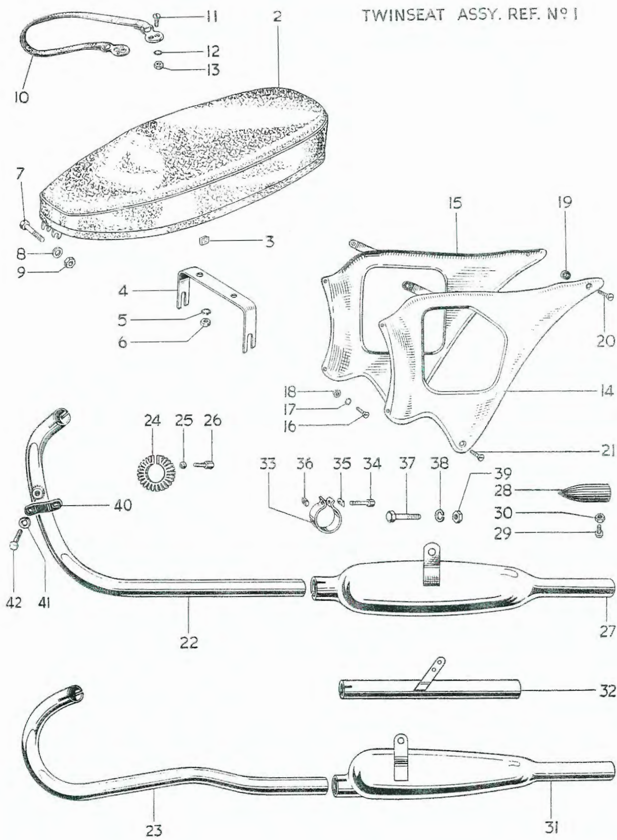
Fig. 15. TWINSEAT, REAR PANELS AND EXHAUST SYSTEM
