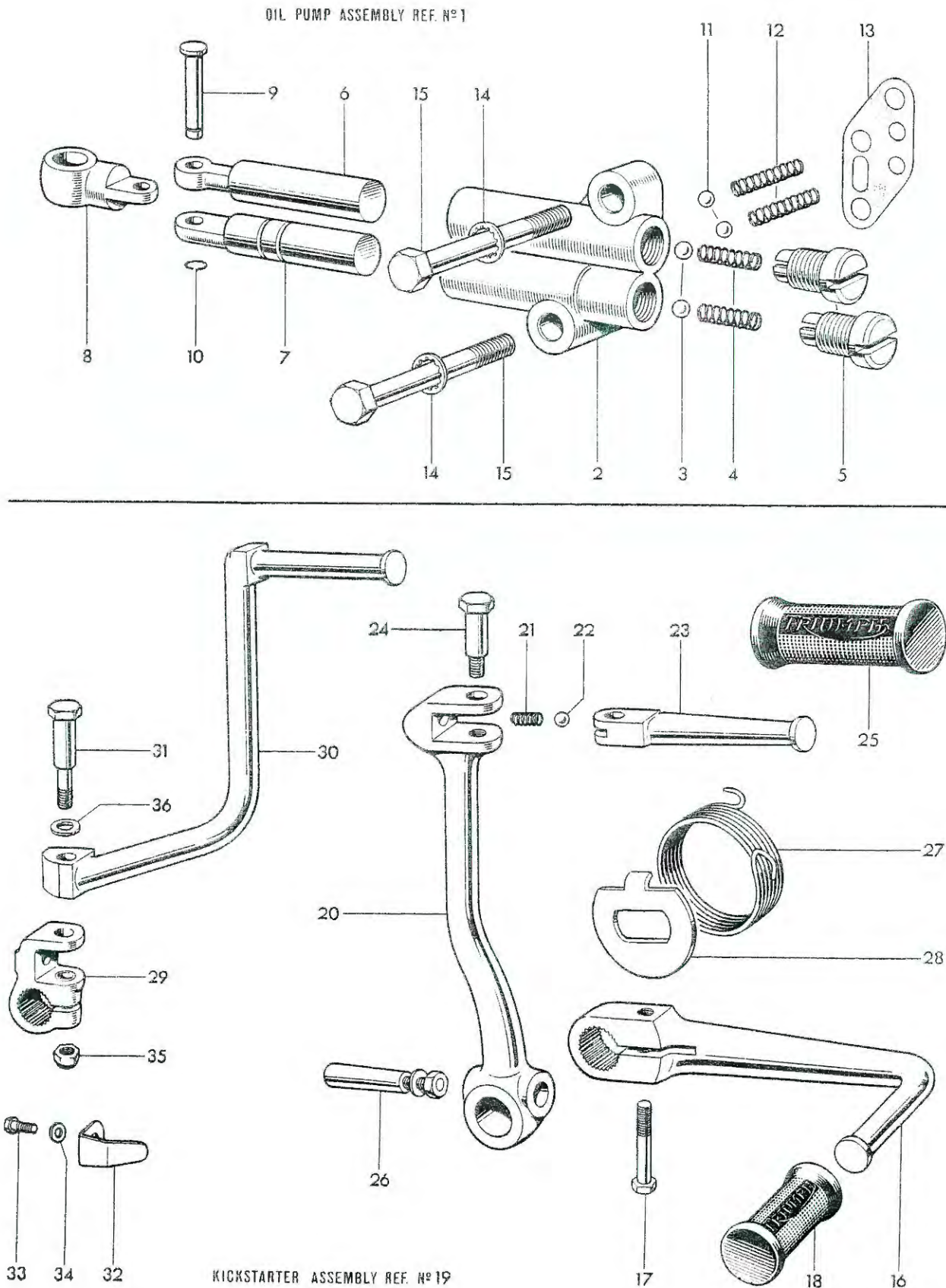
Fig. 4. OIL PUMP AND CONTROL PEDALS
