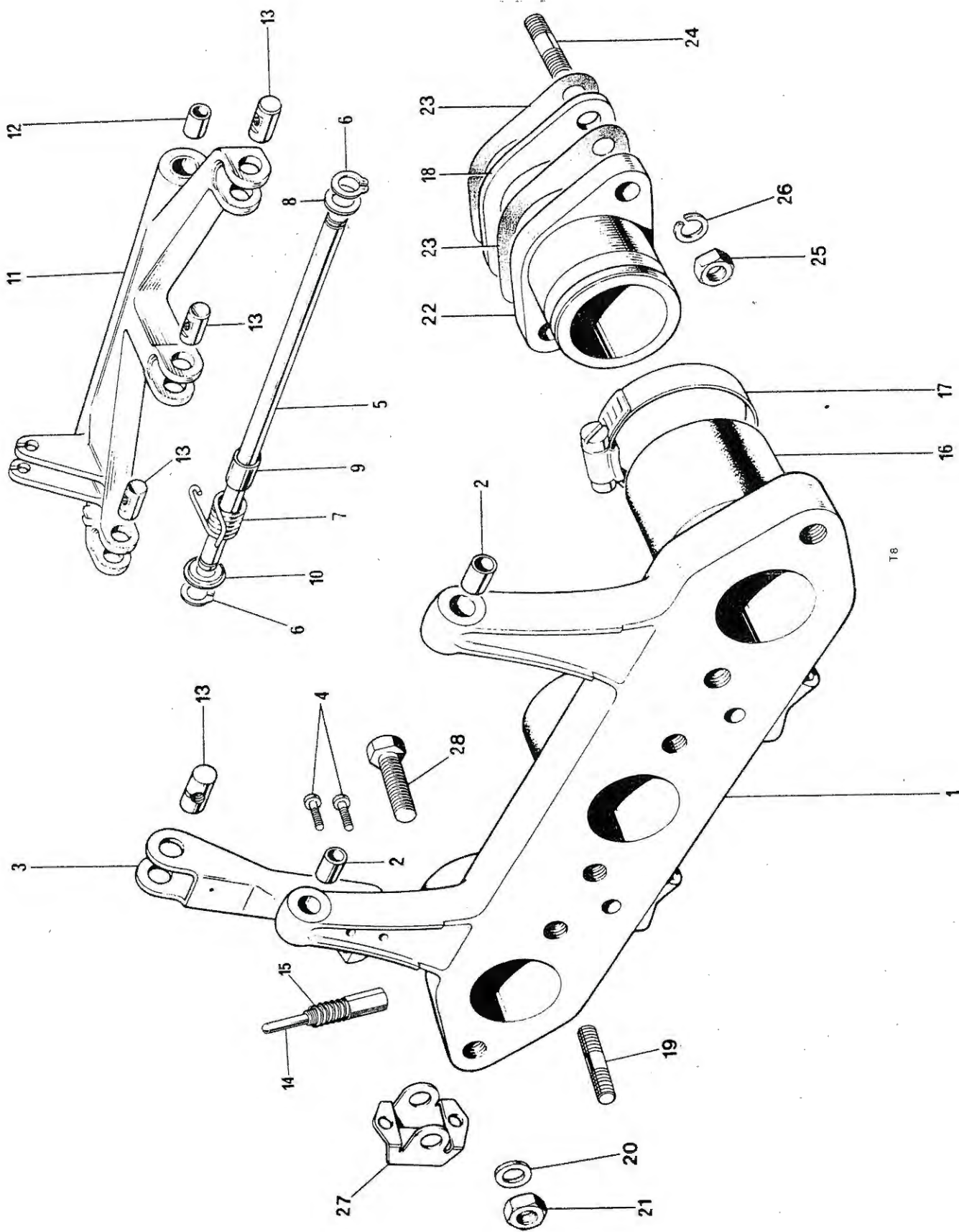
Fig. 8. MANIFOLD AND THROTTLE LINKAGE
