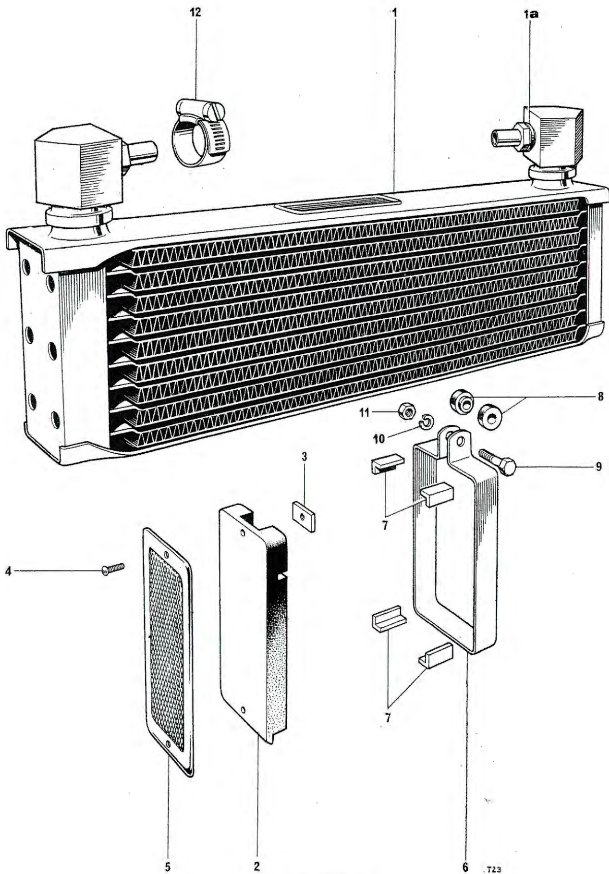
Fig. 23. OIL COOLER
