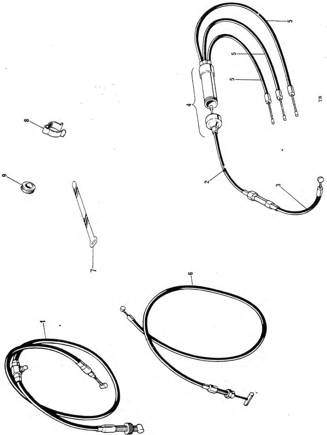
Fig.31. CONTROL CABLES
