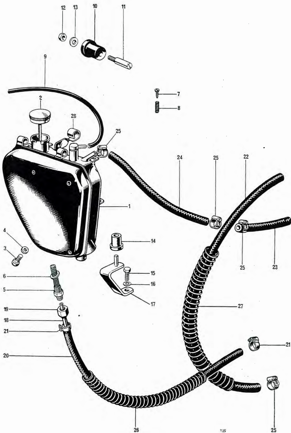
Fig. 25. OIL TANK
