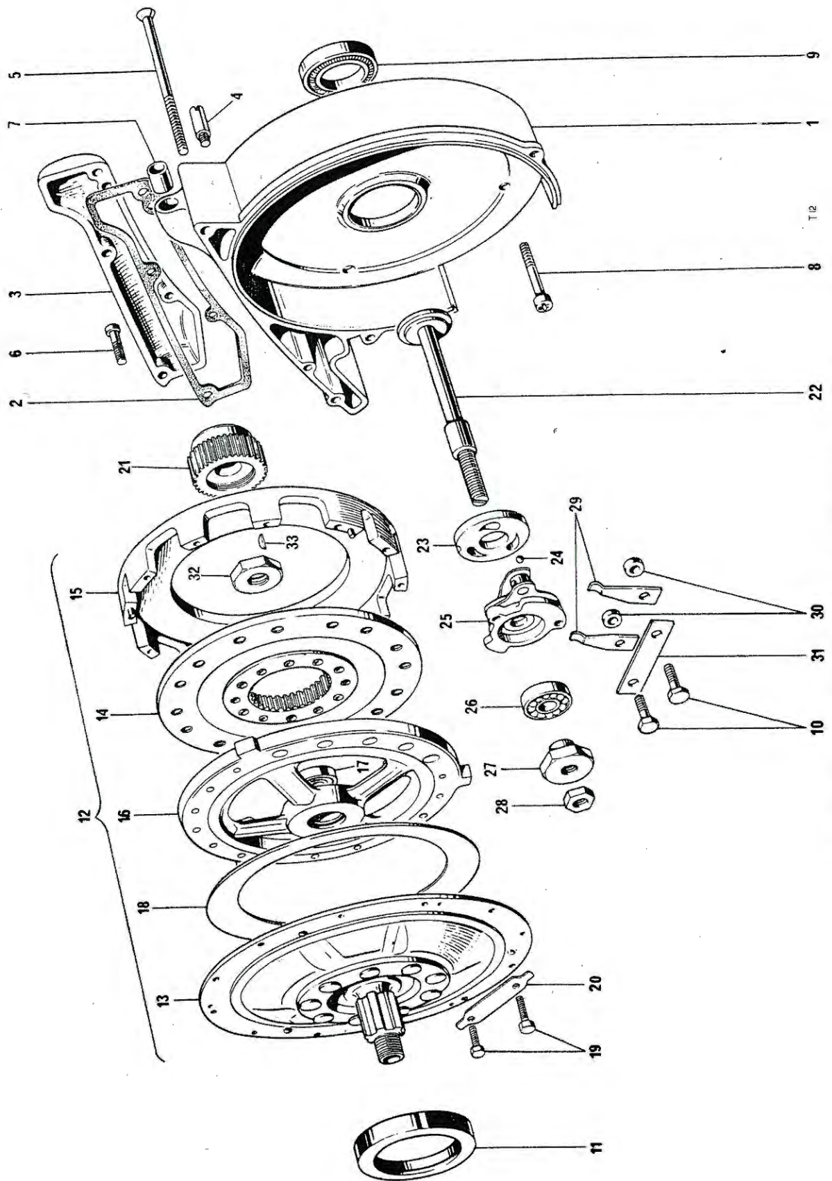
Fig. 12. CLUTCH AND CLUTCH OPERATING MECHANISM
