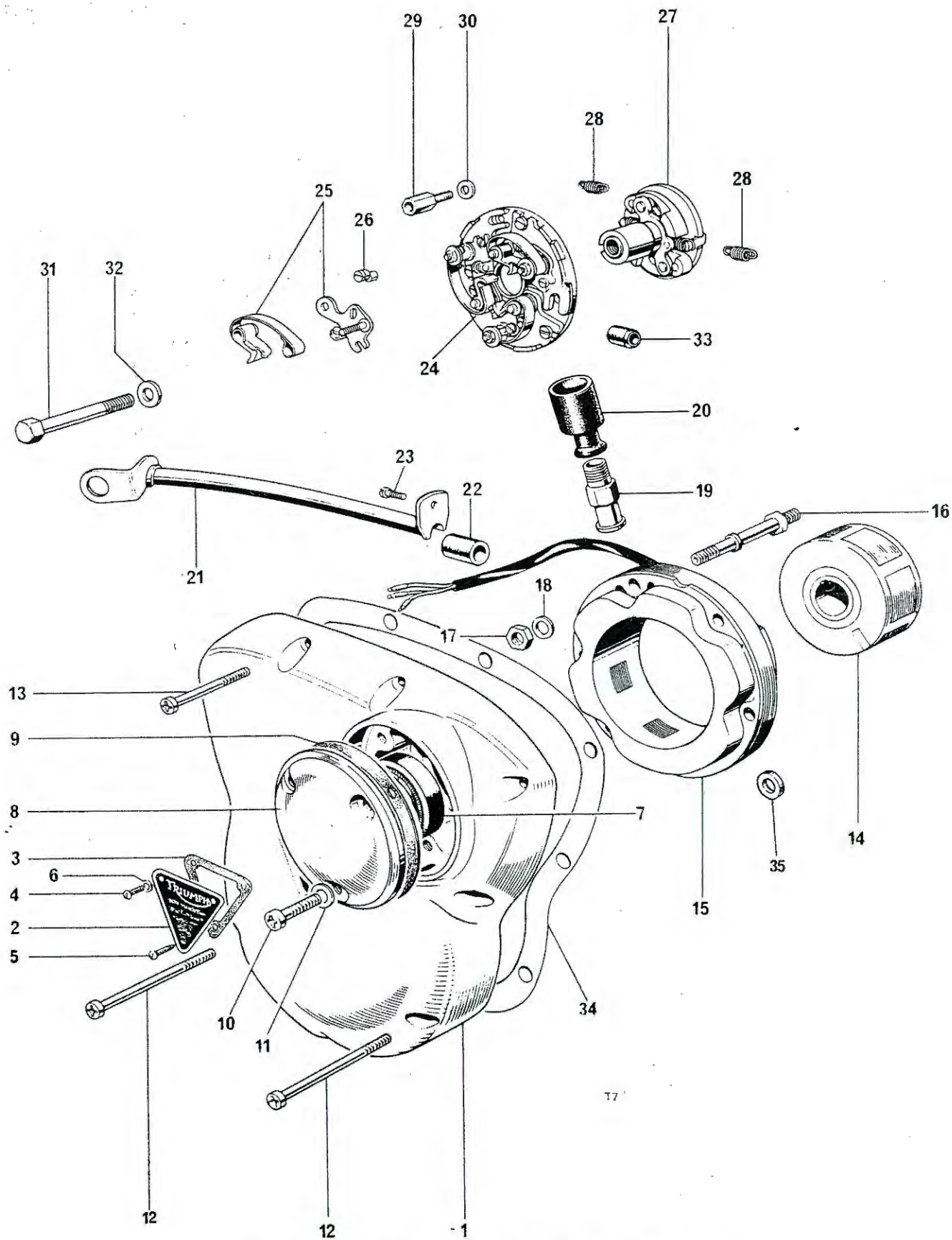
Fig. 7. TIMING COVER AND CONTACT BREAKER
